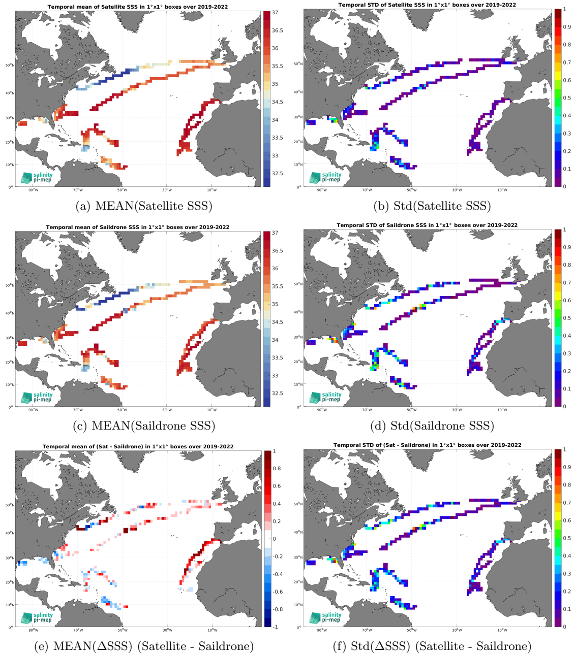
Figure 7: Temporal mean (left) and Std (right) of SSS from SMOS SSS L3 v9 - 18 Days (CATDS-CEC-LOCEAN) (top), Saildrone (middle), and of \Delta SSS (Satellite - Saildrone). Only match-up pairs are used to generate these maps.
