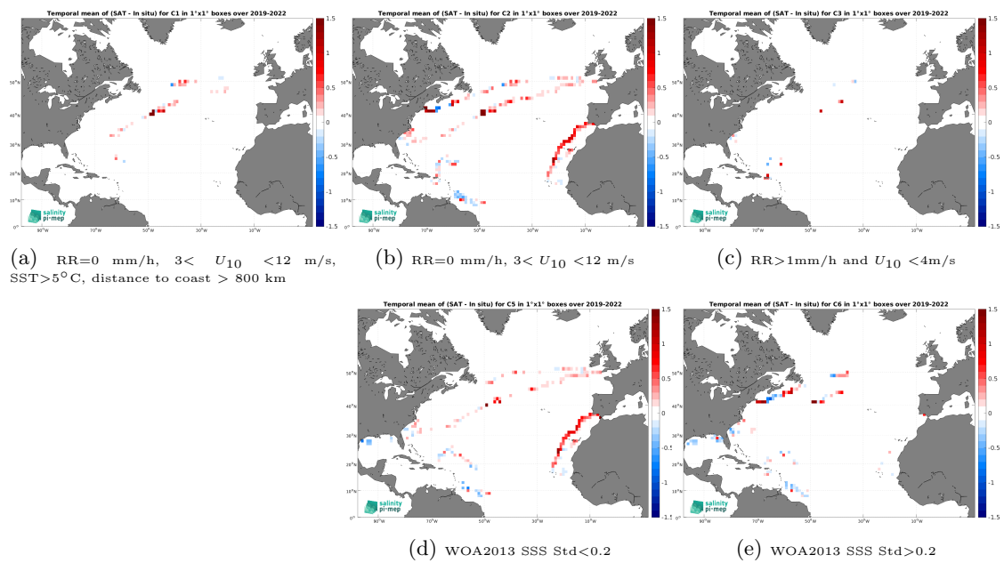
Figure 14: Temporal mean gridded over spatial boxes of size 1^\circ \times 1^\circ of \Delta\text{SSS} (SMOS SSS L3 v9 - 18 Days (CATDS-CEC-LOCEAN) - Saildrone) for 5 different subdatasets corresponding to:RR=0 mm/h, 3 < U_{10} < 12 m/s, SST >5^\circ\text{C} , distance to coast > 800 km (a), RR=0 mm/h, 3 < U_{10} < 12 m/s (b), RR >1 mm/h and U_{10} < 4 m/s (c), WOA2013 SSS Std <0.2 (d), WOA2013 SSS Std >0.2 (e).
