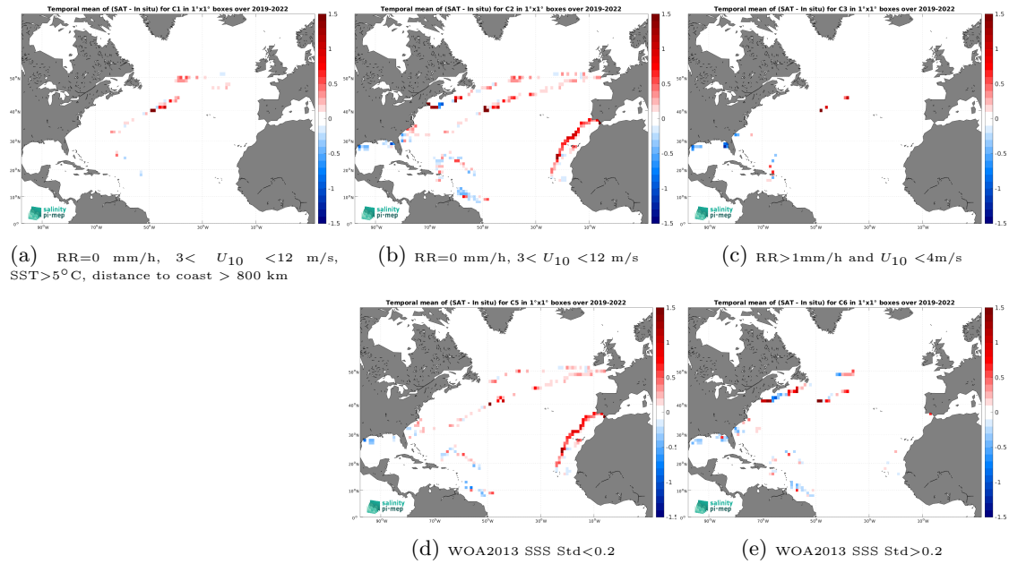
Figure 12: Temporal mean gridded over spatial boxes of size 1^\circ \times 1^\circ of \Delta\text{SSS} (SMOS SSS L3 v9 - 18 Days (CATDS-CEC-LOCEAN) - Saildrone) for 5 different subdatasets corresponding to:RR=0 mm/h, 3 < U_{10} < 12 m/s, SST >5^\circ\text{C} , distance to coast > 800 km (a), RR=0 mm/h, 3 < U_{10} < 12 m/s (b), RR >1 mm/h and U_{10} < 4 m/s (c), WOA2013 SSS Std <0.2 (d), WOA2013 SSS Std >0.2 (e).
