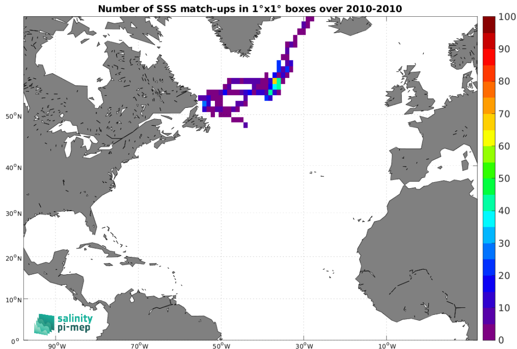
Figure 4: Number of SSS match-ups between Marine mammals SSS and the SMOS SSS L3 v9 - 18 Days (CATDS-CEC-LOCEAN) SSS product for the North Atlantic Ocean Pi-MEP region over 1^\circ \times 1^\circ boxes and for the full satellite product period.
