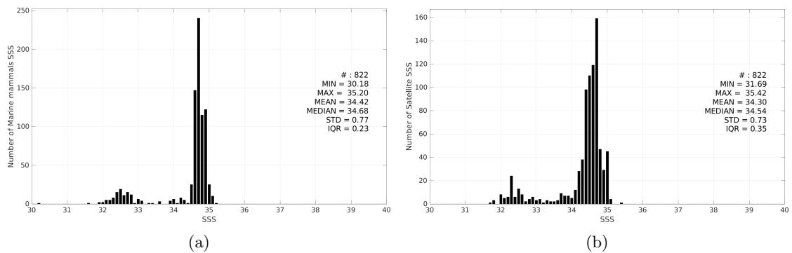
Figure 2: Histograms of SSS from Marine mammals (a) and SMOS SSS L3 v9 - 18 Days (CATDS-CEC-LOCEAN) (b) considering all match-up pairs per bins of 0.1 over the North Atlantic Ocean Pi-MEP region and for the full satellite product period.
