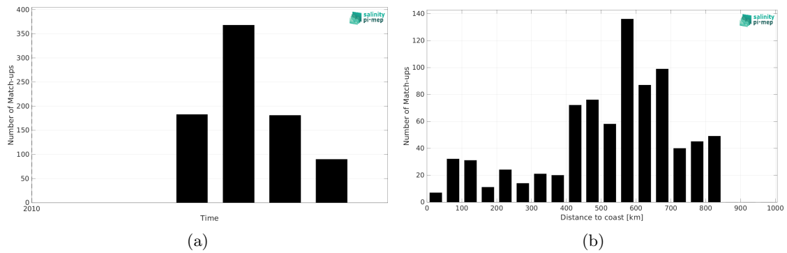
Figure 1: Number of match-ups between Marine mammals and SMOS SSS L3 v9 - 18 Days (CATDS-CEC-LOCEAN) SSS as a function of time (a) and as function of the distance to coast (b) over the North Atlantic Ocean Pi-MEP region and for the full satellite product period.
