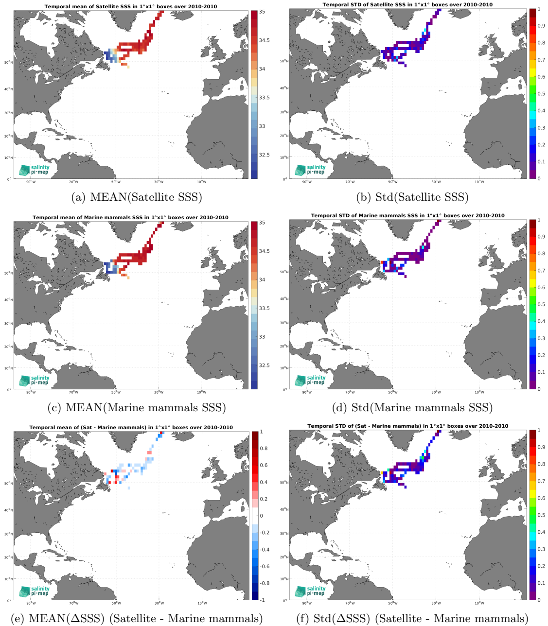
Figure 6: Temporal mean (left) and Std (right) of SSS from SMOS SSS L3 v9 - 18 Days (CATDS-CEC-LOCEAN) (top), Marine mammals (middle), and of \Delta SSS (Satellite - Marine mammals). Only match-up pairs are used to generate these maps.
