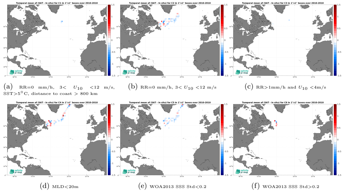
Figure 12: Temporal mean gridded over spatial boxes of size 1^{\circ}\times 1^{\circ} of \Delta\text{SSS} (SMOS SSS L3 v9 - 18 Days (CATDS-CEC-LOCEAN) - Marine mammals) for 6 different subdatasets corresponding to:RR=0 mm/h, 3 < U_{10} < 12 m/s, SST >5^{\circ}\text{C} , distance to coast > 800 km (a), RR=0 mm/h, 3 < U_{10} < 12 m/s (b), RR >1\text{mm/h} and U_{10} < 4\text{m/s} (c),MLD <20\text{m} (d),WOA2013 SSS Std <0.2 (e),WOA2013 SSS Std >0.2 (f).
