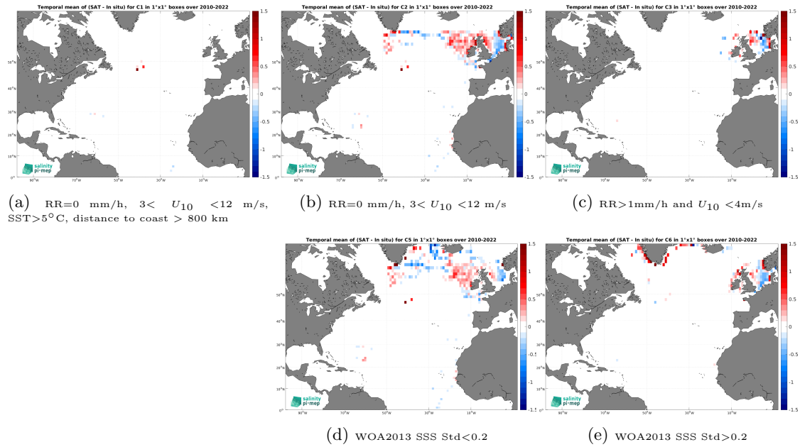
Figure 12: Temporal mean gridded over spatial boxes of size 1^\circ \times 1^\circ of \Delta\text{SSS} (SMOS SSS L3 v9 - 18 Days (CATDS-CEC-LOCEAN) - ICES) for 5 different subdatasets corresponding to:RR=0 mm/h, 3 < U_{10} < 12 m/s, SST >5^\circ\text{C} , distance to coast > 800 km (a), RR=0 mm/h, 3 < U_{10} < 12 m/s (b), RR >1 mm/h and U_{10} < 4 m/s (c), WOA2013 SSS Std <0.2 (d), WOA2013 SSS Std >0.2 (e).
