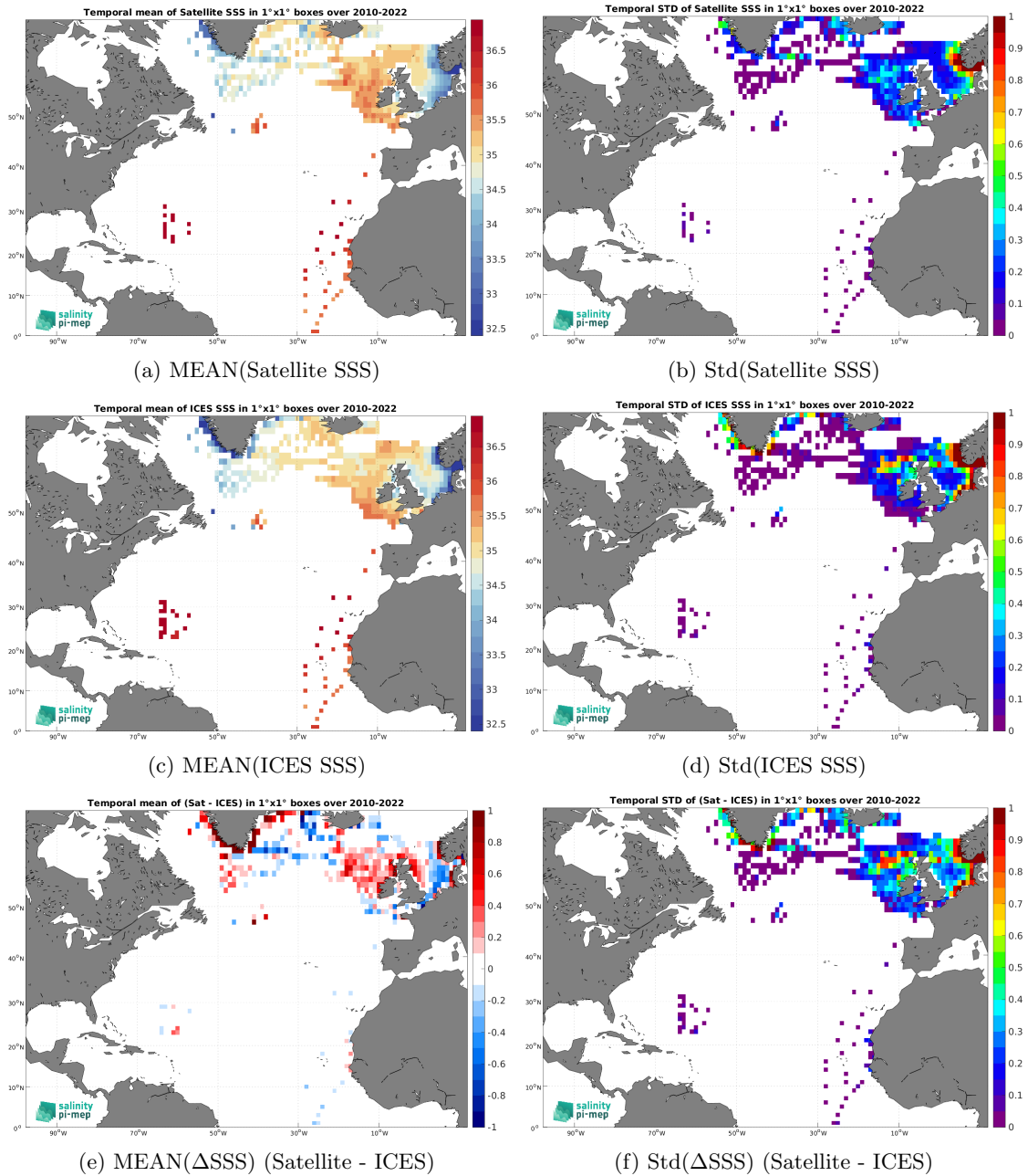
Figure 6: Temporal mean (left) and Std (right) of SSS from SMOS SSS L3 v9 - 18 Days (CATDS-CEC-LOCEAN) (top), ICES (middle), and of \Delta SSS (Satellite - ICES). Only match-up pairs are used to generate these maps.
