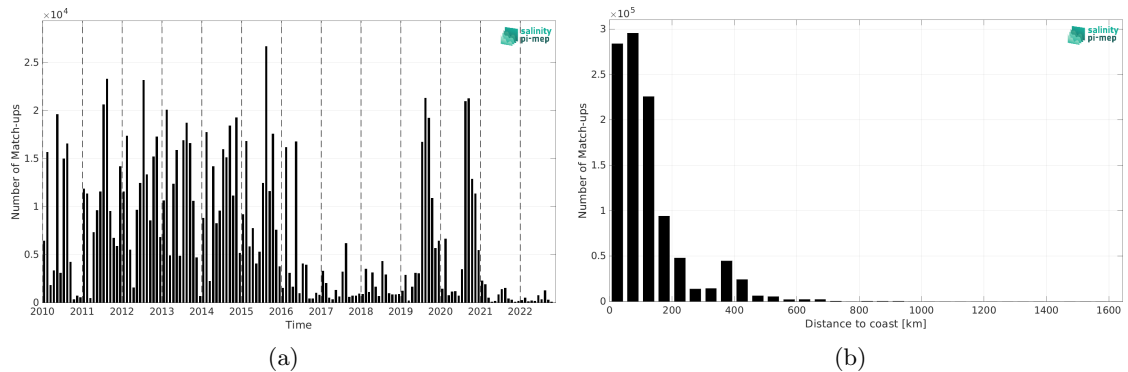
Figure 1: Number of match-ups between ICES and SMOS SSS L3 v9 - 18 Days (CATDS-CEC-LOCEAN) SSS as a function of time (a) and as function of the distance to coast (b) over the North Atlantic Ocean Pi-MEP region and for the full satellite product period.
