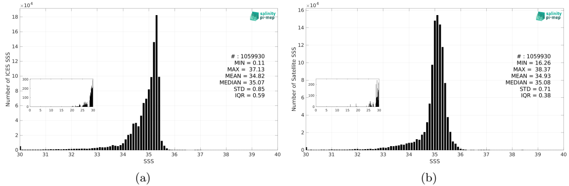
Figure 2: Histograms of SSS from ICES (a) and SMOS SSS L3 v9 - 18 Days (CATDS-CEC-LOCEAN) (b) considering all match-up pairs per bins of 0.1 over the North Atlantic Ocean Pi-MEP region and for the full satellite product period.
