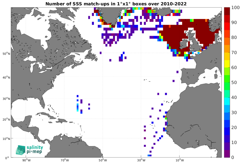
Figure 4: Number of SSS match-ups between ICES SSS and the SMOS SSS L3 v9 - 18 Days (CATDS-CEC-LOCEAN) SSS product for the North Atlantic Ocean Pi-MEP region over 1^\circ \times 1^\circ boxes and for the full satellite product period.
