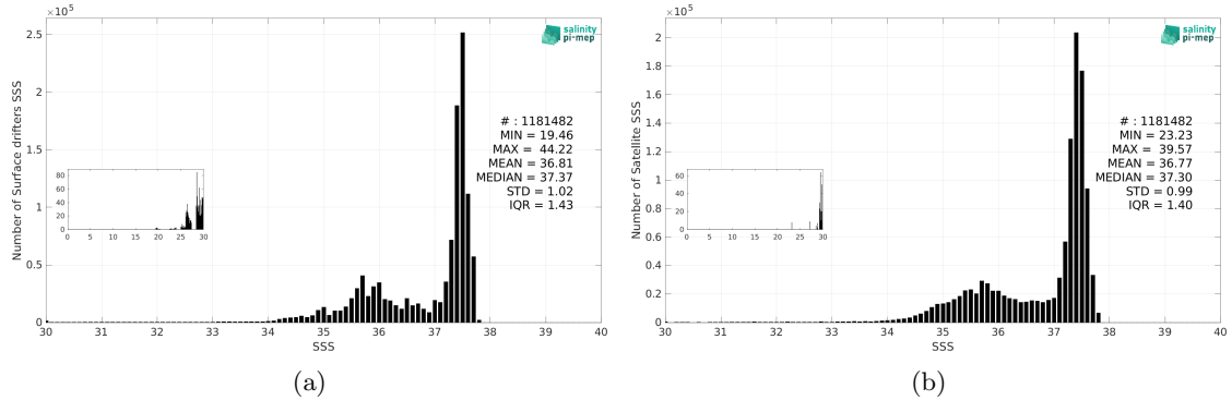
Figure 2: Histograms of SSS from Surface drifters (a) and SMOS SSS L3 v9 - 18 Days (CATDS-CEC-LOCEAN) (b) considering all match-up pairs per bins of 0.1 over the North Atlantic Ocean Pi-MEP region and for the full satellite product period.
