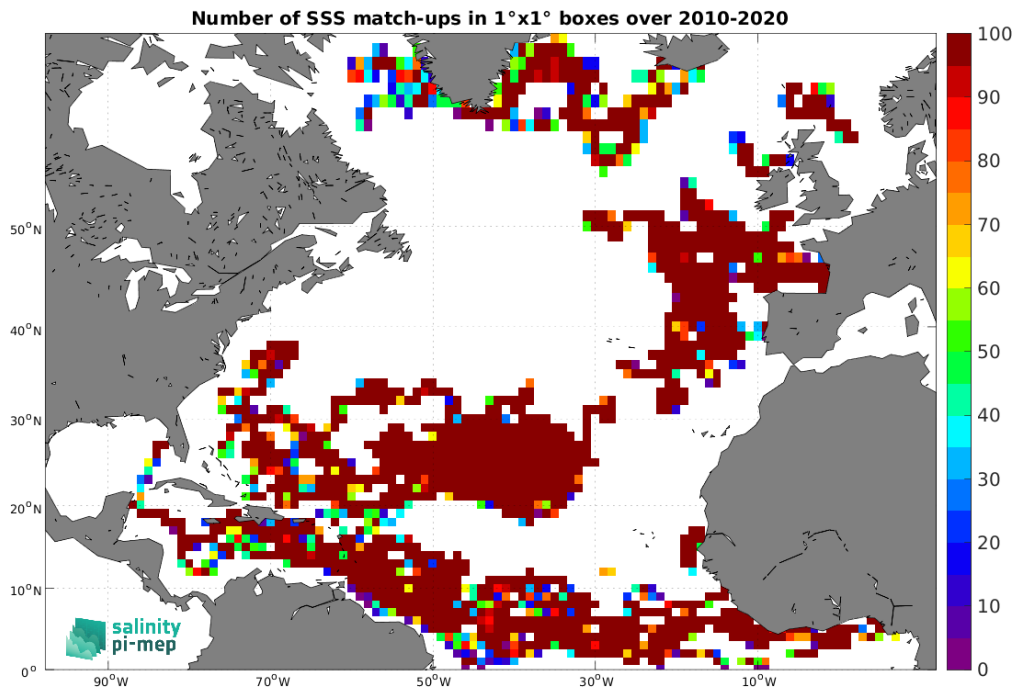
Figure 3: Number of SSS match-ups between Surface drifters SSS and the SMOS SSS L3 v9 - 18 Days (CATDS-CEC-LOCEAN) SSS product for the North Atlantic Ocean Pi-MEP region over 1^\circ \times 1^\circ boxes and for the full satellite product period.
