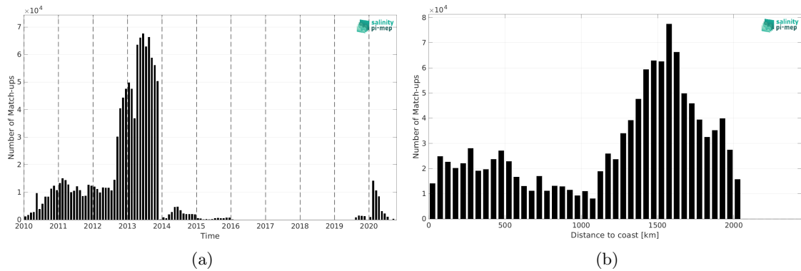
Figure 1: Number of match-ups between Surface drifters and SMOS SSS L3 v9 - 18 Days (CATDS-CEC-LOCEAN) SSS as a function of time (a) and as function of the distance to coast (b) over the North Atlantic Ocean Pi-MEP region and for the full satellite product period.
