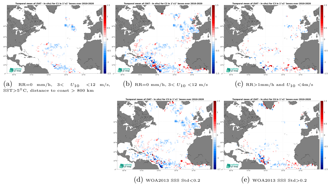
Figure 11: Temporal mean gridded over spatial boxes of size 1^\circ \times 1^\circ of \Delta\text{SSS} (SMOS SSS L3 v9 - 18 Days (CATDS-CEC-LOCEAN) - Surface drifters) for 5 different subdatasets corresponding to:RR=0 mm/h, 3 < U_{10} < 12 m/s, SST >5^\circ\text{C} , distance to coast > 800 km (a), RR=0 mm/h, 3 < U_{10} < 12 m/s (b), RR >1 mm/h and U_{10} < 4 m/s (c), WOA2013 SSS Std <0.2 (d), WOA2013 SSS Std >0.2 (e).
