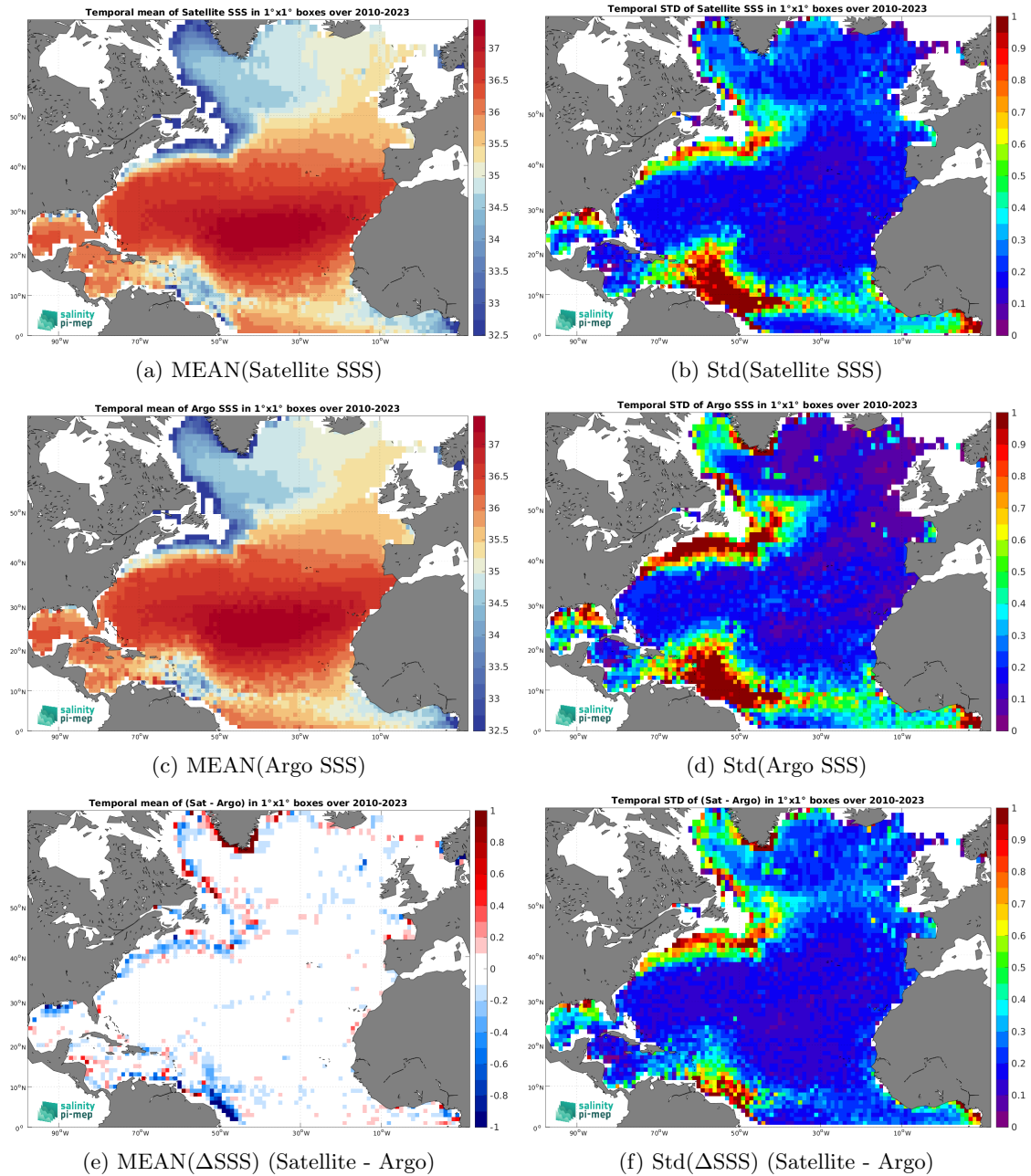
Figure 6: Temporal mean (left) and Std (right) of SSS from SMOS SSS L3 v9 - 18 Days (CATDS-CEC-LOCEAN) (top), Argo (middle), and of \Delta SSS (Satellite - Argo). Only match-up pairs are used to generate these maps.
