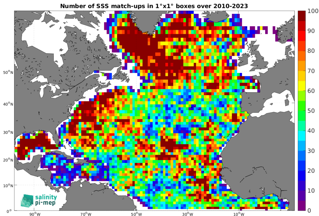
Figure 4: Number of SSS match-ups between Argo SSS and the SMOS SSS L3 v9 - 18 Days (CATDS-CEC-LOCEAN) SSS product for the North Atlantic Ocean Pi-MEP region over 1^\circ \times 1^\circ boxes and for the full satellite product period.
