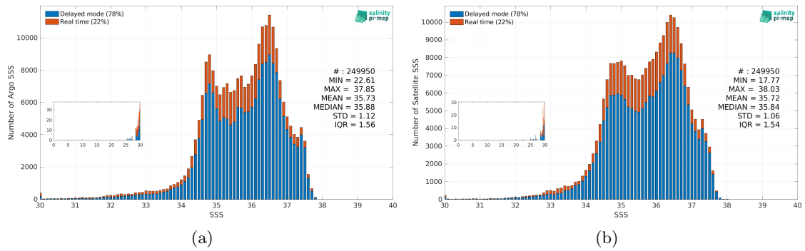
Figure 2: Histograms of SSS from Argo (a) and SMOS SSS L3 v9 - 18 Days (CATDS-CEC-LOCEAN) (b) considering all match-up pairs per bins of 0.1 over the North Atlantic Ocean Pi-MEP region and for the full satellite product period.
