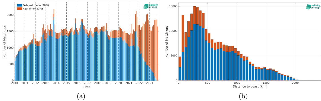
Figure 1: Number of match-ups between Argo and SMOS SSS L3 v9 - 18 Days (CATDS-CEC-LOCEAN) SSS as a function of time (a) and as function of the distance to coast (b) over the North Atlantic Ocean Pi-MEP region and for the full satellite product period.
