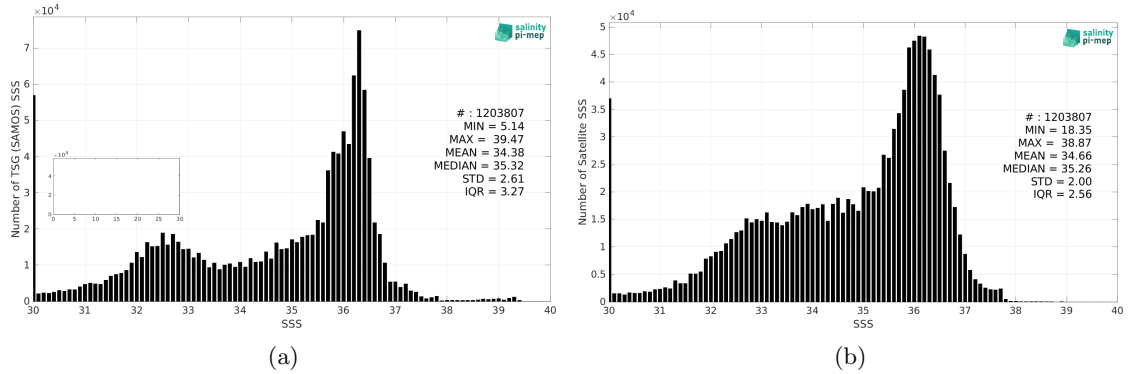
Figure 2: Histograms of SSS from TSG (SAMOS) (a) and SMOS SSS L3 v8 - 9 Days (CATDS-CEC-LOCEAN) (b) considering all match-up pairs per bins of 0.1 over the North Atlantic Ocean Pi-MEP region and for the full satellite product period.
