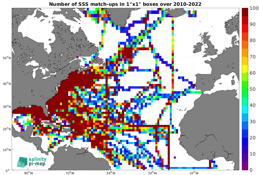
Figure 4: Number of SSS match-ups between TSG (SAMOS) SSS and the SMOS SSS L3 v8 - 9 Days (CATDS-CEC-LOCEAN) SSS product for the North Atlantic Ocean Pi-MEP region over 1^\circ \times 1^\circ boxes and for the full satellite product period.
