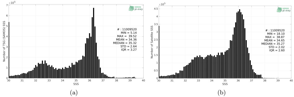
Figure 2: Histograms of SSS from TSG (SAMOS) (a) and SMOS SSS L3 v8 - 9 Days (CATDS-CECOS-LOCEAN) (b) considering all match-up pairs per bins of 0.1 over the North Atlantic Ocean Pi-MEP region and for the full satellite product period.
