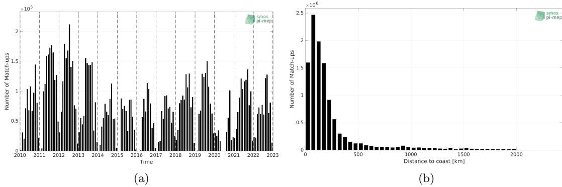
Figure 1: Number of match-ups between TSG (SAMOS) and SMOS SSS L3 v8 - 9 Days (CATDS-CECOS-LOCEAN) SSS as a function of time (a) and as function of the distance to coast (b) over the North Atlantic Ocean Pi-MEP region and for the full satellite product period.
