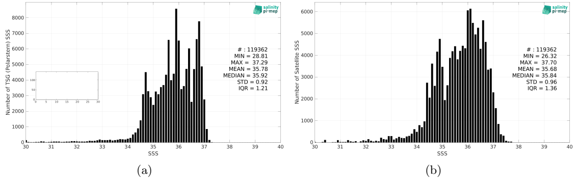
Figure 2: Histograms of SSS from TSG (Polarstern) (a) and SMOS SSS L3 v8 - 9 Days (CATDS-CEC-LOCEAN) (b) considering all match-up pairs per bins of 0.1 over the North Atlantic Ocean Pi-MEP region and for the full satellite product period.
