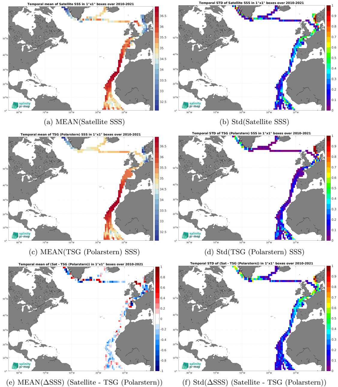
Figure 6: Temporal mean (left) and Std (right) of SSS from SMOS SSS L3 v8 - 9 Days (CATDS-CEC-LOCEAN) (top), TSG (Polarstern) (middle), and of \Delta SSS (Satellite - TSG (Polarstern)). Only match-up pairs are used to generate these maps.
