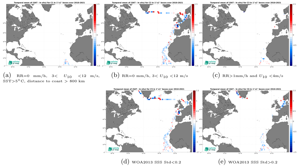
Figure 12: Temporal mean gridded over spatial boxes of size 1^\circ \times 1^\circ of \Delta\text{SSS} (SMOS SSS L3 v8 - 9 Days (CATDS-CEC-LOCEAN) - TSG (Polarstern)) for 5 different subdatasets corresponding to:RR=0 mm/h, 3 < U_{10} < 12 m/s, SST >5^\circ\text{C} , distance to coast > 800 km (a), RR=0 mm/h, 3 < U_{10} < 12 m/s (b), RR >1 mm/h and U_{10} < 4 m/s (c), WOA2013 SSS Std <0.2 (d), WOA2013 SSS Std >0.2 (e).
