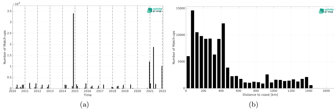
Figure 1: Number of match-ups between TSG (Polarstern) and SMOS SSS L3 v8 - 9 Days (CATDS-CEC-LOCEAN) SSS as a function of time (a) and as function of the distance to coast (b) over the North Atlantic Ocean Pi-MEP region and for the full satellite product period.
