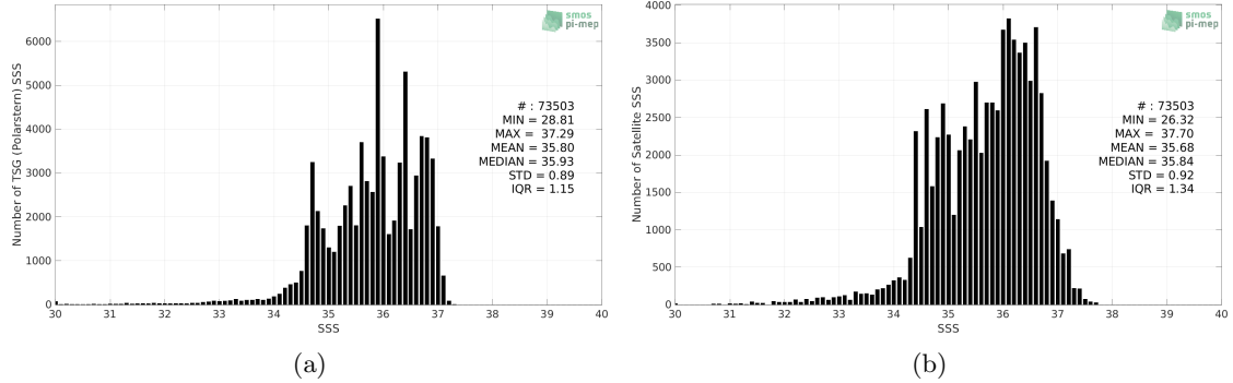
Figure 2: Histograms of SSS from TSG (Polarstern) (a) and SMOS SSS L3 v8 - 9 Days (CATDS-CECOS-LOCEAN) (b) considering all match-up pairs per bins of 0.1 over the North Atlantic Ocean Pi-MEP region and for the full satellite product period.
