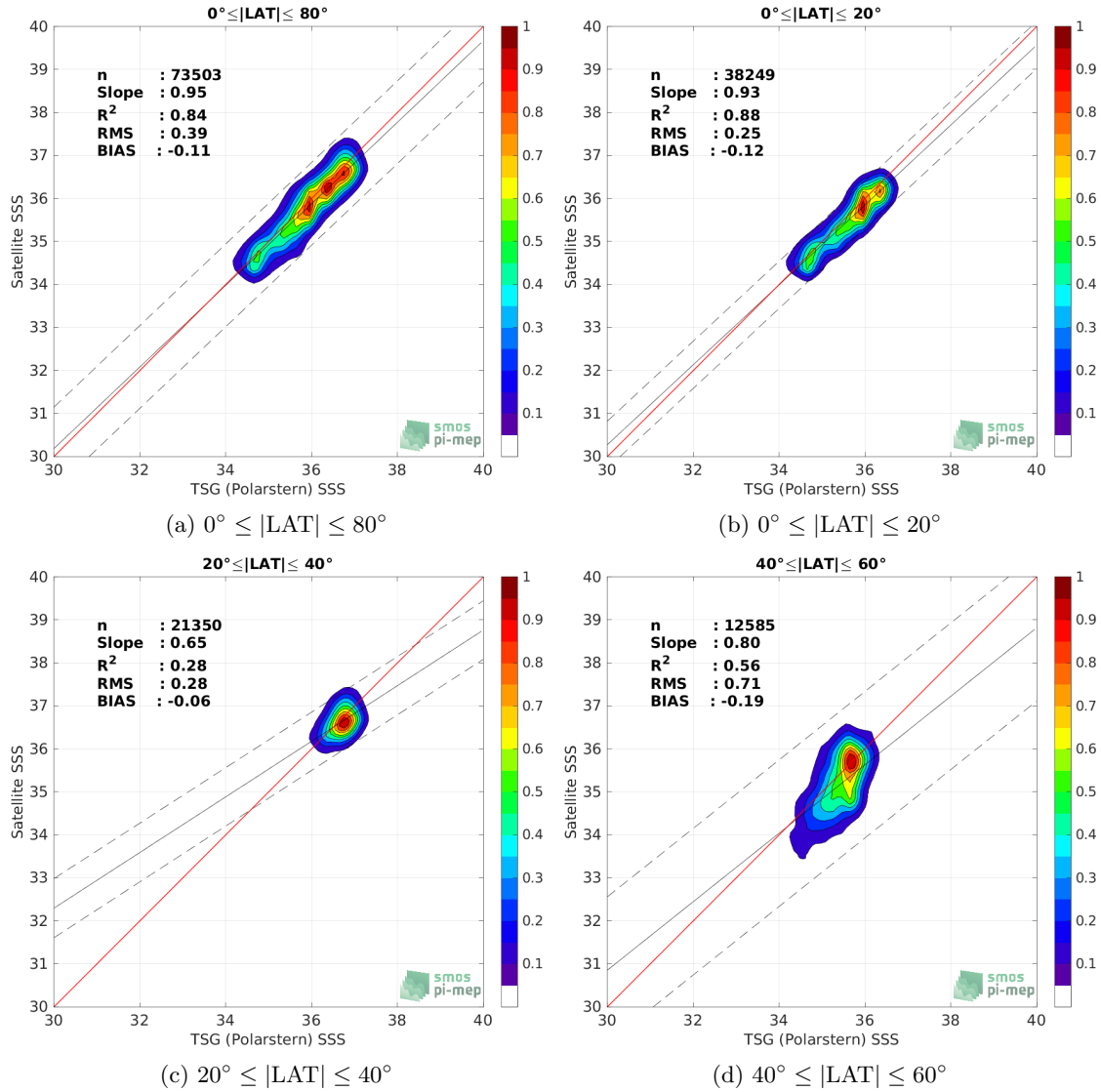
Figure 9: Contour maps of the concentration of SMOS SSS L3 v8 - 9 Days (CATDS-CECOS-LOCEAN) SSS (y-axis) versus TSG (Polarstern) SSS (x-axis) at match-up pairs for different latitude bands. For each plot, the red line shows x=y . The black thin and dashed lines indicate a linear fit through the data cloud and the \pm 95\% confidence levels, respectively. The number match-up pairs n , the slope and R^2 coefficient of the linear fit, the root mean square (RMS) and the mean bias between satellite and in situ data are indicated for each latitude band in each plots.
