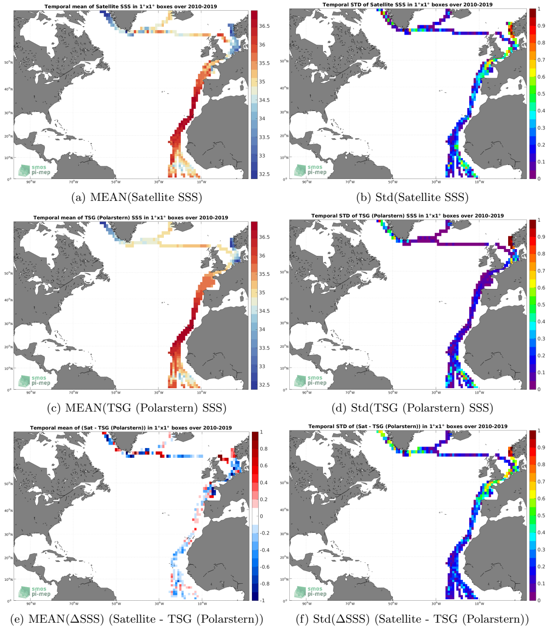
Figure 6: Temporal mean (left) and Std (right) of SSS from SMOS SSS L3 v8 - 9 Days (CATDS-CECOS-LOCEAN) (top), TSG (Polarstern) (middle), and of \Delta SSS (Satellite - TSG (Polarstern)). Only match-up pairs are used to generate these maps.
