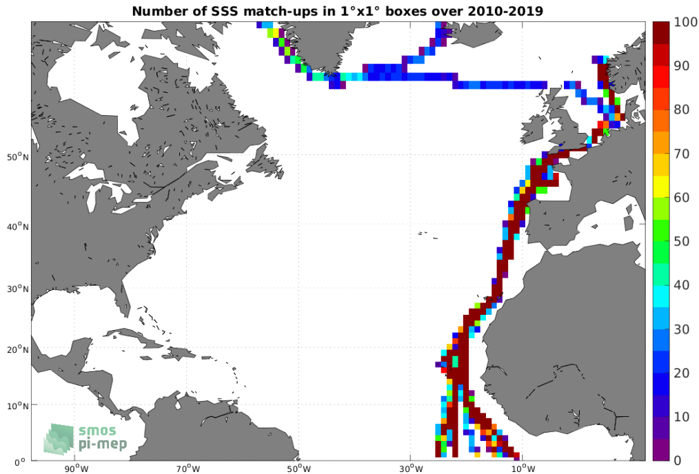
Figure 4: Number of SSS match-ups between TSG (Polarstern) SSS and the SMOS SSS L3 v8 - 9 Days (CATDS-CECOS-LOCEAN) SSS product for the North Atlantic Ocean Pi-MEP region over 1^\circ \times 1^\circ boxes and for the full satellite product period.
