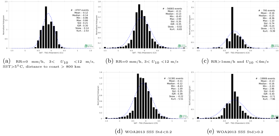
Figure 13: Normalized histogram of \Delta SSS (SMOS SSS L3 v8 - 9 Days (CATDS-CECOS-LOCEAN) - TSG (Polarstern)) for 5 different subdatasets corresponding to: RR=0 mm/h, 3 < U_{10} < 12 m/s, SST>5°C, distance to coast > 800 km (a), RR=0 mm/h, 3 < U_{10} < 12 m/s (b), RR>1mm/h and U_{10} < 4 m/s (c), WOA2013 SSS Std<0.2 (d), WOA2013 SSS Std>0.2 (e).
