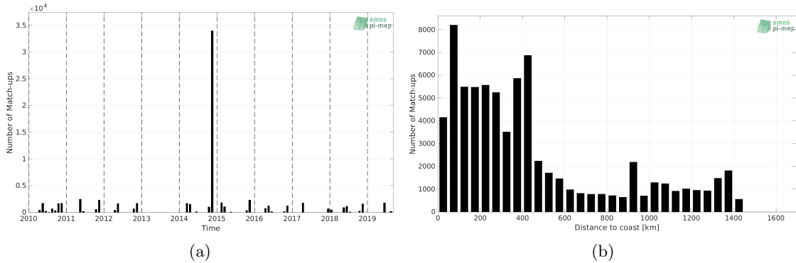
Figure 1: Number of match-ups between TSG (Polarstern) and SMOS SSS L3 v8 - 9 Days (CATDS-CECOS-LOCEAN) SSS as a function of time (a) and as function of the distance to coast (b) over the North Atlantic Ocean Pi-MEP region and for the full satellite product period.
