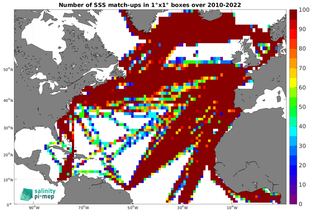
Figure 4: Number of SSS match-ups between TSG (LEGOS-DM) SSS and the SMOS SSS L3 v8 - 9 Days (CATDS-CEC-LOCEAN) SSS product for the North Atlantic Ocean Pi-MEP region over 1^\circ \times 1^\circ boxes and for the full satellite product period.
