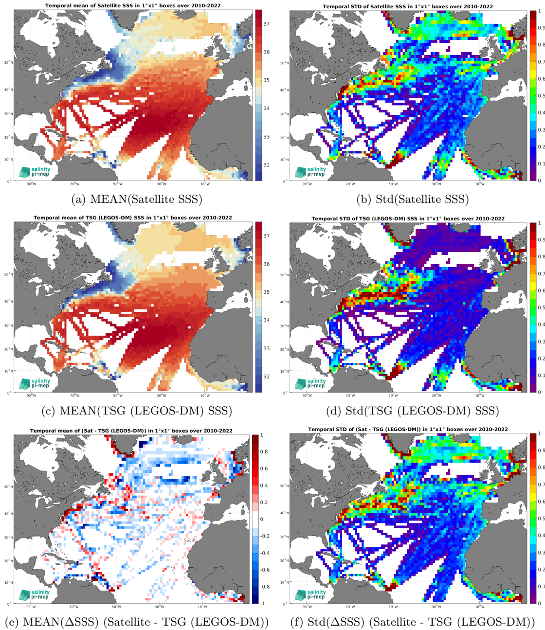
Figure 6: Temporal mean (left) and Std (right) of SSS from SMOS SSS L3 v8 - 9 Days (CATDS-CEC-LOCEAN) (top), TSG (LEGOS-DM) (middle), and of \Delta SSS (Satellite - TSG (LEGOS-DM)). Only match-up pairs are used to generate these maps.
