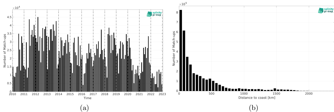
Figure 1: Number of match-ups between TSG (LEGOS-DM) and SMOS SSS L3 v8 - 9 Days (CATDS-CEC-LOCEAN) SSS as a function of time (a) and as function of the distance to coast (b) over the North Atlantic Ocean Pi-MEP region and for the full satellite product period.
