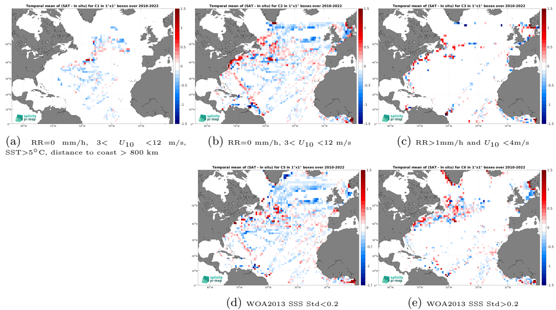
Figure 12: Temporal mean gridded over spatial boxes of size 1^\circ \times 1^\circ of \Delta\text{SSS} (SMOS SSS L3 v8 - 9 Days (CATDS-CEC-LOCEAN) - TSG (LEGOS-DM)) for 5 different subdatasets corresponding to:RR=0 mm/h, 3 < U_{10} < 12 m/s, SST > 5^\circ\text{C} , distance to coast > 800 km (a), RR=0 mm/h, 3 < U_{10} < 12 m/s (b), RR > 1 mm/h and U_{10} < 4 m/s (c), WOA2013 SSS Std < 0.2 (d), WOA2013 SSS Std > 0.2 (e).
