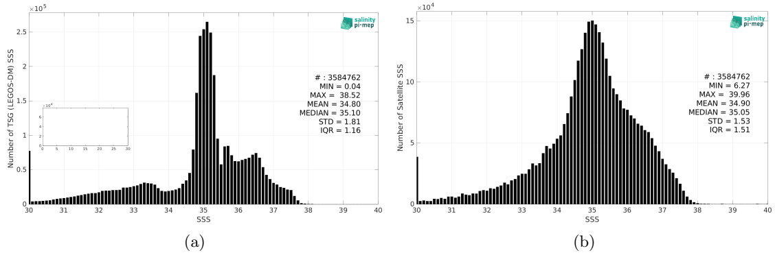
Figure 2: Histograms of SSS from TSG (LEGOS-DM) (a) and SMOS SSS L3 v8 - 9 Days (CATDS-CEC-LOCEAN) (b) considering all match-up pairs per bins of 0.1 over the North Atlantic Ocean Pi-MEP region and for the full satellite product period.
