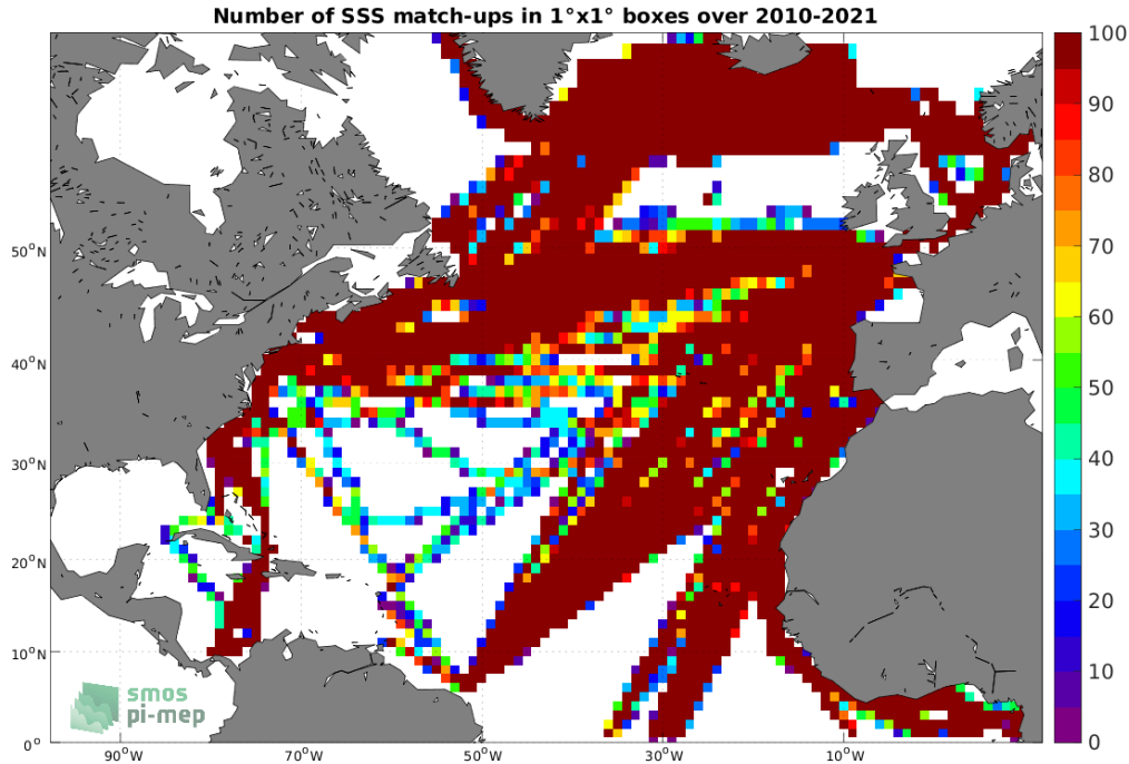
Figure 4: Number of SSS match-ups between TSG (LEGOS-DM) SSS and the SMOS SSS L3 v8 - 9 Days (CATDS-CECOS-LOCEAN) SSS product for the North Atlantic Ocean Pi-MEP region over 1^\circ \times 1^\circ boxes and for the full satellite product period.
