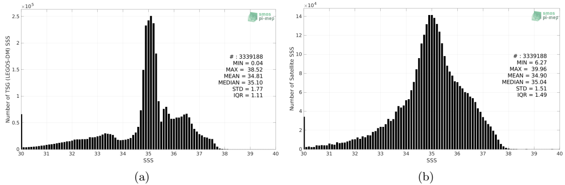
Figure 2: Histograms of SSS from TSG (LEGOS-DM) (a) and SMOS SSS L3 v8 - 9 Days (CATDS-CECOS-LOCEAN) (b) considering all match-up pairs per bins of 0.1 over the North Atlantic Ocean Pi-MEP region and for the full satellite product period.
