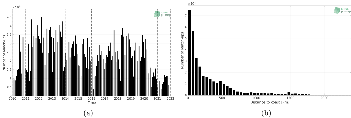
Figure 1: Number of match-ups between TSG (LEGOS-DM) and SMOS SSS L3 v8 - 9 Days (CATDS-CECOS-LOCEAN) SSS as a function of time (a) and as function of the distance to coast (b) over the North Atlantic Ocean Pi-MEP region and for the full satellite product period.
