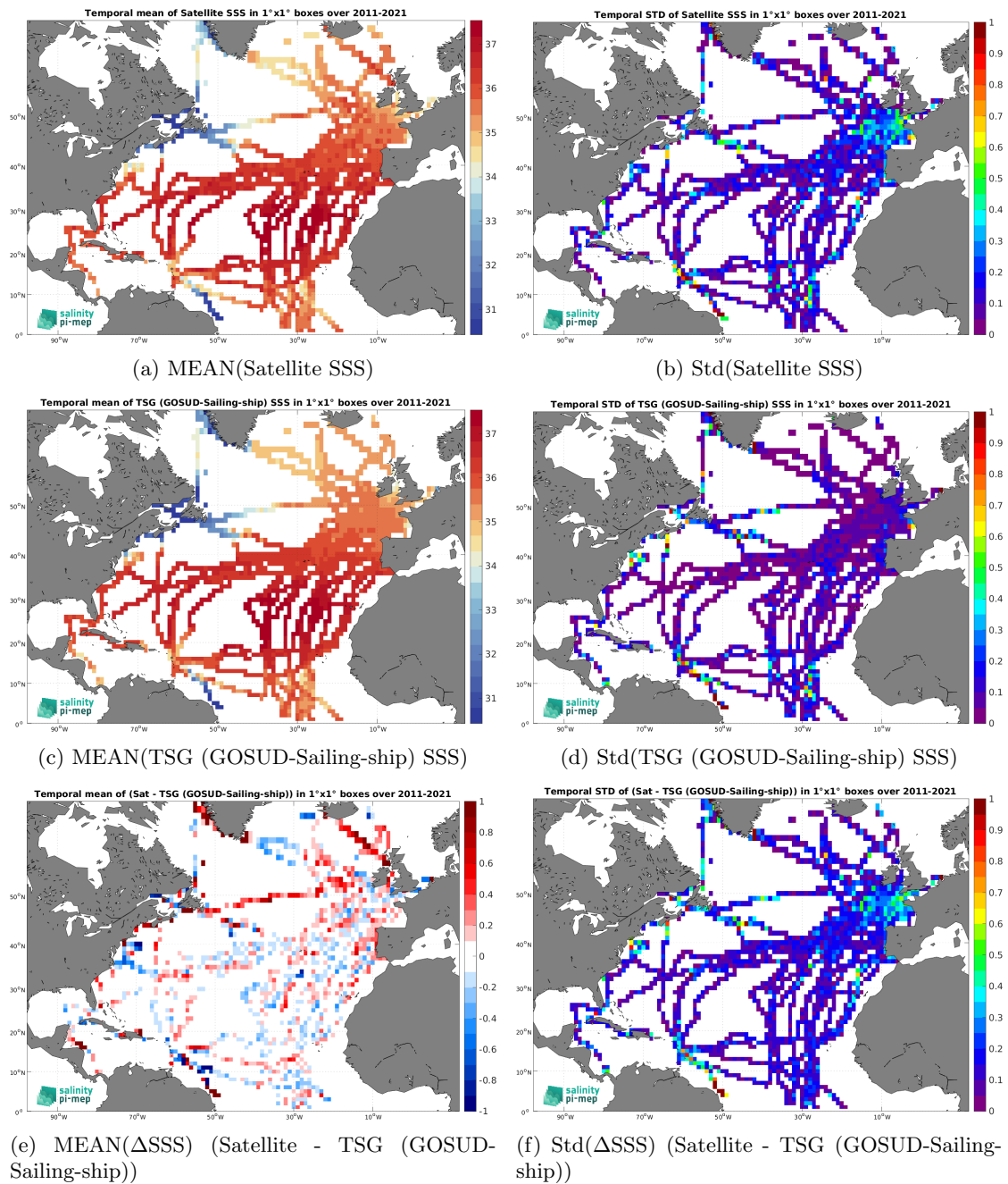
Figure 6: Temporal mean (left) and Std (right) of SSS from SMOS SSS L3 v8 - 9 Days (CATDS-CEC-LOCEAN) (top), TSG (GOSUD-Sailing-ship) (middle), and of \Delta SSS (Satellite - TSG (GOSUD-Sailing-ship)). Only match-up pairs are used to generate these maps.
