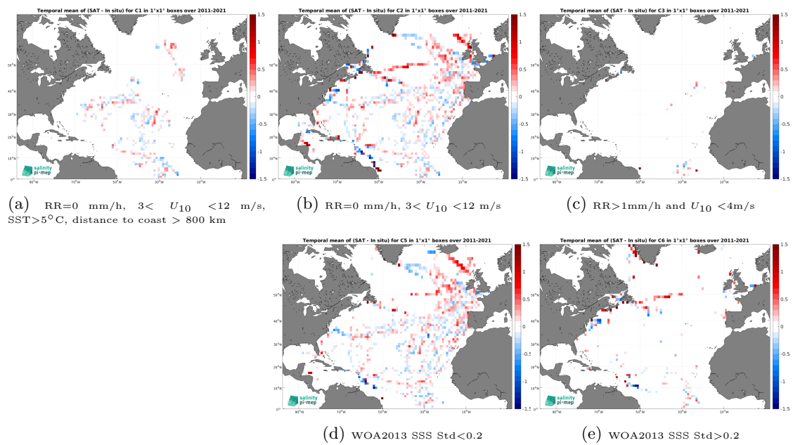
Figure 12: Temporal mean gridded over spatial boxes of size 1^\circ \times 1^\circ of \Delta\text{SSS} (SMOS SSS L3 v8 - 9 Days (CATDS-CEC-LOCEAN) - TSG (GOSUD-Sailing-ship)) for 5 different subdatasets corresponding to:RR=0 mm/h, 3 < U_{10} < 12 m/s, SST >5^\circ\text{C} , distance to coast > 800 km (a), RR=0 mm/h, 3 < U_{10} < 12 m/s (b), RR >1 mm/h and U_{10} < 4 m/s (c), WOA2013 SSS Std <0.2 (d), WOA2013 SSS Std >0.2 (e).
