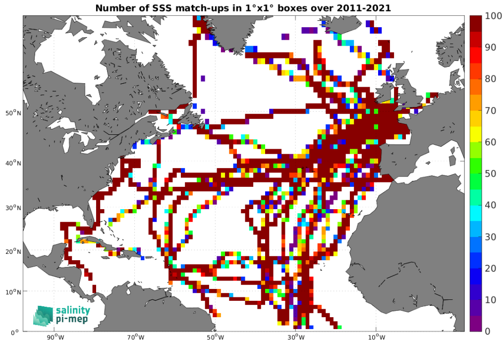
Figure 4: Number of SSS match-ups between TSG (GOSUD-Sailing-ship) SSS and the SMOS SSS L3 v8 - 9 Days (CATDS-CEC-LOCEAN) SSS product for the North Atlantic Ocean Pi-MEP region over 1^\circ \times 1^\circ boxes and for the full satellite product period.
