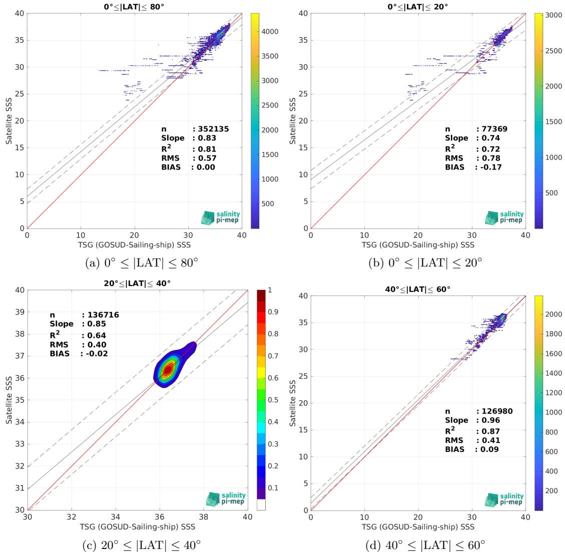
Figure 9: Contour maps of the concentration of SMOS SSS L3 v8 - 9 Days (CATDS-CEC-LOCEAN) SSS (y-axis) versus TSG (GOSUD-Sailing-ship) SSS (x-axis) at match-up pairs for different latitude bands. For each plot, the red line shows x=y . The black thin and dashed lines indicate a linear fit through the data cloud and the \pm 95\% confidence levels, respectively. The number match-up pairs n , the slope and R^2 coefficient of the linear fit, the root mean square (RMS) and the mean bias between satellite and in situ data are indicated for each latitude band in each plots.
