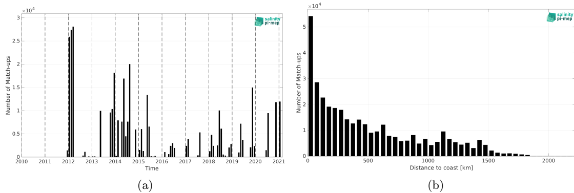
Figure 1: Number of match-ups between TSG (GOSUD-Sailing-ship) and SMOS SSS L3 v8 - 9 Days (CATDS-CEC-LOCEAN) SSS as a function of time (a) and as function of the distance to coast (b) over the North Atlantic Ocean Pi-MEP region and for the full satellite product period.
