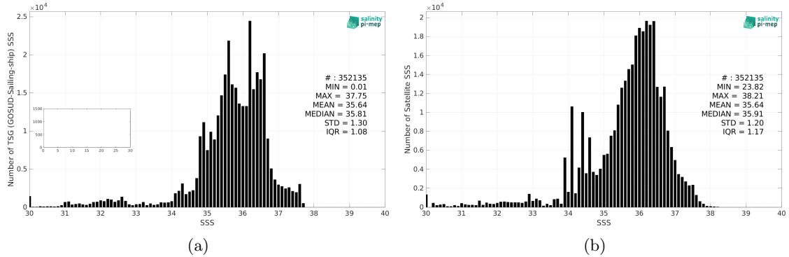
Figure 2: Histograms of SSS from TSG (GOSUD-Sailing-ship) (a) and SMOS SSS L3 v8 - 9 Days (CATDS-CEC-LOCEAN) (b) considering all match-up pairs per bins of 0.1 over the North Atlantic Ocean Pi-MEP region and for the full satellite product period.
