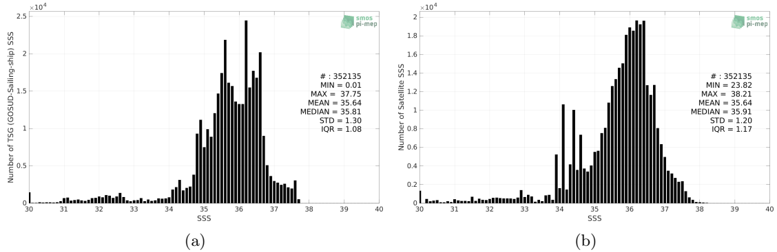
Figure 2: Histograms of SSS from TSG (GOSUD-Sailing-ship) (a) and SMOS SSS L3 v8 - 9 Days (CATDS-CECOS-LOCEAN) (b) considering all match-up pairs per bins of 0.1 over the North Atlantic Ocean Pi-MEP region and for the full satellite product period.
