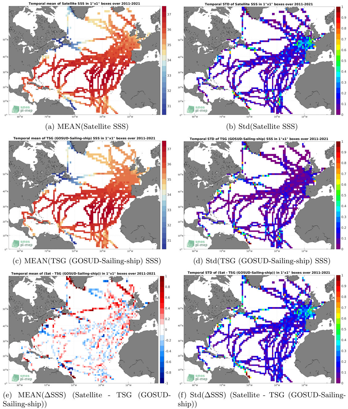
Figure 6: Temporal mean (left) and Std (right) of SSS from SMOS SSS L3 v8 - 9 Days (CATDS-CECOS-LOCEAN) (top), TSG (GOSUD-Sailing-ship) (middle), and of \Delta SSS (Satellite - TSG (GOSUD-Sailing-ship)). Only match-up pairs are used to generate these maps.
