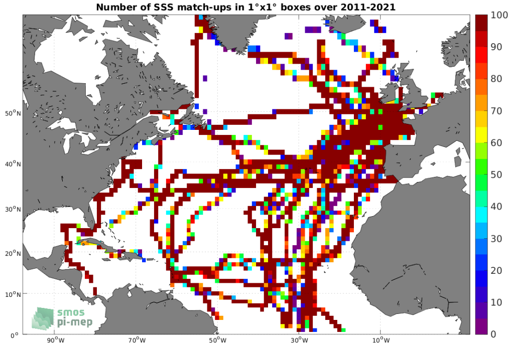
Figure 4: Number of SSS match-ups between TSG (GOSUD-Sailing-ship) SSS and the SMOS SSS L3 v8 - 9 Days (CATDS-CECOS-LOCEAN) SSS product for the North Atlantic Ocean Pi-MEP region over 1^\circ \times 1^\circ boxes and for the full satellite product period.
