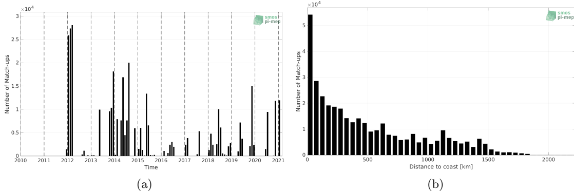
Figure 1: Number of match-ups between TSG (GOSUD-Sailing-ship) and SMOS SSS L3 v8 - 9 Days (CATDS-CECOS-LOCEAN) SSS as a function of time (a) and as function of the distance to coast (b) over the North Atlantic Ocean Pi-MEP region and for the full satellite product period.
