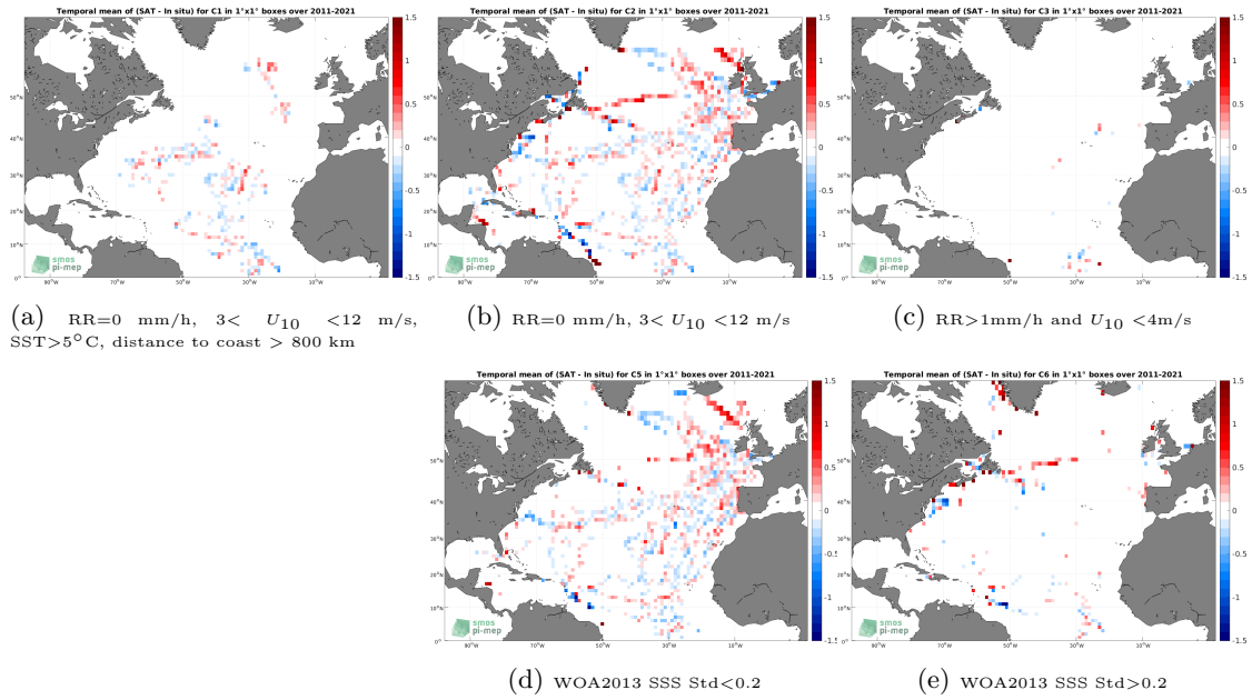
Figure 12: Temporal mean gridded over spatial boxes of size 1^\circ \times 1^\circ of \Delta SSS (SMOS SSS L3 v8 - 9 Days (CATDS-CECOS-LOCEAN) - TSG (GOSUD-Sailing-ship)) for 5 different subdatasets corresponding to:RR=0 mm/h, 3 < U_{10} < 12 m/s, SST>5°C, distance to coast > 800 km (a), RR=0 mm/h, 3 < U_{10} < 12 m/s (b), RR>1mm/h and U_{10} < 4 m/s (c), WOA2013 SSS Std<0.2 (d), WOA2013 SSS Std>0.2 (e).
