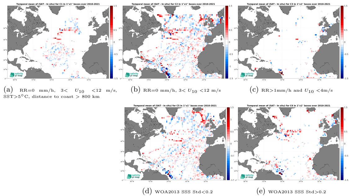
Figure 12: Temporal mean gridded over spatial boxes of size 1^\circ \times 1^\circ of \Delta\text{SSS} (SMOS SSS L3 v8 - 9 Days (CATDS-CEC-LOCEAN) - TSG (GOSUD-Research-vessel)) for 5 different subdatasets corresponding to:RR=0 mm/h, 3 < U_{10} < 12 m/s, SST > 5°C, distance to coast > 800 km (a), RR=0 mm/h, 3 < U_{10} < 12 m/s (b), RR > 1mm/h and U_{10} < 4 m/s (c), WOA2013 SSS Std < 0.2 (d), WOA2013 SSS Std > 0.2 (e).
