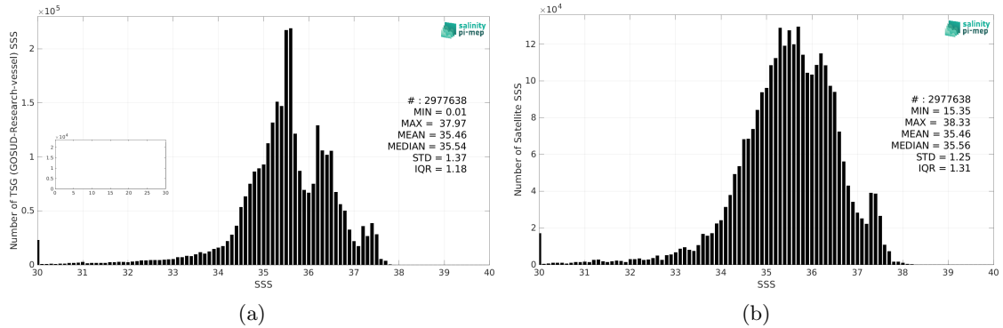
Figure 2: Histograms of SSS from TSG (GOSUD-Research-vessel) (a) and SMOS SSS L3 v8 - 9 Days (CATDS-CEC-LOCEAN) (b) considering all match-up pairs per bins of 0.1 over the North Atlantic Ocean Pi-MEP region and for the full satellite product period.
