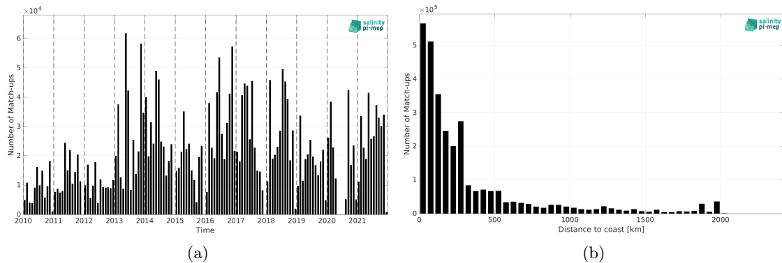
Figure 1: Number of match-ups between TSG (GOSUD-Research-vessel) and SMOS SSS L3 v8 - 9 Days (CATDS-CEC-LOCEAN) SSS as a function of time (a) and as function of the distance to coast (b) over the North Atlantic Ocean Pi-MEP region and for the full satellite product period.
