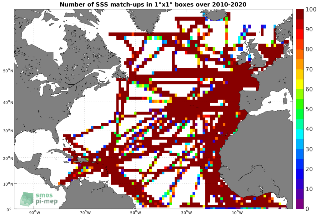
Figure 4: Number of SSS match-ups between TSG (GOSUD-Research-vessel) SSS and the SMOS SSS L3 v8 - 9 Days (CATDS-CECOS-LOCEAN) SSS product for the North Atlantic Ocean Pi-MEP region over 1^\circ \times 1^\circ boxes and for the full satellite product period.
