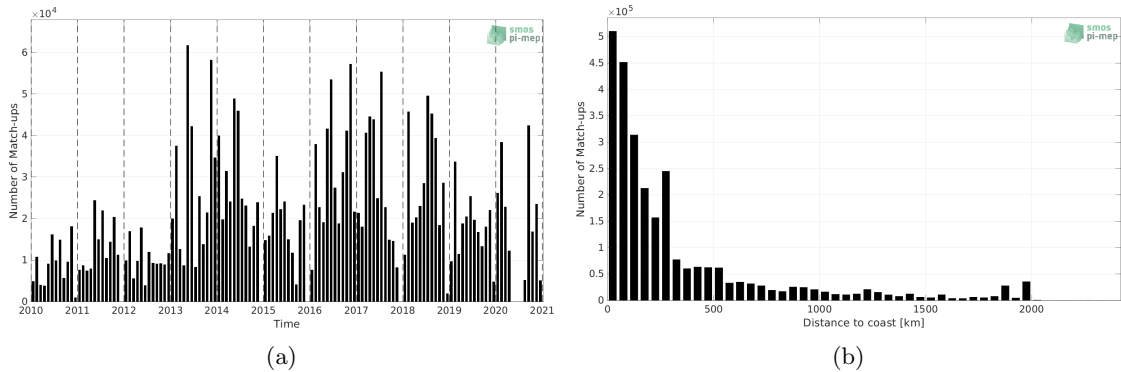
Figure 1: Number of match-ups between TSG (GOSUD-Research-vessel) and SMOS SSS L3 v8 - 9 Days (CATDS-CECOS-LOCEAN) SSS as a function of time (a) and as function of the distance to coast (b) over the North Atlantic Ocean Pi-MEP region and for the full satellite product period.
