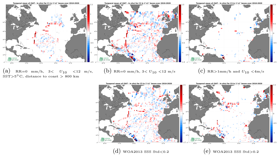
Figure 12: Temporal mean gridded over spatial boxes of size 1^\circ \times 1^\circ of \Delta\text{SSS} (SMOS SSS L3 v8 - 9 Days (CATDS-CECOS-LOCEAN) - TSG (GOSUD-Research-vessel)) for 5 different subdatasets corresponding to:RR=0 mm/h, 3 < U_{10} < 12 m/s, SST>5°C, distance to coast > 800 km (a), RR=0 mm/h, 3 < U_{10} < 12 m/s (b), RR>1mm/h and U_{10} < 4 m/s (c), WOA2013 SSS Std<0.2 (d), WOA2013 SSS Std>0.2 (e).
