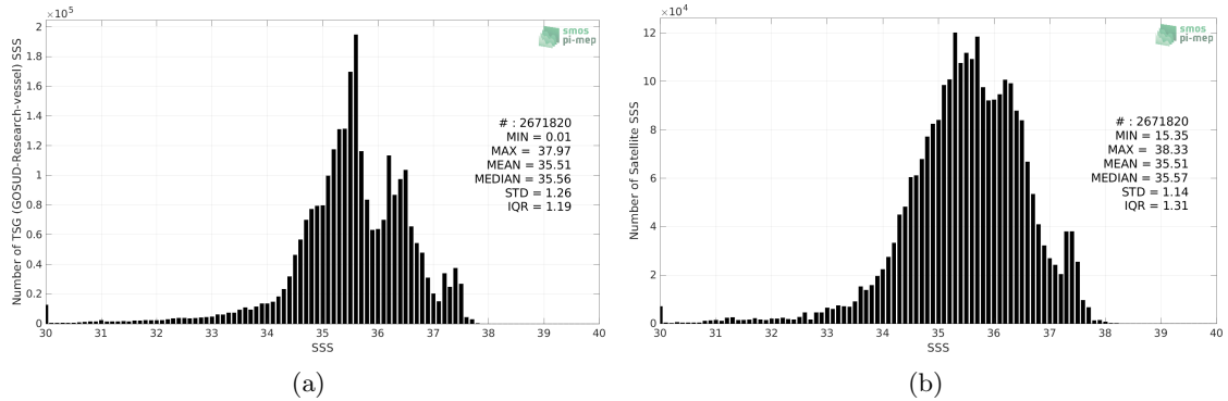
Figure 2: Histograms of SSS from TSG (GOSUD-Research-vessel) (a) and SMOS SSS L3 v8 - 9 Days (CATDS-CECOS-LOCEAN) (b) considering all match-up pairs per bins of 0.1 over the North Atlantic Ocean Pi-MEP region and for the full satellite product period.
