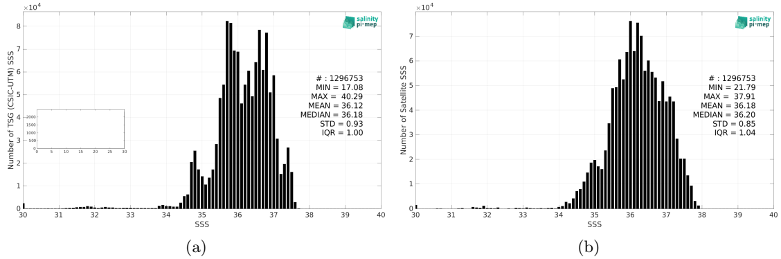
Figure 2: Histograms of SSS from TSG (CSIC-UTM) (a) and SMOS SSS L3 v8 - 9 Days (CATDS-CEC-LOCEAN) (b) considering all match-up pairs per bins of 0.1 over the North Atlantic Ocean Pi-MEP region and for the full satellite product period.
