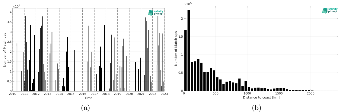
Figure 1: Number of match-ups between TSG (CSIC-UTM) and SMOS SSS L3 v8 - 9 Days (CATDS-CEC-LOCEAN) SSS as a function of time (a) and as function of the distance to coast (b) over the North Atlantic Ocean Pi-MEP region and for the full satellite product period.
