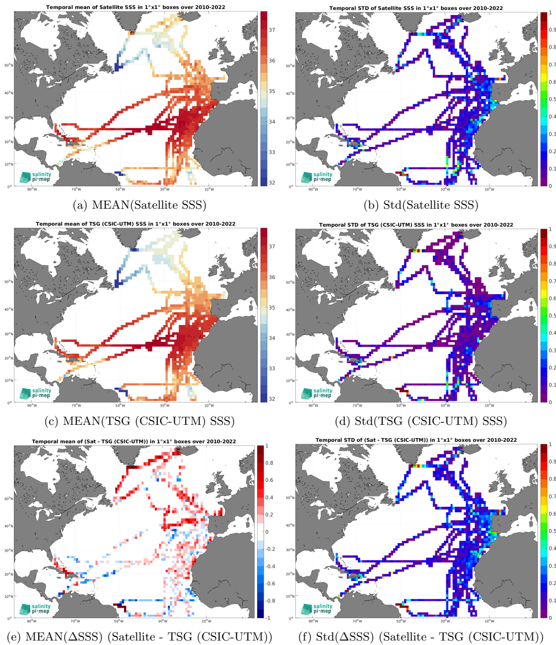
Figure 6: Temporal mean (left) and Std (right) of SSS from SMOS SSS L3 v8 - 9 Days (CATDS-CEC-LOCEAN) (top), TSG (CSIC-UTM) (middle), and of \Delta SSS (Satellite - TSG (CSIC-UTM)). Only match-up pairs are used to generate these maps.
