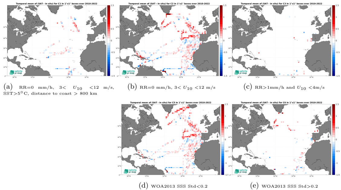
Figure 12: Temporal mean gridded over spatial boxes of size 1^\circ \times 1^\circ of \Delta SSS (SMOS SSS L3 v8 - 9 Days (CATDS-CEC-LOCEAN) - TSG (CSIC-UTM)) for 5 different subdatasets corresponding to:RR=0 mm/h, 3 < U_{10} < 12 m/s, SST >5^\circ\text{C} , distance to coast > 800 km (a), RR=0 mm/h, 3 < U_{10} < 12 m/s (b), RR >1 mm/h and U_{10} < 4 m/s (c), WOA2013 SSS Std <0.2 (d), WOA2013 SSS Std >0.2 (e).
