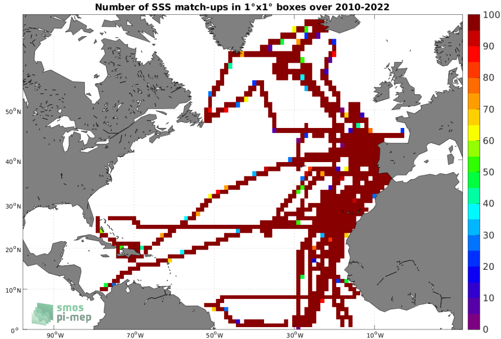
Figure 4: Number of SSS match-ups between TSG (CSIC-UTM) SSS and the SMOS SSS L3 v8 - 9 Days (CATDS-CECOS-LOCEAN) SSS product for the North Atlantic Ocean Pi-MEP region over 1^\circ \times 1^\circ boxes and for the full satellite product period.
