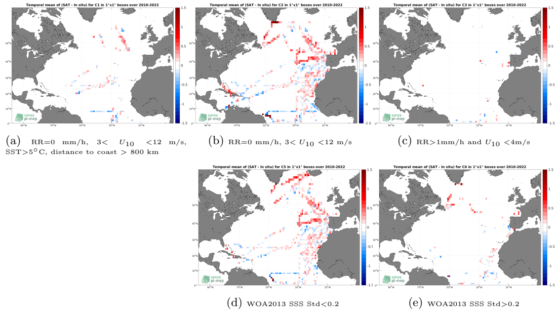
Figure 12: Temporal mean gridded over spatial boxes of size 1^\circ \times 1^\circ of \Delta SSS (SMOS SSS L3 v8 - 9 Days (CATDS-CECOS-LOCEAN) - TSG (CSIC-UTM)) for 5 different subdatasets corresponding to:RR=0 mm/h, 3 < U_{10} < 12 m/s, SST >5^\circ\text{C} , distance to coast > 800 km (a), RR=0 mm/h, 3 < U_{10} < 12 m/s (b), RR >1 mm/h and U_{10} < 4 m/s (c), WOA2013 SSS Std <0.2 (d), WOA2013 SSS Std >0.2 (e).
