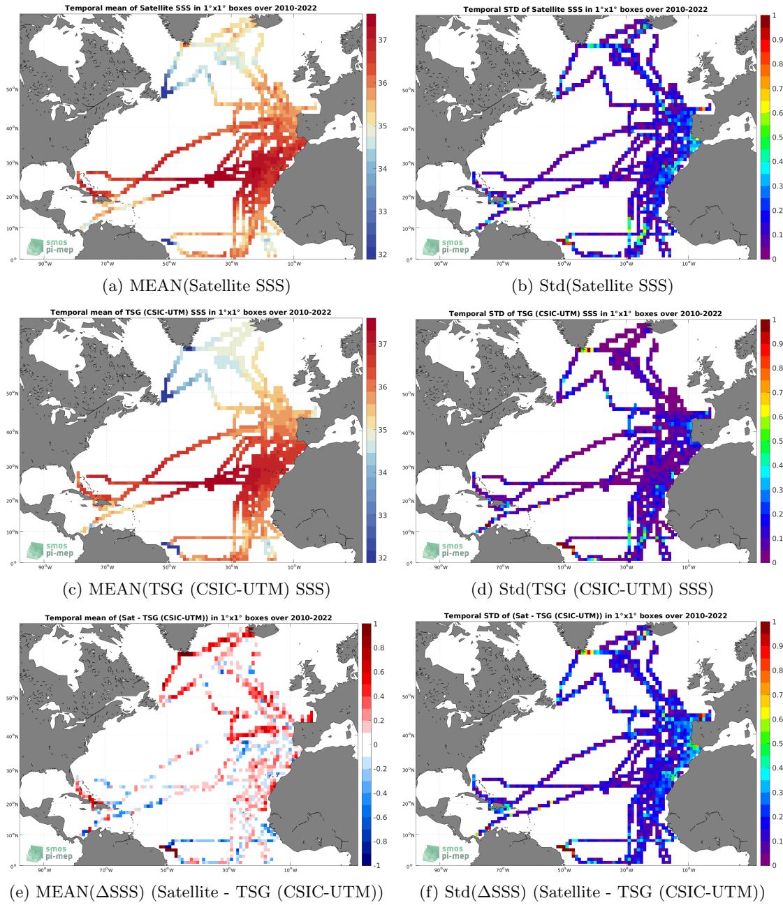
Figure 6: Temporal mean (left) and Std (right) of SSS from SMOS SSS L3 v8 - 9 Days (CATDS-CECOS-LOCEAN) (top), TSG (CSIC-UTM) (middle), and of \Delta SSS (Satellite - TSG (CSIC-UTM)). Only match-up pairs are used to generate these maps.
