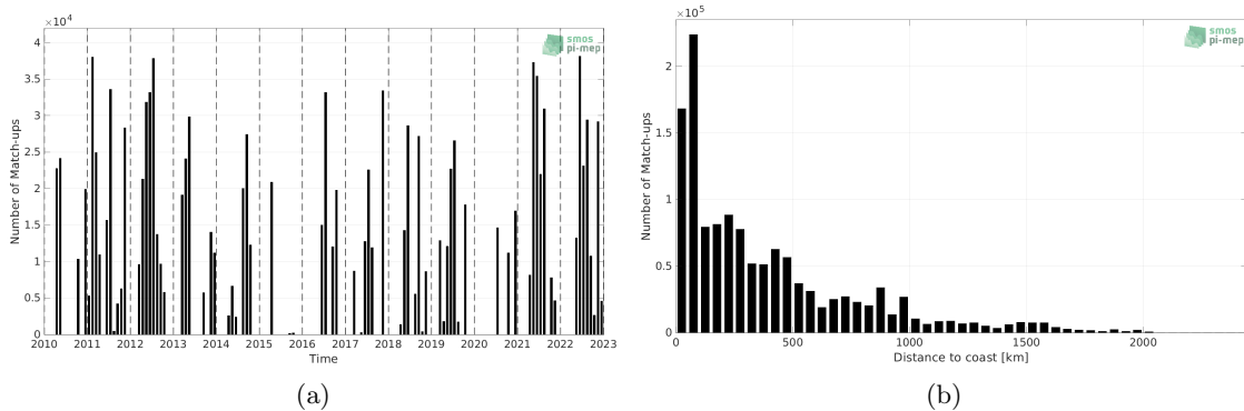
Figure 1: Number of match-ups between TSG (CSIC-UTM) and SMOS SSS L3 v8 - 9 Days (CATDS-CECOS-LOCEAN) SSS as a function of time (a) and as function of the distance to coast (b) over the North Atlantic Ocean Pi-MEP region and for the full satellite product period.
