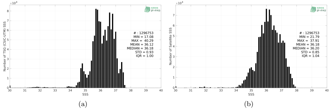
Figure 2: Histograms of SSS from TSG (CSIC-UTM) (a) and SMOS SSS L3 v8 - 9 Days (CATDS-CECOS-LOCEAN) (b) considering all match-up pairs per bins of 0.1 over the North Atlantic Ocean Pi-MEP region and for the full satellite product period.
