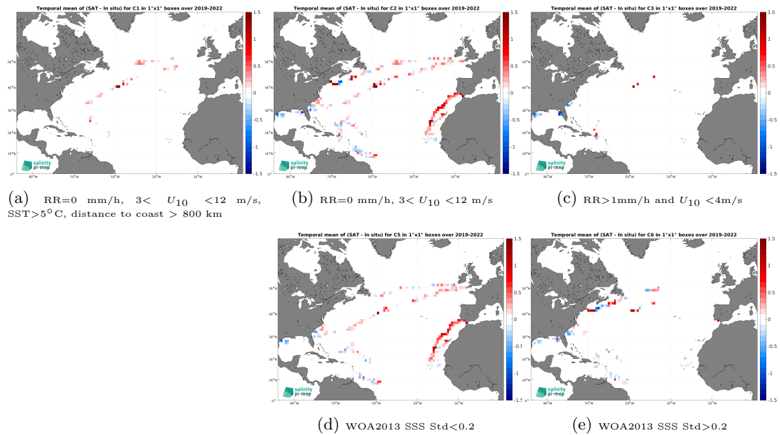
Figure 12: Temporal mean gridded over spatial boxes of size 1^\circ \times 1^\circ of \Delta\text{SSS} (SMOS SSS L3 v8 - 9 Days (CATDS-CEC-LOCEAN) - Saildrone) for 5 different subdatasets corresponding to:RR=0 mm/h, 3 < U_{10} < 12 m/s, SST >5^\circ\text{C} , distance to coast > 800 km (a), RR=0 mm/h, 3 < U_{10} < 12 m/s (b), RR >1 mm/h and U_{10} < 4 m/s (c), WOA2013 SSS Std <0.2 (d), WOA2013 SSS Std >0.2 (e).
