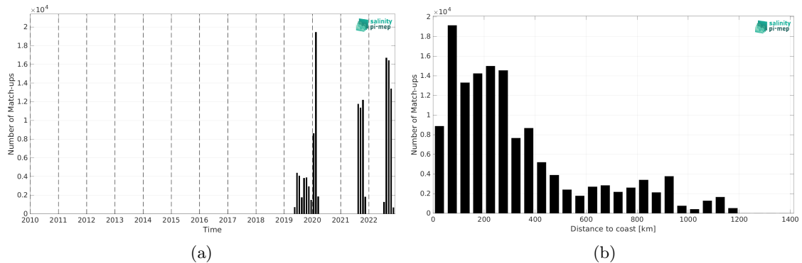
Figure 1: Number of match-ups between Saildrone and SMOS SSS L3 v8 - 9 Days (CATDS-CEC-LOCEAN) SSS as a function of time (a) and as function of the distance to coast (b) over the North Atlantic Ocean Pi-MEP region and for the full satellite product period.
