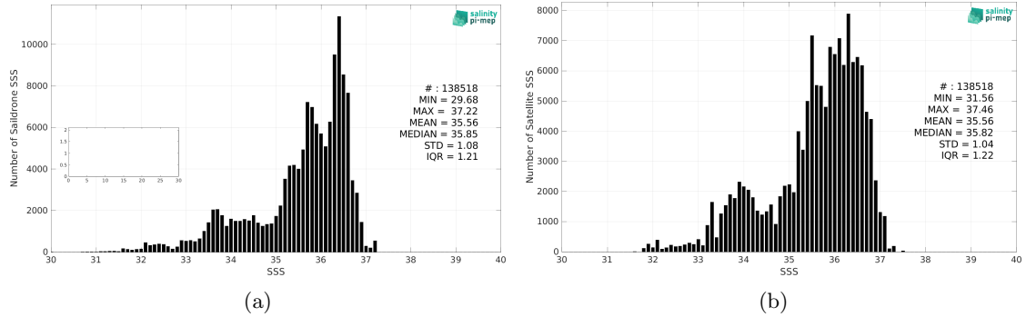
Figure 2: Histograms of SSS from Saildrone (a) and SMOS SSS L3 v8 - 9 Days (CATDS-CEC-LOCEAN) (b) considering all match-up pairs per bins of 0.1 over the North Atlantic Ocean Pi-MEP region and for the full satellite product period.
