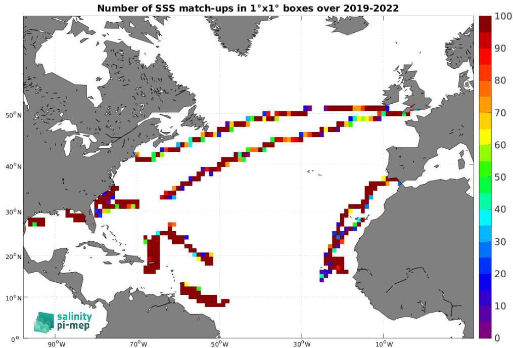
Figure 4: Number of SSS match-ups between Saildrone SSS and the SMOS SSS L3 v8 - 9 Days (CATDS-CEC-LOCEAN) SSS product for the North Atlantic Ocean Pi-MEP region over 1^\circ \times 1^\circ boxes and for the full satellite product period.
