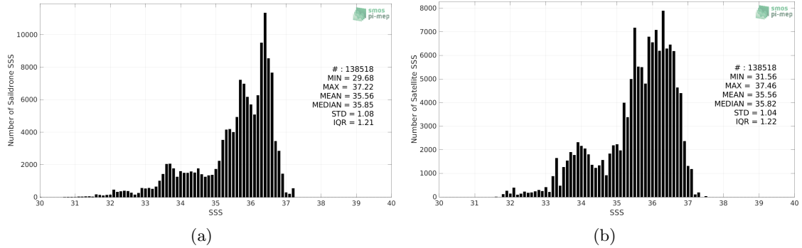
Figure 2: Histograms of SSS from Saildrone (a) and SMOS SSS L3 v8 - 9 Days (CATDS-CECOS-LOCEAN) (b) considering all match-up pairs per bins of 0.1 over the North Atlantic Ocean Pi-MEP region and for the full satellite product period.
