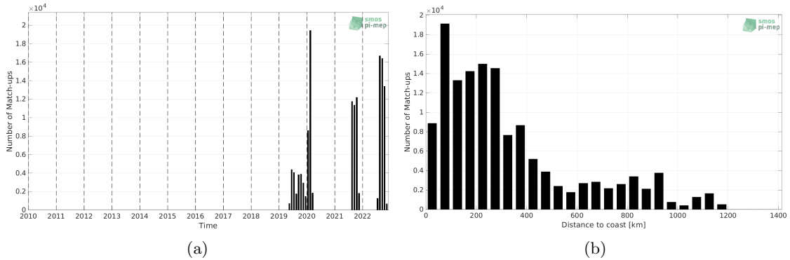
Figure 1: Number of match-ups between Saildrone and SMOS SSS L3 v8 - 9 Days (CATDS-CECOS-LOCEAN) SSS as a function of time (a) and as function of the distance to coast (b) over the North Atlantic Ocean Pi-MEP region and for the full satellite product period.
