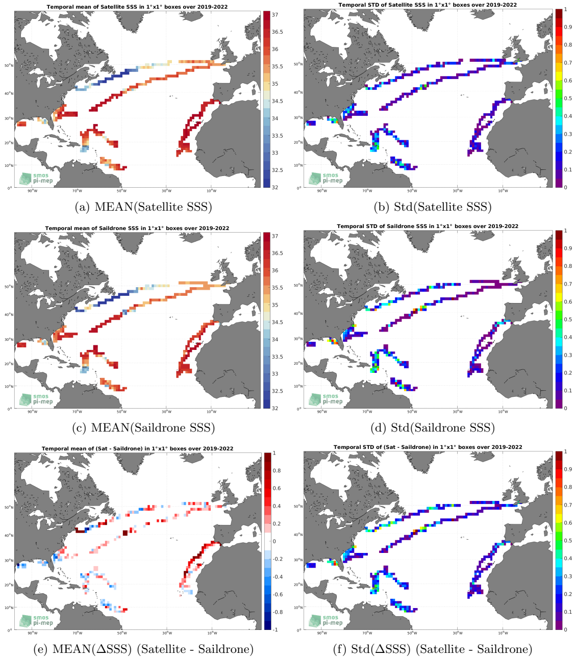
Figure 6: Temporal mean (left) and Std (right) of SSS from SMOS SSS L3 v8 - 9 Days (CATDS-CECOS-LOCEAN) (top), Saildrone (middle), and of \Delta SSS (Satellite - Saildrone). Only match-pairs are used to generate these maps.
