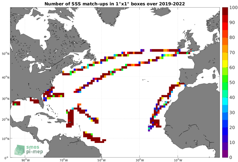
Figure 4: Number of SSS match-ups between Saildrone SSS and the SMOS SSS L3 v8 - 9 Days (CATDS-CECOS-LOCEAN) SSS product for the North Atlantic Ocean Pi-MEP region over 1^\circ \times 1^\circ boxes and for the full satellite product period.
