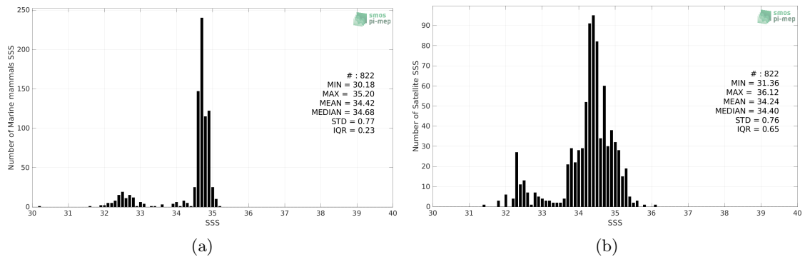
Figure 2: Histograms of SSS from Marine mammals (a) and SMOS SSS L3 v8 - 9 Days (CATDS-CECOS-LOCEAN) (b) considering all match-up pairs per bins of 0.1 over the North Atlantic Ocean Pi-MEP region and for the full satellite product period.
