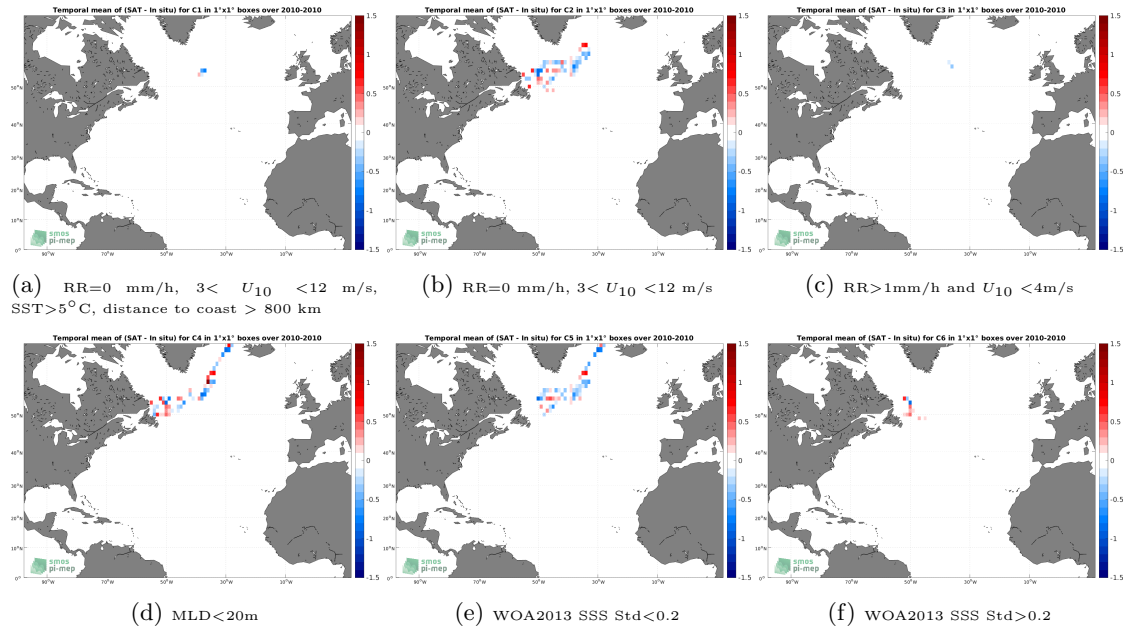
Figure 12: Temporal mean gridded over spatial boxes of size 1^{\circ}\times 1^{\circ} of \Delta\text{SSS} (SMOS SSS L3 v8 - 9 Days (CATDS-CECOS-LOCEAN) - Marine mammals) for 6 different subdatasets corresponding to:RR=0 mm/h, 3 < U_{10} < 12 m/s, SST >5^{\circ}\text{C} , distance to coast > 800 km (a), RR=0 mm/h, 3 < U_{10} < 12 m/s (b), RR >1\text{mm/h} and U_{10} < 4\text{m/s} (c),MLD <20\text{m} (d),WOA2013 SSS Std <0.2 (e),WOA2013 SSS Std >0.2 (f).
