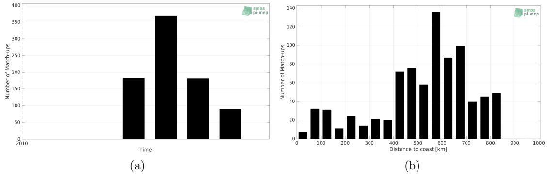
Figure 1: Number of match-ups between Marine mammals and SMOS SSS L3 v8 - 9 Days (CATDS-CECOS-LOCEAN) SSS as a function of time (a) and as function of the distance to coast (b) over the North Atlantic Ocean Pi-MEP region and for the full satellite product period.
