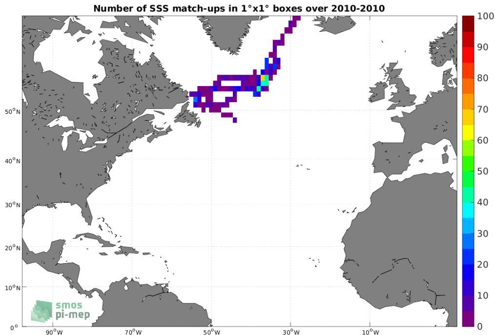
Figure 4: Number of SSS match-ups between Marine mammals SSS and the SMOS SSS L3 v8 - 9 Days (CATDS-CECOS-LOCEAN) SSS product for the North Atlantic Ocean Pi-MEP region over 1^\circ \times 1^\circ boxes and for the full satellite product period.
