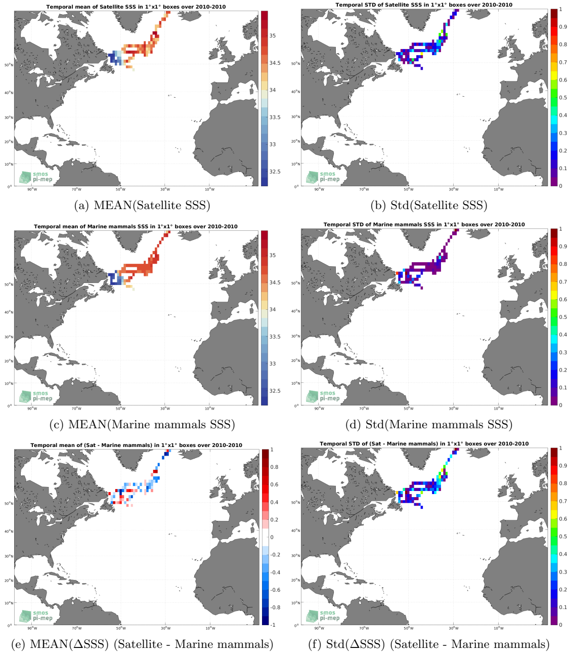
Figure 6: Temporal mean (left) and Std (right) of SSS from SMOS SSS L3 v8 - 9 Days (CATDS-CECOS-LOCEAN) (top), Marine mammals (middle), and of \Delta SSS (Satellite - Marine mammals). Only match-up pairs are used to generate these maps.
