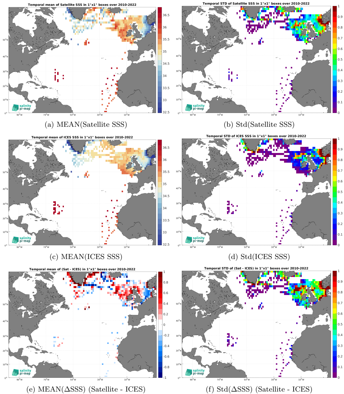
Figure 6: Temporal mean (left) and Std (right) of SSS from SMOS SSS L3 v8 - 9 Days (CATDS-CEC-LOCEAN) (top), ICES (middle), and of \Delta SSS (Satellite - ICES). Only match-up pairs are used to generate these maps.
