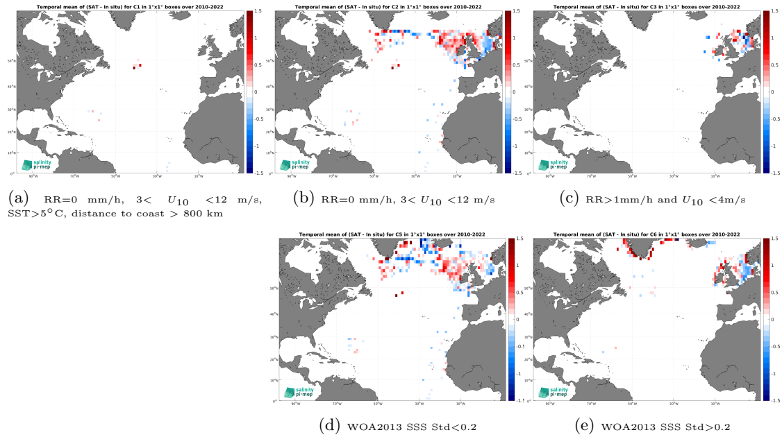
Figure 12: Temporal mean gridded over spatial boxes of size 1^\circ \times 1^\circ of \Delta\text{SSS} (SMOS SSS L3 v8 - 9 Days (CATDS-CEC-LOCEAN) - ICES) for 5 different subdatasets corresponding to:RR=0 mm/h, 3 < U_{10} < 12 m/s, SST >5^\circ\text{C} , distance to coast > 800 km (a), RR=0 mm/h, 3 < U_{10} < 12 m/s (b), RR >1 mm/h and U_{10} < 4 m/s (c), WOA2013 SSS Std <0.2 (d), WOA2013 SSS Std >0.2 (e).
