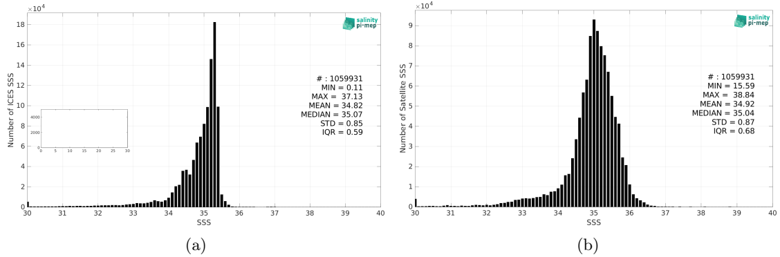
Figure 2: Histograms of SSS from ICES (a) and SMOS SSS L3 v8 - 9 Days (CATDS-CEC-LOCEAN) (b) considering all match-up pairs per bins of 0.1 over the North Atlantic Ocean Pi-MEP region and for the full satellite product period.
