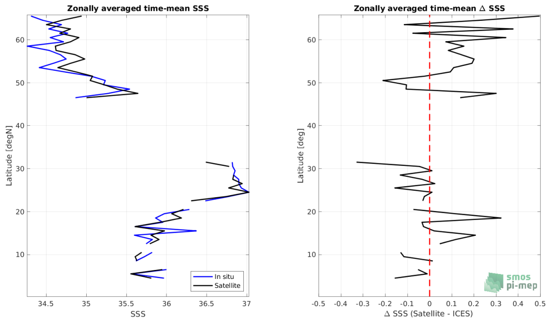
Figure 8: Left panel: Zonal mean SSS from SMOS SSS L3 v8 - 9 Days (CATDS-CECOS-LOCEAN) satellite product (black) and from ICES (blue). Right panel: Zonal mean of \Delta SSS (Satellite - ICES) for all the collected Pi-MEP match-up pairs estimated over the full satellite product period.
