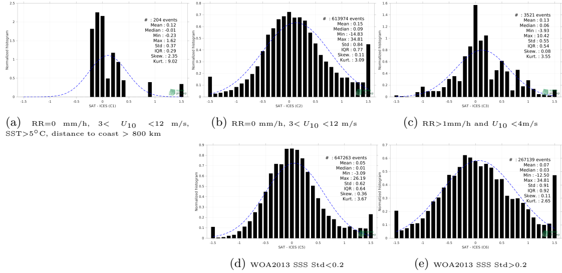
Figure 13: Normalized histogram of \Delta SSS (SMOS SSS L3 v8 - 9 Days (CATDS-CECOS-LOCEAN) - ICES) for 5 different subdatasets corresponding to: RR=0 mm/h, 3 < U_{10} < 12 m/s, SST > 5°C, distance to coast > 800 km (a), RR=0 mm/h, 3 < U_{10} < 12 m/s (b), RR > 1mm/h and U_{10} < 4 m/s (c), WOA2013 SSS Std < 0.2 (d), WOA2013 SSS Std > 0.2 (e).
