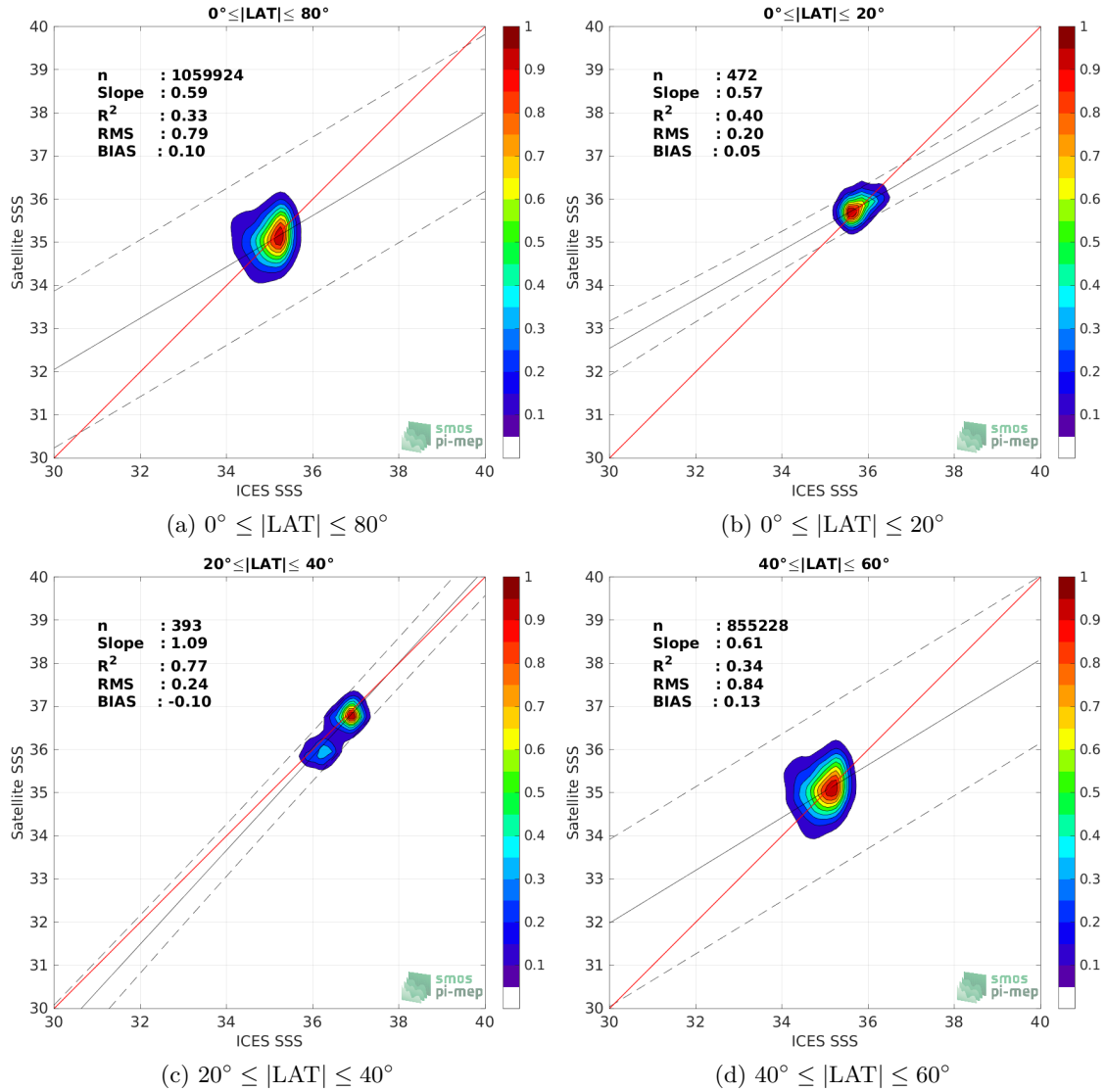
Figure 9: Contour maps of the concentration of SMOS SSS L3 v8 - 9 Days (CATDS-CECOS-LOCEAN) SSS (y-axis) versus ICES SSS (x-axis) at match-up pairs for different latitude bands. For each plot, the red line shows x=y . The black thin and dashed lines indicate a linear fit through the data cloud and the \pm 95\% confidence levels, respectively. The number match-up pairs n , the slope and R^2 coefficient of the linear fit, the root mean square (RMS) and the mean bias between satellite and in situ data are indicated for each latitude band in each plots.
