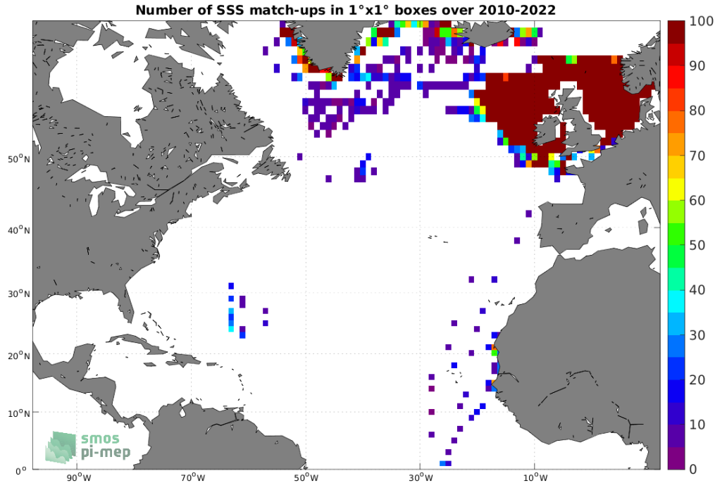
Figure 4: Number of SSS match-ups between ICES SSS and the SMOS SSS L3 v8 - 9 Days (CATDS-CECOS-LOCEAN) SSS product for the North Atlantic Ocean Pi-MEP region over 1^\circ \times 1^\circ boxes and for the full satellite product period.
