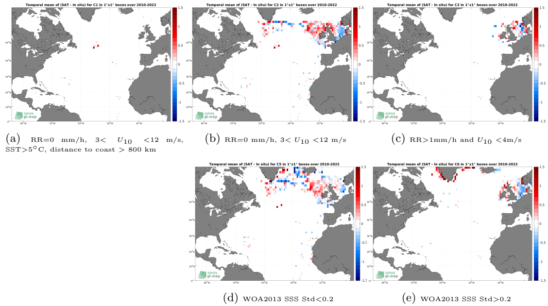
Figure 12: Temporal mean gridded over spatial boxes of size 1^\circ \times 1^\circ of \Delta\text{SSS} (SMOS SSS L3 v8 - 9 Days (CATDS-CECOS-LOCEAN) - ICES) for 5 different subdatasets corresponding to:RR=0 mm/h, 3 < U_{10} < 12 m/s, SST >5^\circ\text{C} , distance to coast > 800 km (a), RR=0 mm/h, 3 < U_{10} < 12 m/s (b), RR >1 mm/h and U_{10} < 4 m/s (c), WOA2013 SSS Std <0.2 (d), WOA2013 SSS Std >0.2 (e).
