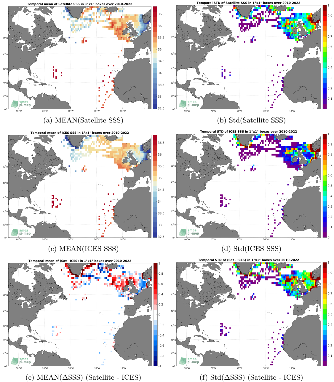
Figure 6: Temporal mean (left) and Std (right) of SSS from SMOS SSS L3 v8 - 9 Days (CATDS-CECOS-LOCEAN) (top), ICES (middle), and of \Delta SSS (Satellite - ICES). Only match-up pairs are used to generate these maps.
