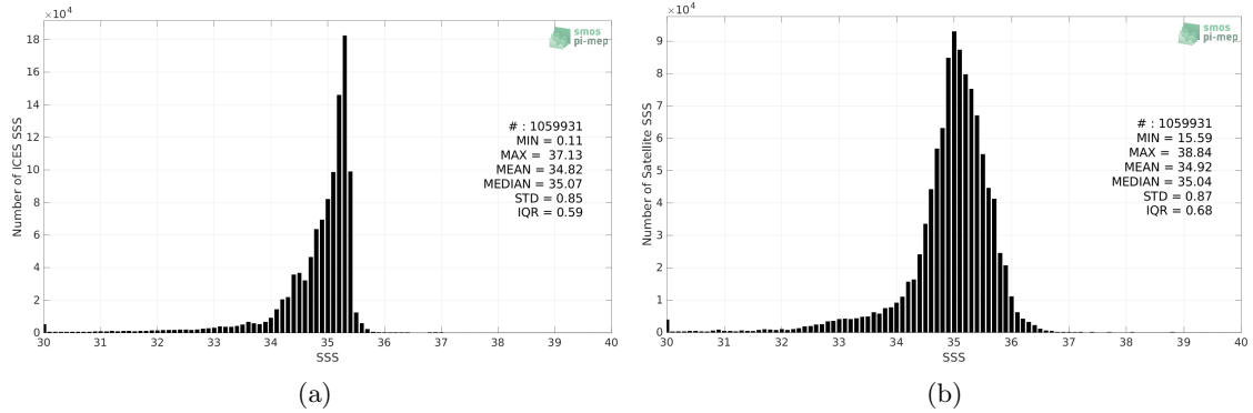
Figure 2: Histograms of SSS from ICES (a) and SMOS SSS L3 v8 - 9 Days (CATDS-CECOS-LOCEAN) (b) considering all match-up pairs per bins of 0.1 over the North Atlantic Ocean Pi-MEP region and for the full satellite product period.
