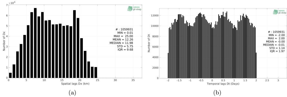
Figure 5: Histograms of the spatial (a) and temporal (b) lags between the location/time of the ICES measurement and the date of the corresponding SMOS SSS L3 v8 - 9 Days (CATDS-CECOS-LOCEAN) SSS pixel.
