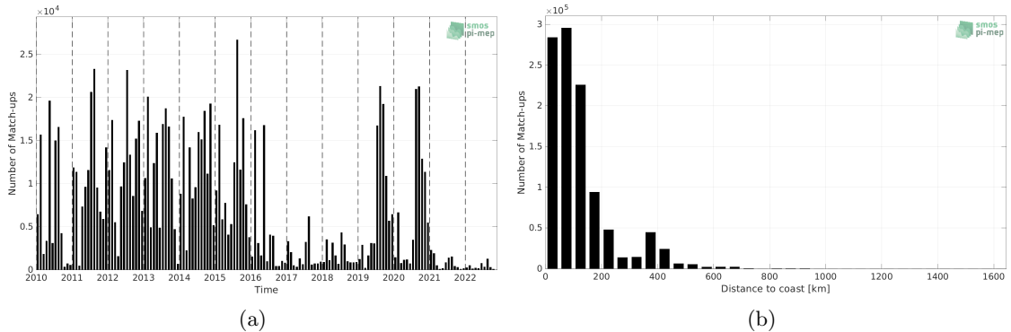
Figure 1: Number of match-ups between ICES and SMOS SSS L3 v8 - 9 Days (CATDS-CECOS-LOCEAN) SSS as a function of time (a) and as function of the distance to coast (b) over the North Atlantic Ocean Pi-MEP region and for the full satellite product period.
