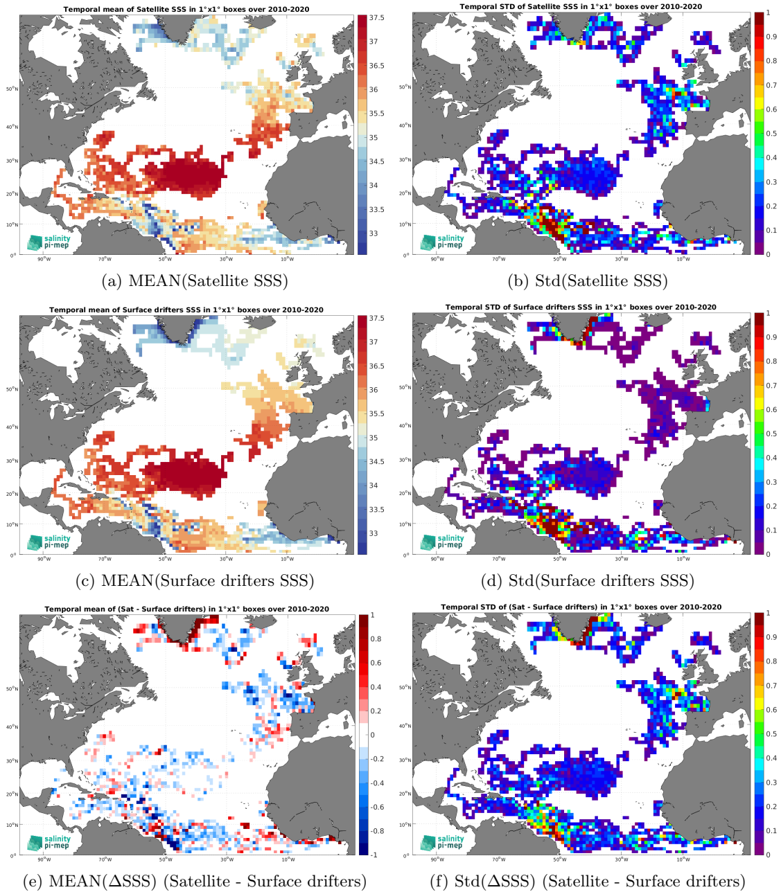
Figure 5: Temporal mean (left) and Std (right) of SSS from SMOS SSS L3 v8 - 9 Days (CATDS-CEC-LOCEAN) (top), Surface drifters (middle), and of \Delta SSS (Satellite - Surface drifters). Only match-up pairs are used to generate these maps.
