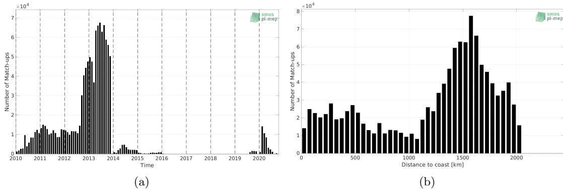
Figure 1: Number of match-ups between Surface drifters and SMOS SSS L3 v8 - 9 Days (CATDS-CECOS-LOCEAN) SSS as a function of time (a) and as function of the distance to coast (b) over the North Atlantic Ocean Pi-MEP region and for the full satellite product period.
