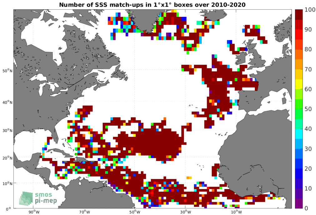
Figure 3: Number of SSS match-ups between Surface drifters SSS and the SMOS SSS L3 v8 - 9 Days (CATDS-CECOS-LOCEAN) SSS product for the North Atlantic Ocean Pi-MEP region over 1^\circ \times 1^\circ boxes and for the full satellite product period.
