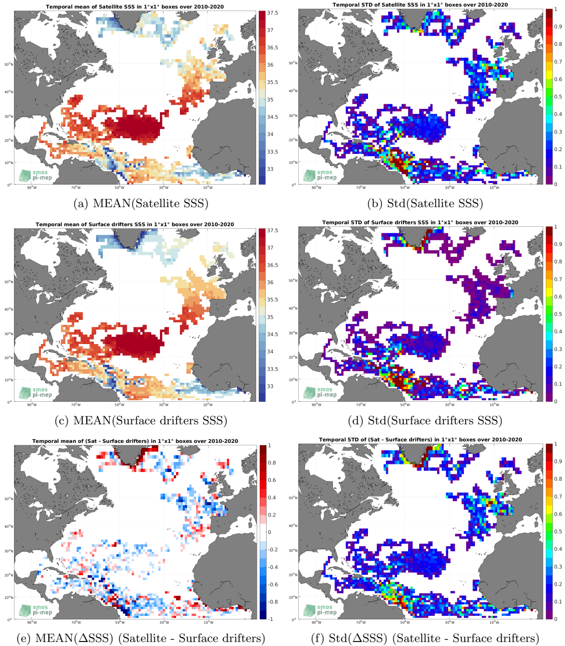
Figure 5: Temporal mean (left) and Std (right) of SSS from SMOS SSS L3 v8 - 9 Days (CATDS-CECOS-LOCEAN) (top), Surface drifters (middle), and of \Delta SSS (Satellite - Surface drifters). Only match-up pairs are used to generate these maps.
