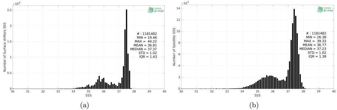
Figure 2: Histograms of SSS from Surface drifters (a) and SMOS SSS L3 v8 - 9 Days (CATDS-CECOS-LOCEAN) (b) considering all match-up pairs per bins of 0.1 over the North Atlantic Ocean Pi-MEP region and for the full satellite product period.
