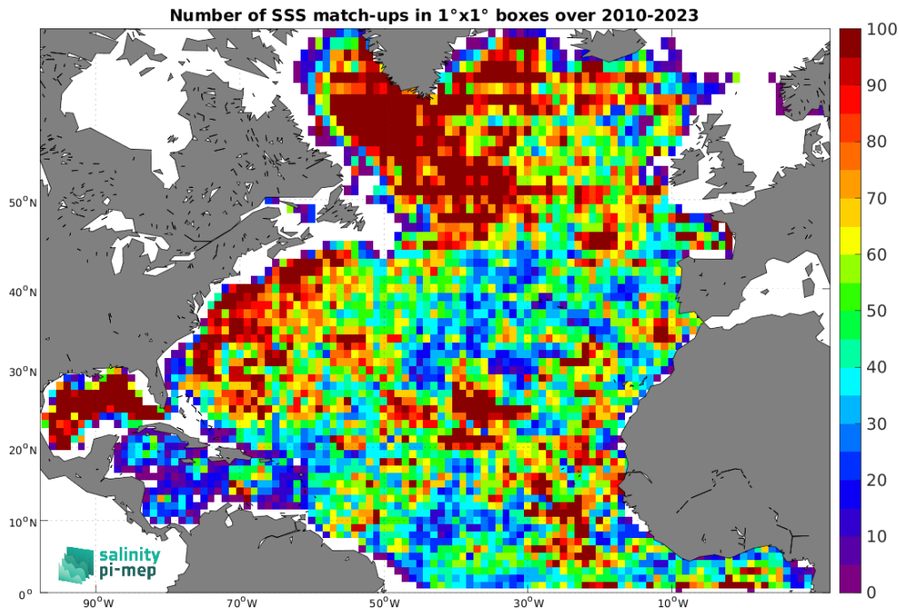
Figure 4: Number of SSS match-ups between Argo SSS and the SMOS SSS L3 v8 - 9 Days (CATDS-CEC-LOCEAN) SSS product for the North Atlantic Ocean Pi-MEP region over 1^\circ \times 1^\circ boxes and for the full satellite product period.
