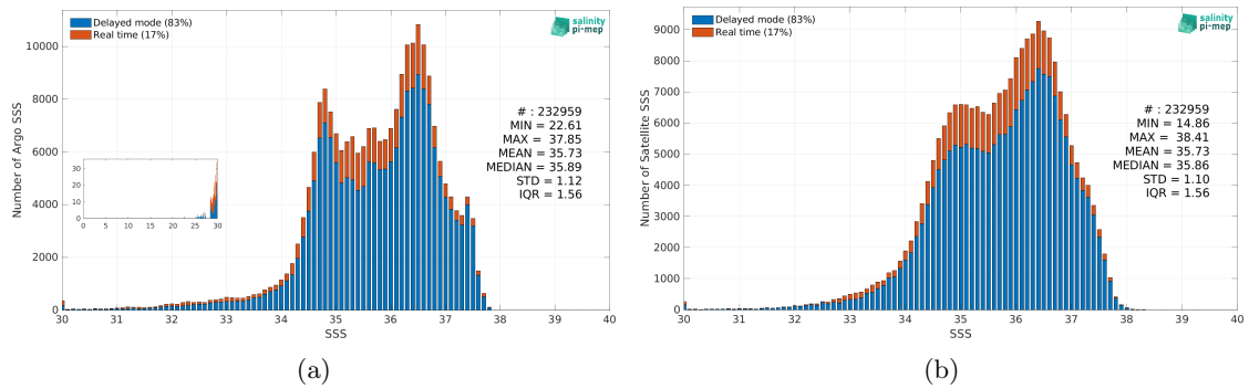
Figure 2: Histograms of SSS from Argo (a) and SMOS SSS L3 v8 - 9 Days (CATDS-CEC-LOCEAN) (b) considering all match-up pairs per bins of 0.1 over the North Atlantic Ocean Pi-MEP region and for the full satellite product period.
