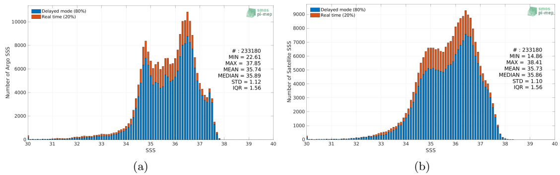
Figure 2: Histograms of SSS from Argo (a) and SMOS SSS L3 v8 - 9 Days (CATDS-CECOS-LOCEAN) (b) considering all match-up pairs per bins of 0.1 over the North Atlantic Ocean Pi-MEP region and for the full satellite product period.
