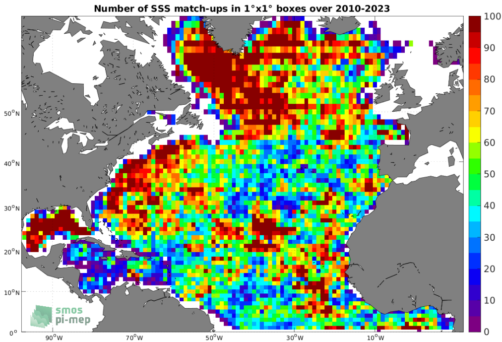
Figure 4: Number of SSS match-ups between Argo SSS and the SMOS SSS L3 v8 - 9 Days (CATDS-CECOS-LOCEAN) SSS product for the North Atlantic Ocean Pi-MEP region over 1^\circ \times 1^\circ boxes and for the full satellite product period.
