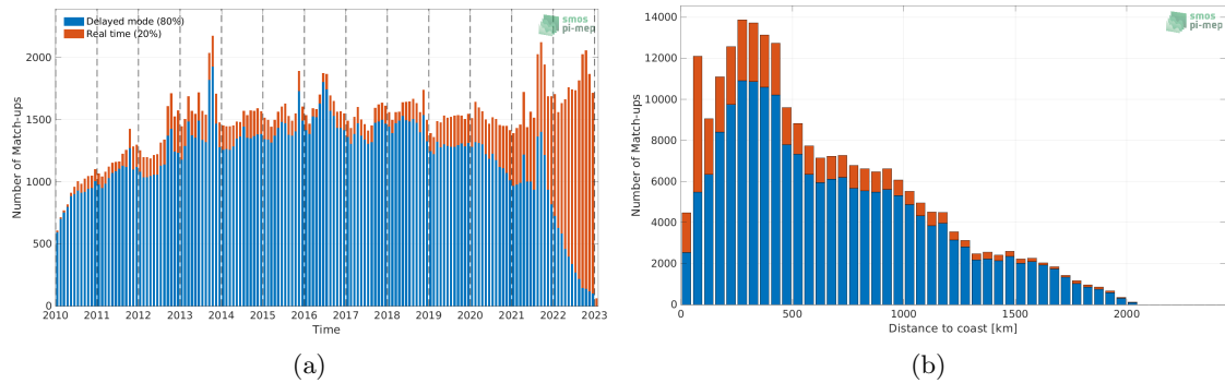
Figure 1: Number of match-ups between Argo and SMOS SSS L3 v8 - 9 Days (CATDS-CECOS-LOCEAN) SSS as a function of time (a) and as function of the distance to coast (b) over the North Atlantic Ocean Pi-MEP region and for the full satellite product period.
