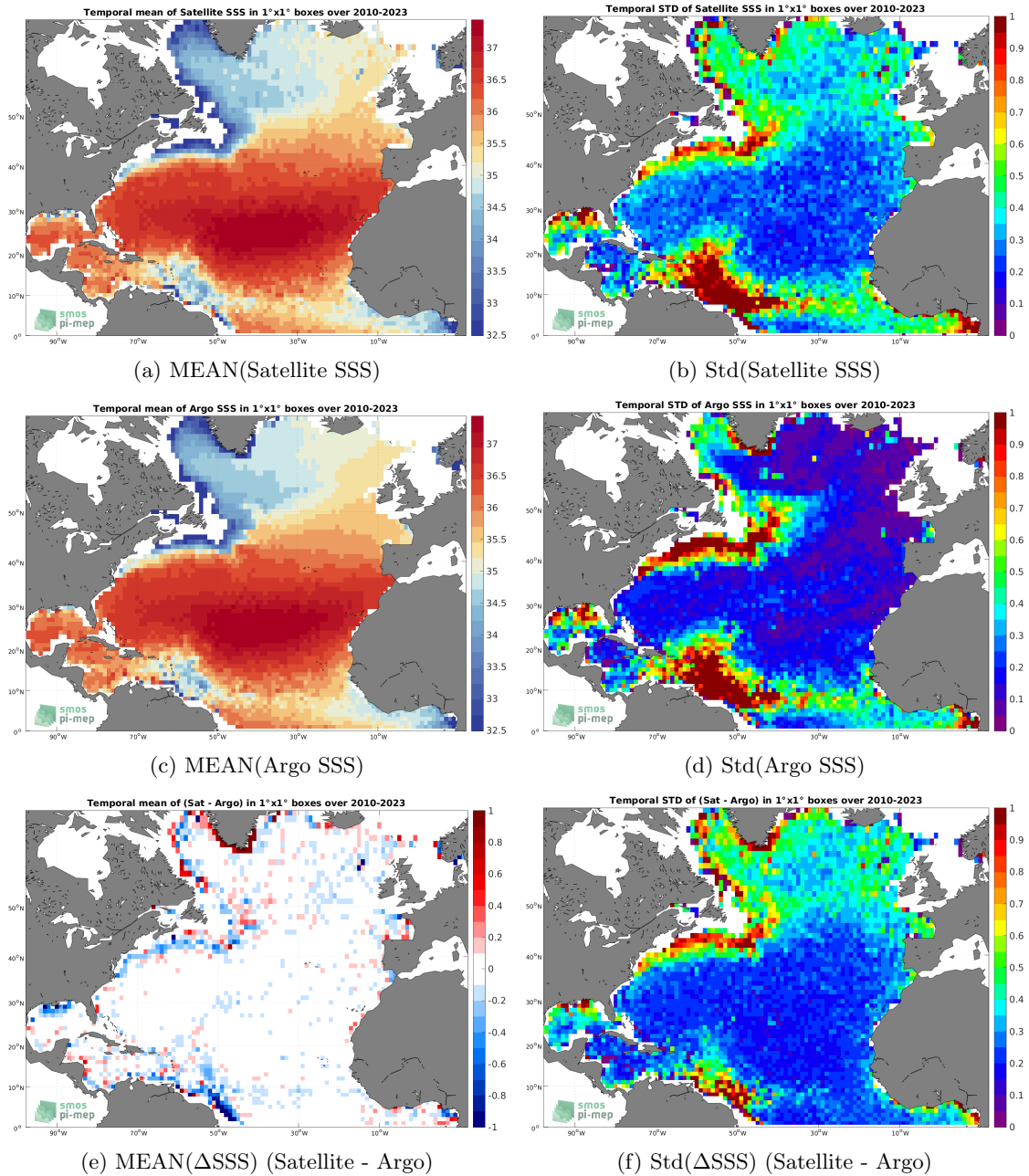
Figure 6: Temporal mean (left) and Std (right) of SSS from SMOS SSS L3 v8 - 9 Days (CATDS-CECOS-LOCEAN) (top), Argo (middle), and of \Delta SSS (Satellite - Argo). Only match-up pairs are used to generate these maps.
