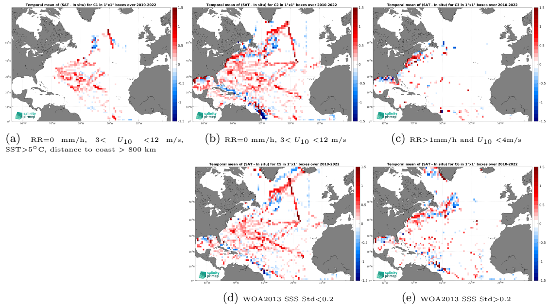
Figure 12: Temporal mean gridded over spatial boxes of size 1^\circ \times 1^\circ of \Delta\text{SSS} (SMOS SSS L3 v8 - 18 Days (CATDS-CEC-LOCEAN) - TSG (SAMOS)) for 5 different subdatasets corresponding to:RR=0 mm/h, 3 < U_{10} < 12 m/s, SST >5^\circ\text{C} , distance to coast > 800 km (a), RR=0 mm/h, 3 < U_{10} < 12 m/s (b), RR >1 mm/h and U_{10} < 4 m/s (c), WOA2013 SSS Std <0.2 (d), WOA2013 SSS Std >0.2 (e).
