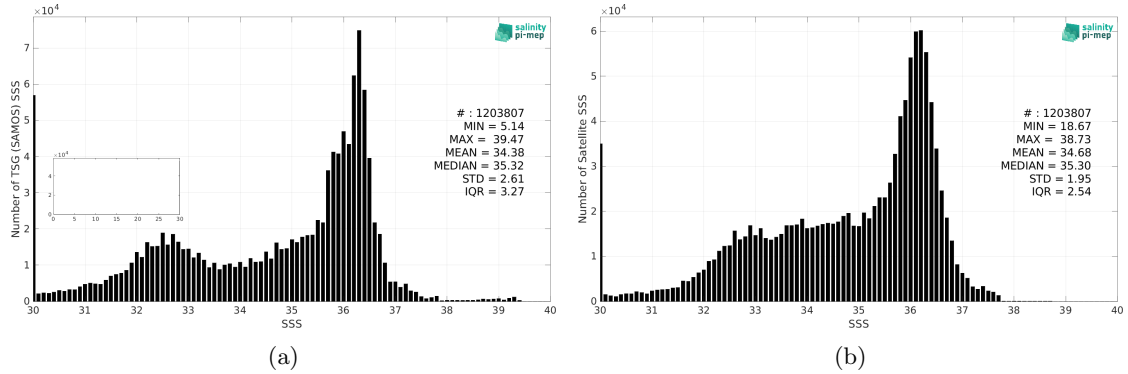
Figure 2: Histograms of SSS from TSG (SAMOS) (a) and SMOS SSS L3 v8 - 18 Days (CATDS-CEC-LOCEAN) (b) considering all match-up pairs per bins of 0.1 over the North Atlantic Ocean Pi-MEP region and for the full satellite product period.
