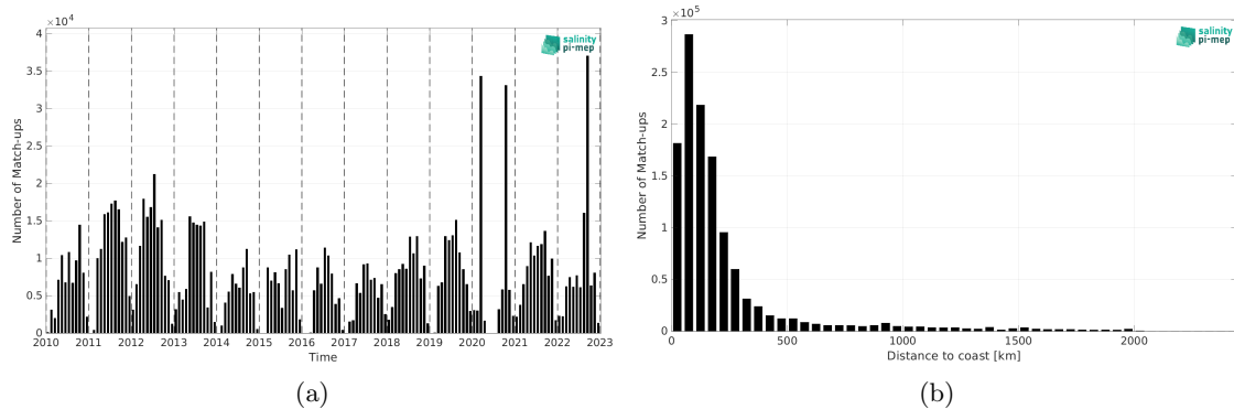
Figure 1: Number of match-ups between TSG (SAMOS) and SMOS SSS L3 v8 - 18 Days (CATDS-CEC-LOCEAN) SSS as a function of time (a) and as function of the distance to coast (b) over the North Atlantic Ocean Pi-MEP region and for the full satellite product period.
