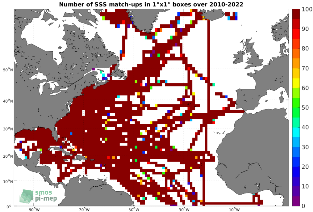
Figure 4: Number of SSS match-ups between TSG (SAMOS) SSS and the SMOS SSS L3 v8 - 18 Days (CATDS-CECOS-LOCEAN) SSS product for the North Atlantic Ocean Pi-MEP region over 1^\circ \times 1^\circ boxes and for the full satellite product period.
