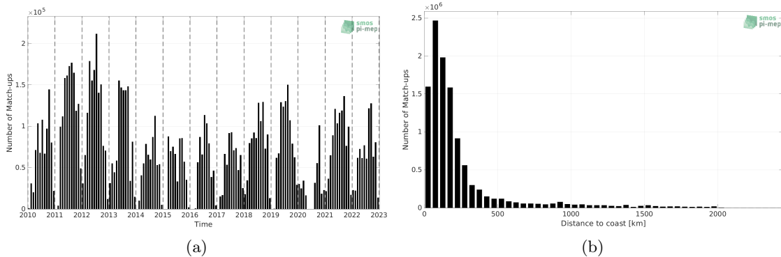
Figure 1: Number of match-ups between TSG (SAMOS) and SMOS SSS L3 v8 - 18 Days (CATDS-CECOS-LOCEAN) SSS as a function of time (a) and as function of the distance to coast (b) over the North Atlantic Ocean Pi-MEP region and for the full satellite product period.
