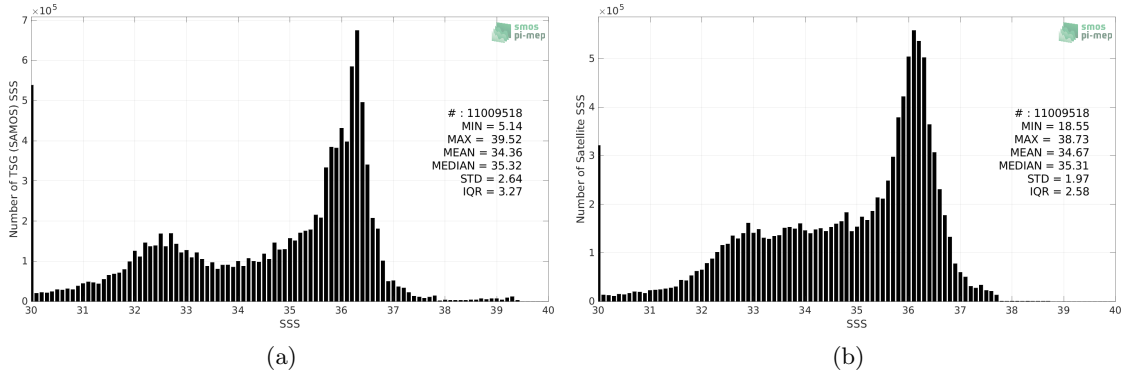
Figure 2: Histograms of SSS from TSG (SAMOS) (a) and SMOS SSS L3 v8 - 18 Days (CATDS-CECOS-LOCEAN) (b) considering all match-up pairs per bins of 0.1 over the North Atlantic Ocean Pi-MEP region and for the full satellite product period.
