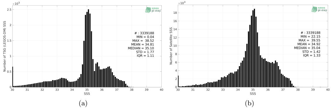
Figure 2: Histograms of SSS from TSG (LEGOS-DM) (a) and SMOS SSS L3 v8 - 18 Days (CATDS-CECOS-LOCEAN) (b) considering all match-up pairs per bins of 0.1 over the North Atlantic Ocean Pi-MEP region and for the full satellite product period.
