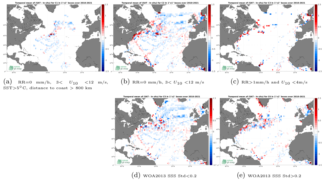
Figure 12: Temporal mean gridded over spatial boxes of size 1^\circ \times 1^\circ of \Delta\text{SSS} (SMOS SSS L3 v8 - 18 Days (CATDS-CECOS-LOCEAN) - TSG (LEGOS-DM)) for 5 different subdatasets corresponding to:RR=0 mm/h, 3 < U_{10} < 12 m/s, SST >5^\circ\text{C} , distance to coast > 800 km (a), RR=0 mm/h, 3 < U_{10} < 12 m/s (b), RR >1 mm/h and U_{10} < 4 m/s (c), WOA2013 SSS Std <0.2 (d), WOA2013 SSS Std >0.2 (e).
