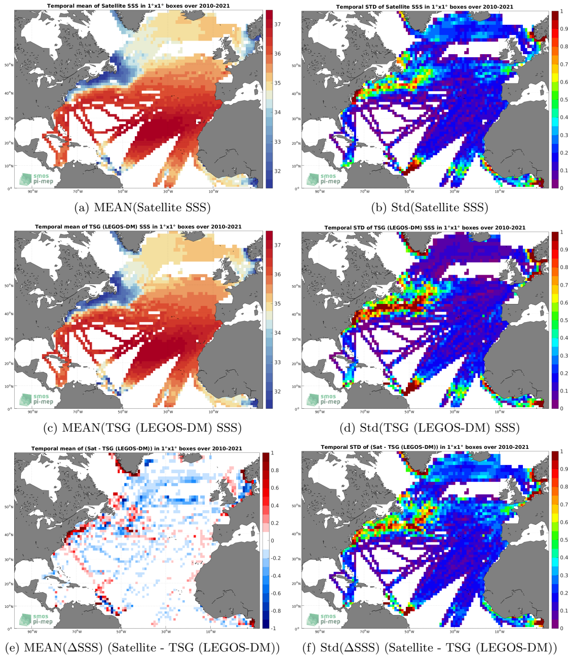
Figure 6: Temporal mean (left) and Std (right) of SSS from SMOS SSS L3 v8 - 18 Days (CATDS-CECOS-LOCEAN) (top), TSG (LEGOS-DM) (middle), and of \Delta SSS (Satellite - TSG (LEGOS-DM)). Only match-up pairs are used to generate these maps.
