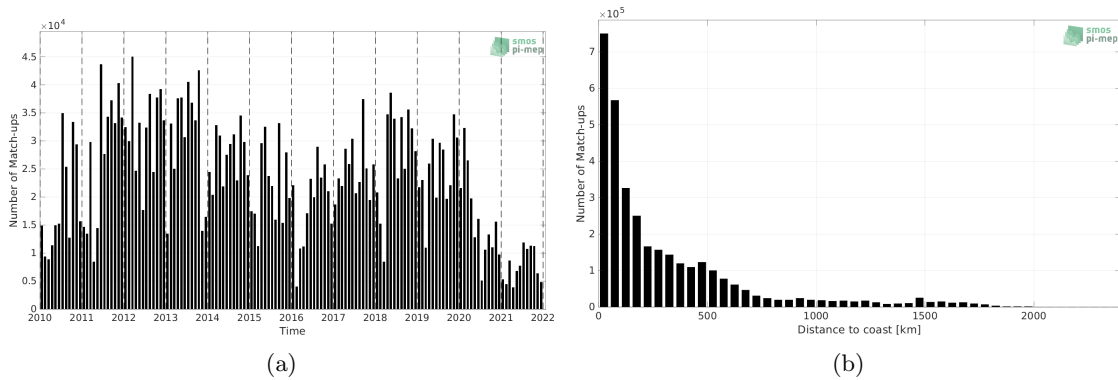
Figure 1: Number of match-ups between TSG (LEGOS-DM) and SMOS SSS L3 v8 - 18 Days (CATDS-CECOS-LOCEAN) SSS as a function of time (a) and as function of the distance to coast (b) over the North Atlantic Ocean Pi-MEP region and for the full satellite product period.
