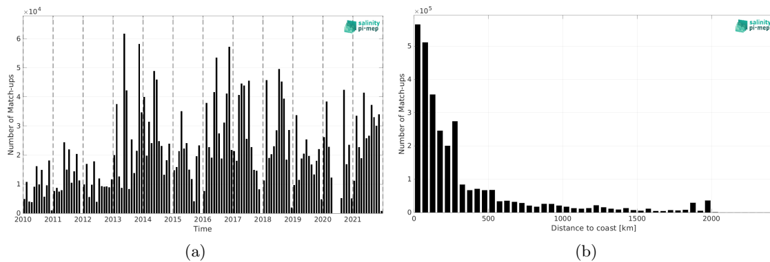
Figure 1: Number of match-ups between TSG (GOSUD-Research-vessel) and SMOS SSS L3 v8 - 18 Days (CATDS-CEC-LOCEAN) SSS as a function of time (a) and as function of the distance to coast (b) over the North Atlantic Ocean Pi-MEP region and for the full satellite product period.
