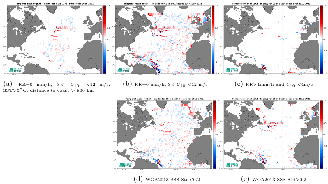
Figure 12: Temporal mean gridded over spatial boxes of size 1^\circ \times 1^\circ of \Delta\text{SSS} (SMOS SSS L3 v8 - 18 Days (CATDS-CEC-LOCEAN) - TSG (GOSUD-Research-vessel)) for 5 different subdatasets corresponding to:RR=0 mm/h, 3 < U_{10} < 12 m/s, SST >5^\circ\text{C} , distance to coast > 800 km (a), RR=0 mm/h, 3 < U_{10} < 12 m/s (b), RR >1 mm/h and U_{10} < 4 m/s (c), WOA2013 SSS Std <0.2 (d), WOA2013 SSS Std >0.2 (e).
