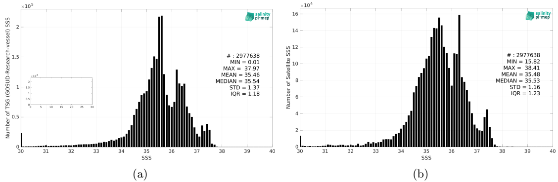
Figure 2: Histograms of SSS from TSG (GOSUD-Research-vessel) (a) and SMOS SSS L3 v8 - 18 Days (CATDS-CEC-LOCEAN) (b) considering all match-up pairs per bins of 0.1 over the North Atlantic Ocean Pi-MEP region and for the full satellite product period.
