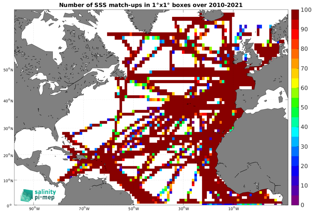
Figure 4: Number of SSS match-ups between TSG (GOSUD-Research-vessel) SSS and the SMOS SSS L3 v8 - 18 Days (CATDS-CEC-LOCEAN) SSS product for the North Atlantic Ocean Pi-MEP region over 1^\circ \times 1^\circ boxes and for the full satellite product period.
