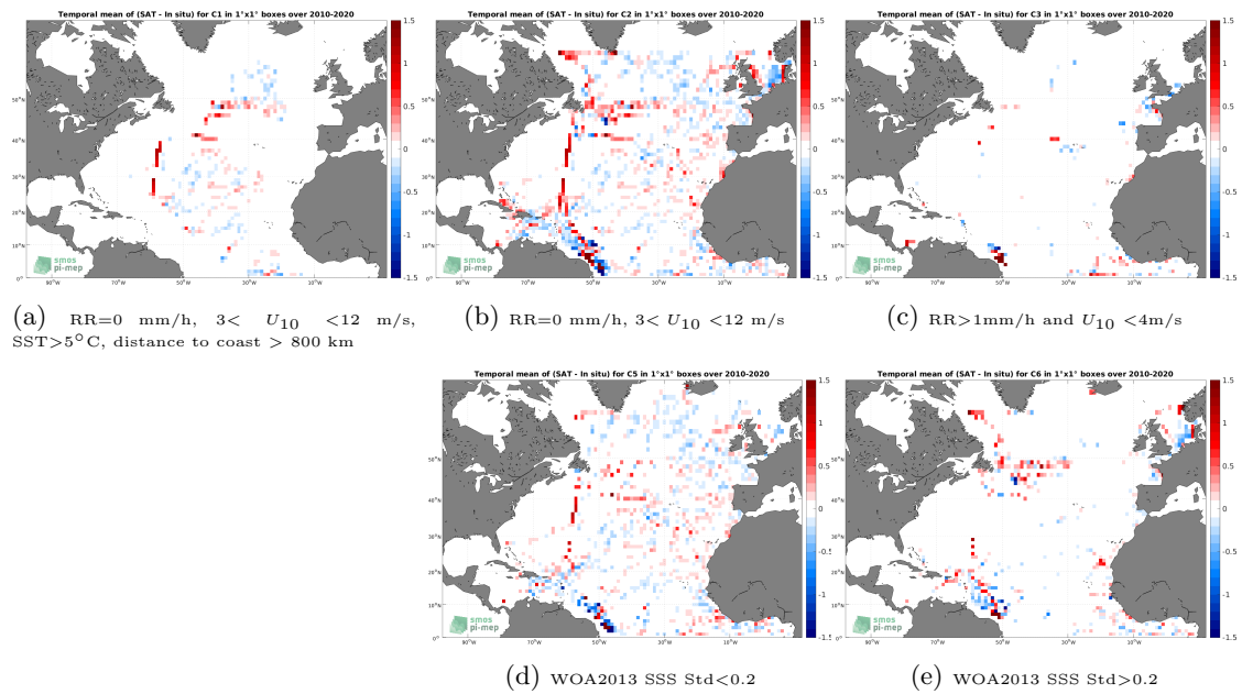
Figure 12: Temporal mean gridded over spatial boxes of size 1^\circ \times 1^\circ of \Delta\text{SSS} (SMOS SSS L3 v8 - 18 Days (CATDS-CECOS-LOCEAN) - TSG (GOSUD-Research-vessel)) for 5 different sub-datasets corresponding to:RR=0 mm/h, 3 < U_{10} < 12 m/s, SST>5°C, distance to coast > 800 km (a), RR=0 mm/h, 3 < U_{10} < 12 m/s (b), RR>1mm/h and U_{10} < 4 m/s (c), WOA2013 SSS Std<0.2 (d), WOA2013 SSS Std>0.2 (e).
