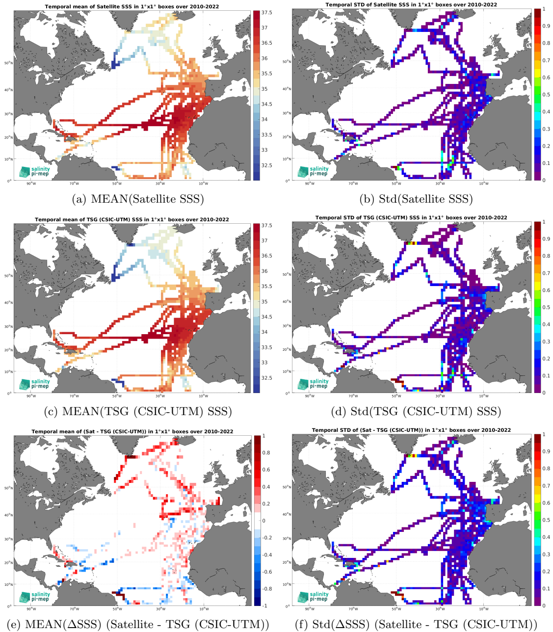
Figure 6: Temporal mean (left) and Std (right) of SSS from SMOS SSS L3 v8 - 18 Days (CATDS-CEC-LOCEAN) (top), TSG (CSIC-UTM) (middle), and of \Delta SSS (Satellite - TSG (CSIC-UTM)). Only match-up pairs are used to generate these maps.
