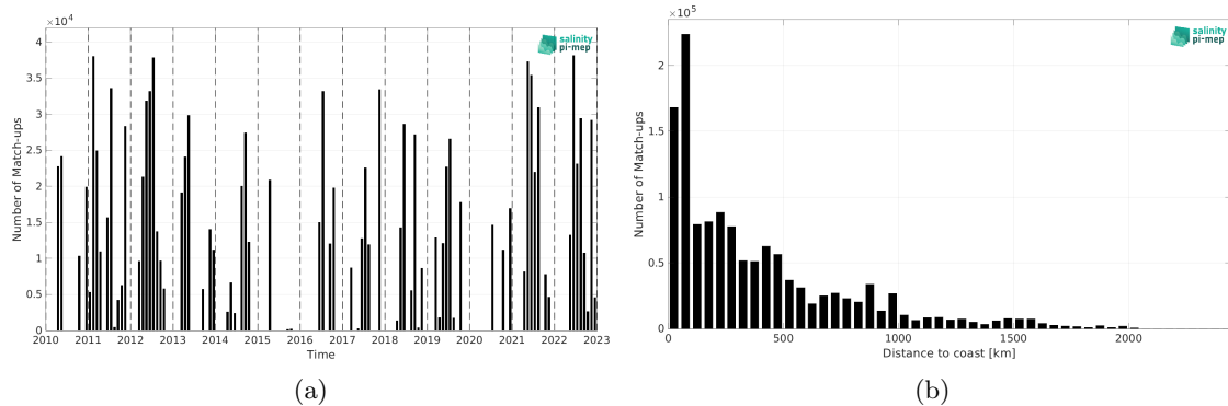
Figure 1: Number of match-ups between TSG (CSIC-UTM) and SMOS SSS L3 v8 - 18 Days (CATDS-CEC-LOCEAN) SSS as a function of time (a) and as function of the distance to coast (b) over the North Atlantic Ocean Pi-MEP region and for the full satellite product period.
