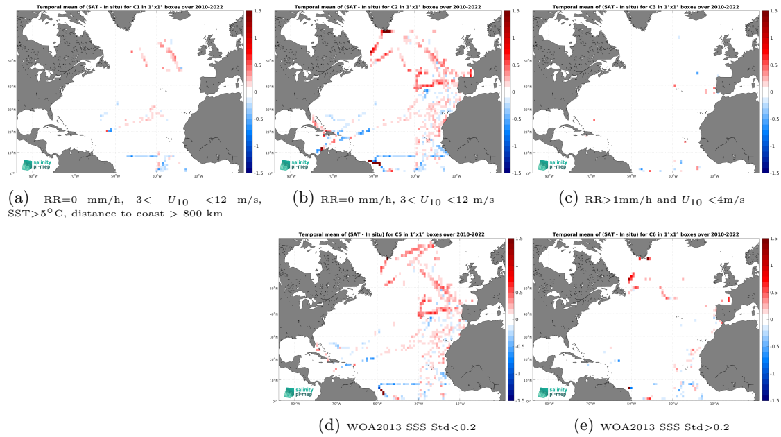
Figure 12: Temporal mean gridded over spatial boxes of size 1^\circ \times 1^\circ of \Delta\text{SSS} (SMOS SSS L3 v8 - 18 Days (CATDS-CEC-LOCEAN) - TSG (CSIC-UTM)) for 5 different subdatasets corresponding to:RR=0 mm/h, 3 < U_{10} < 12 m/s, SST >5^\circ\text{C} , distance to coast > 800 km (a), RR=0 mm/h, 3 < U_{10} < 12 m/s (b), RR >1 mm/h and U_{10} < 4 m/s (c), WOA2013 SSS Std <0.2 (d), WOA2013 SSS Std >0.2 (e).
