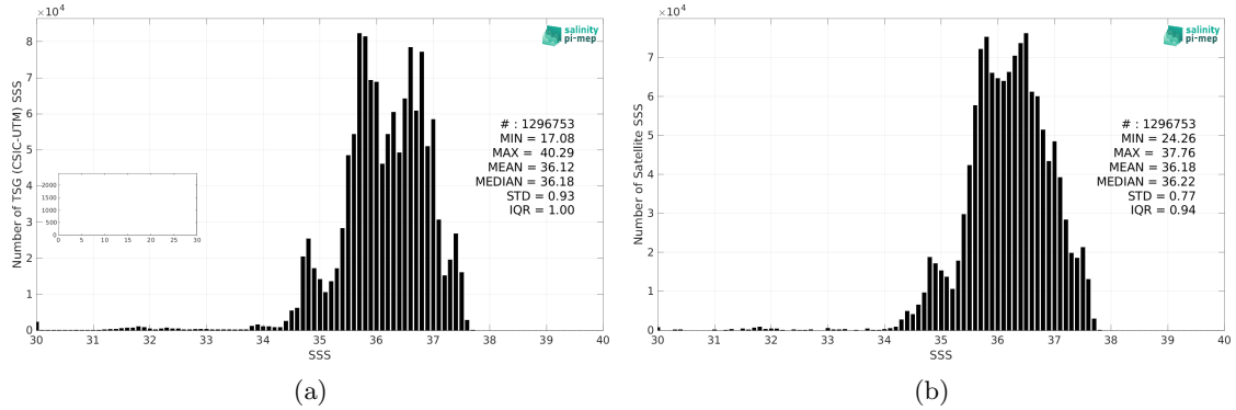
Figure 2: Histograms of SSS from TSG (CSIC-UTM) (a) and SMOS SSS L3 v8 - 18 Days (CATDS-CEC-LOCEAN) (b) considering all match-up pairs per bins of 0.1 over the North Atlantic Ocean Pi-MEP region and for the full satellite product period.
