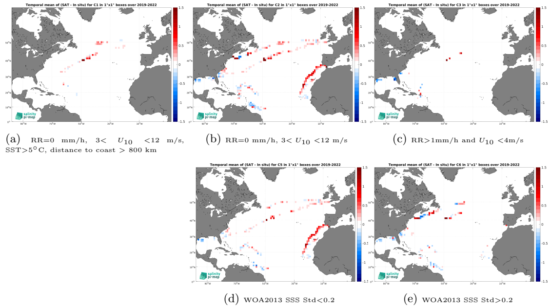
Figure 12: Temporal mean gridded over spatial boxes of size 1^\circ \times 1^\circ of \Delta\text{SSS} (SMOS SSS L3 v8 - 18 Days (CATDS-CEC-LOCEAN) - Saildrone) for 5 different subdatasets corresponding to:RR=0 mm/h, 3 < U_{10} < 12 m/s, SST >5^\circ\text{C} , distance to coast > 800 km (a), RR=0 mm/h, 3 < U_{10} < 12 m/s (b), RR >1 mm/h and U_{10} < 4 m/s (c), WOA2013 SSS Std <0.2 (d), WOA2013 SSS Std >0.2 (e).
