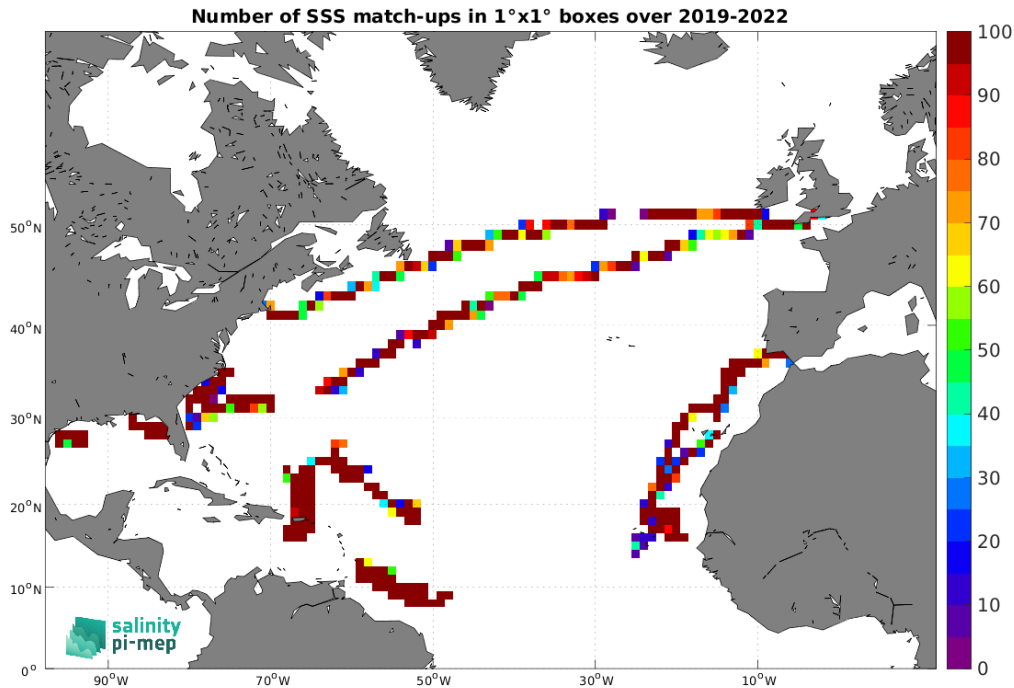
Figure 4: Number of SSS match-ups between Saildrone SSS and the SMOS SSS L3 v8 - 18 Days (CATDS-CEC-LOCEAN) SSS product for the North Atlantic Ocean Pi-MEP region over 1^\circ \times 1^\circ boxes and for the full satellite product period.
