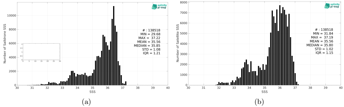
Figure 2: Histograms of SSS from Saildrone (a) and SMOS SSS L3 v8 - 18 Days (CATDS-CEC-LOCEAN) (b) considering all match-up pairs per bins of 0.1 over the North Atlantic Ocean Pi-MEP region and for the full satellite product period.
