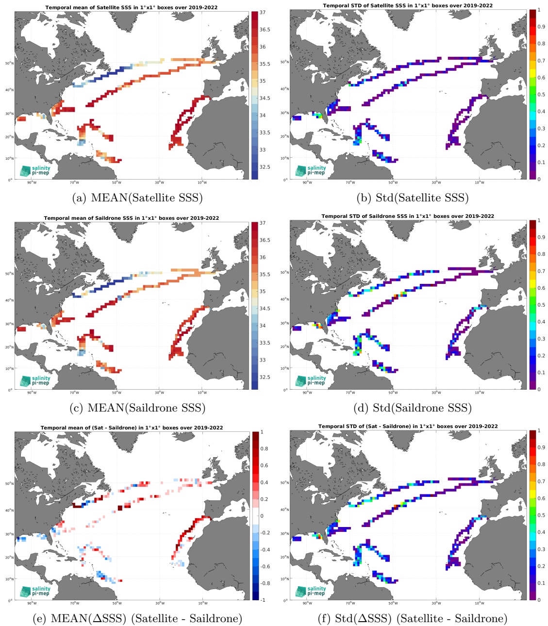
Figure 6: Temporal mean (left) and Std (right) of SSS from SMOS SSS L3 v8 - 18 Days (CATDS-CEC-LOCEAN) (top), Saildrone (middle), and of \Delta SSS (Satellite - Saildrone). Only match-up pairs are used to generate these maps.
