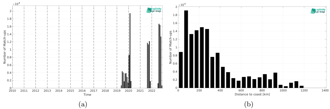
Figure 1: Number of match-ups between Saildrone and SMOS SSS L3 v8 - 18 Days (CATDS-CEC-LOCEAN) SSS as a function of time (a) and as function of the distance to coast (b) over the North Atlantic Ocean Pi-MEP region and for the full satellite product period.
