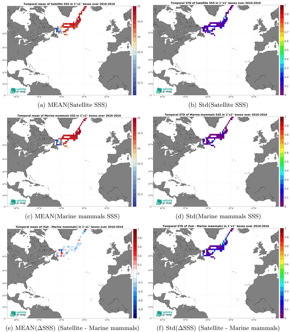
Figure 6: Temporal mean (left) and Std (right) of SSS from SMOS SSS L3 v8 - 18 Days (CATDS-CEC-LOCEAN) (top), Marine mammals (middle), and of \Delta SSS (Satellite - Marine mammals). Only match-up pairs are used to generate these maps.
