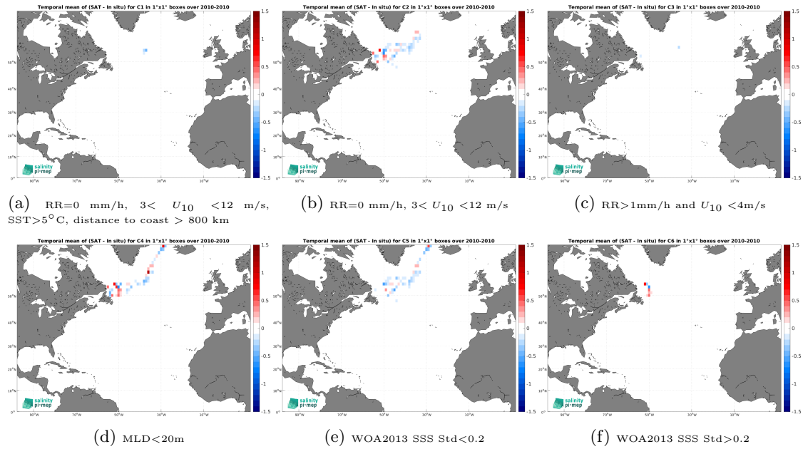
Figure 12: Temporal mean gridded over spatial boxes of size 1^{\circ}\times 1^{\circ} of \Delta\text{SSS} (SMOS SSS L3 v8 - 18 Days (CATDS-CEC-LOCEAN) - Marine mammals) for 6 different subdatasets corresponding to:RR=0 mm/h, 3 < U_{10} < 12 m/s, SST >5^{\circ}\text{C} , distance to coast > 800 km (a), RR=0 mm/h, 3 < U_{10} < 12 m/s (b), RR >1\text{mm/h} and U_{10} < 4\text{m/s} (c),MLD <20\text{m} (d),WOA2013 SSS Std <0.2 (e),WOA2013 SSS Std >0.2 (f).
