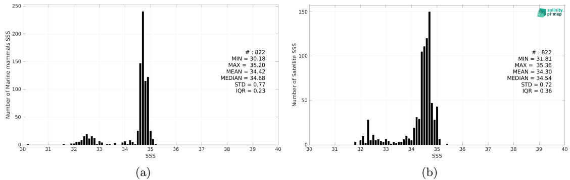
Figure 2: Histograms of SSS from Marine mammals (a) and SMOS SSS L3 v8 - 18 Days (CATDS-CEC-LOCEAN) (b) considering all match-up pairs per bins of 0.1 over the North Atlantic Ocean Pi-MEP region and for the full satellite product period.
