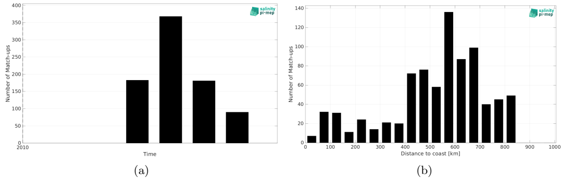
Figure 1: Number of match-ups between Marine mammals and SMOS SSS L3 v8 - 18 Days (CATDS-CEC-LOCEAN) SSS as a function of time (a) and as function of the distance to coast (b) over the North Atlantic Ocean Pi-MEP region and for the full satellite product period.
