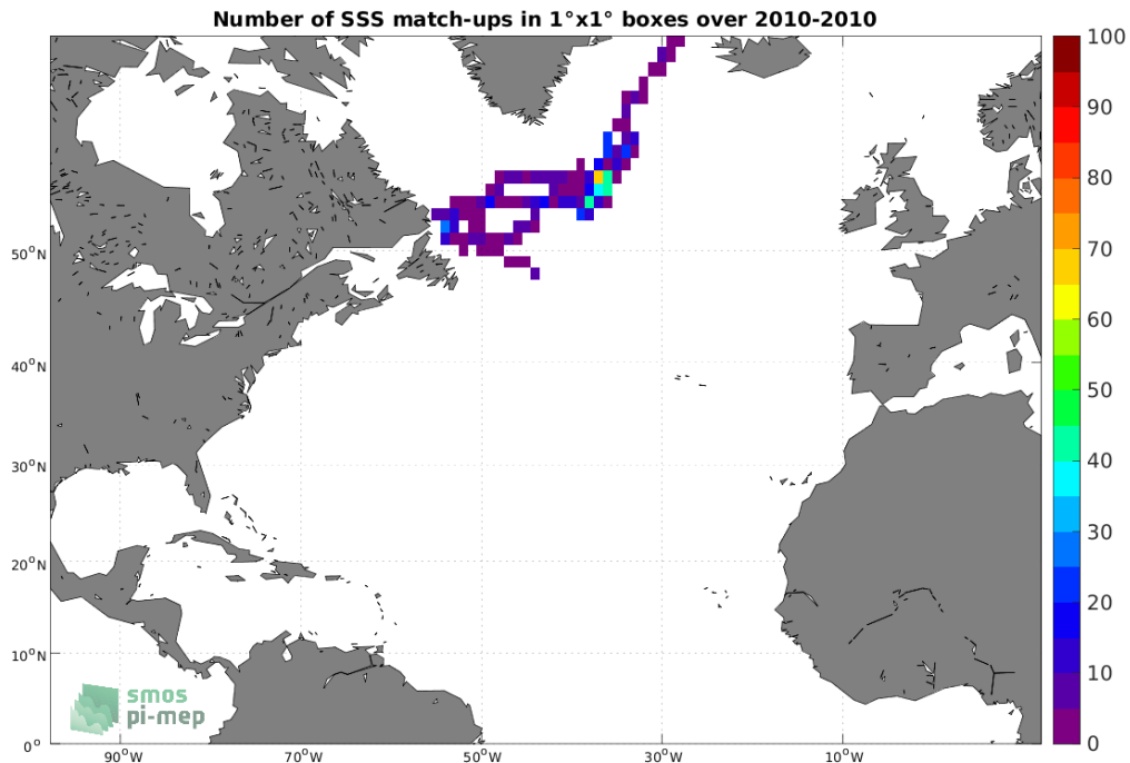
Figure 4: Number of SSS match-ups between Marine mammals SSS and the SMOS SSS L3 v8 - 18 Days (CATDS-CECOS-LOCEAN) SSS product for the North Atlantic Ocean Pi-MEP region over 1^\circ \times 1^\circ boxes and for the full satellite product period.
