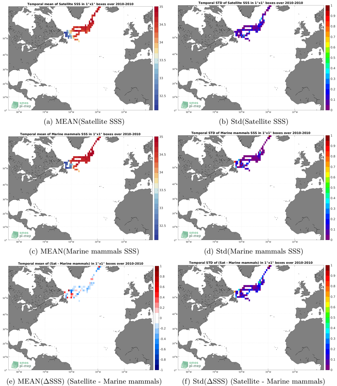
Figure 6: Temporal mean (left) and Std (right) of SSS from SMOS SSS L3 v8 - 18 Days (CATDS-CECOS-LOCEAN) (top), Marine mammals (middle), and of \Delta SSS (Satellite - Marine mammals). Only match-up pairs are used to generate these maps.
