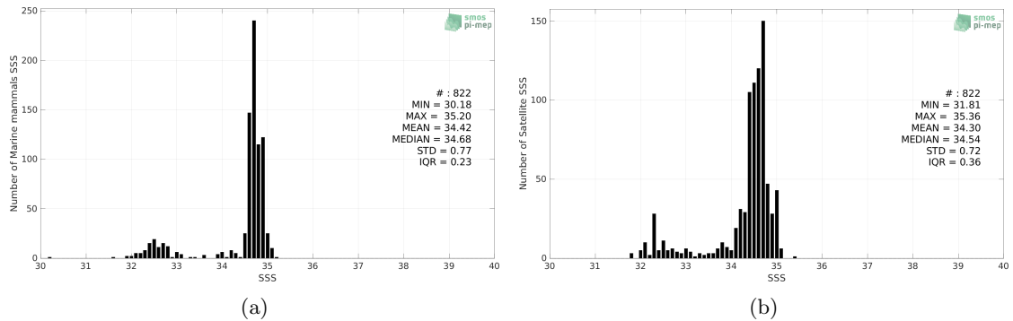
Figure 2: Histograms of SSS from Marine mammals (a) and SMOS SSS L3 v8 - 18 Days (CATDS-CECOS-LOCEAN) (b) considering all match-up pairs per bins of 0.1 over the North Atlantic Ocean Pi-MEP region and for the full satellite product period.
