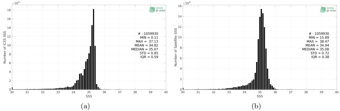
Figure 2: Histograms of SSS from ICES (a) and SMOS SSS L3 v8 - 18 Days (CATDS-CECOS-LOCEAN) (b) considering all match-up pairs per bins of 0.1 over the North Atlantic Ocean Pi-MEP region and for the full satellite product period.
