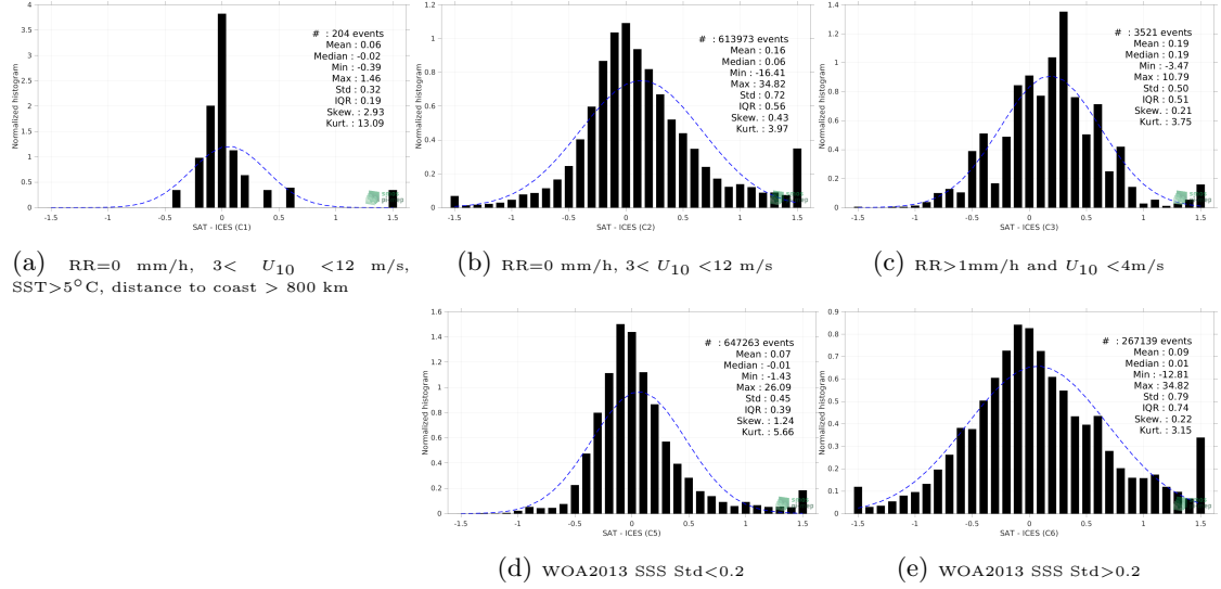
Figure 13: Normalized histogram of \Delta SSS (SMOS SSS L3 v8 - 18 Days (CATDS-CECOS-LOCEAN) - ICES) for 5 different subdatasets corresponding to: RR=0 mm/h, 3 < U_{10} < 12 m/s, SST > 5°C, distance to coast > 800 km (a), RR=0 mm/h, 3 < U_{10} < 12 m/s (b), RR > 1mm/h and U_{10} < 4 m/s (c), WOA2013 SSS Std < 0.2 (d), WOA2013 SSS Std > 0.2 (e).
