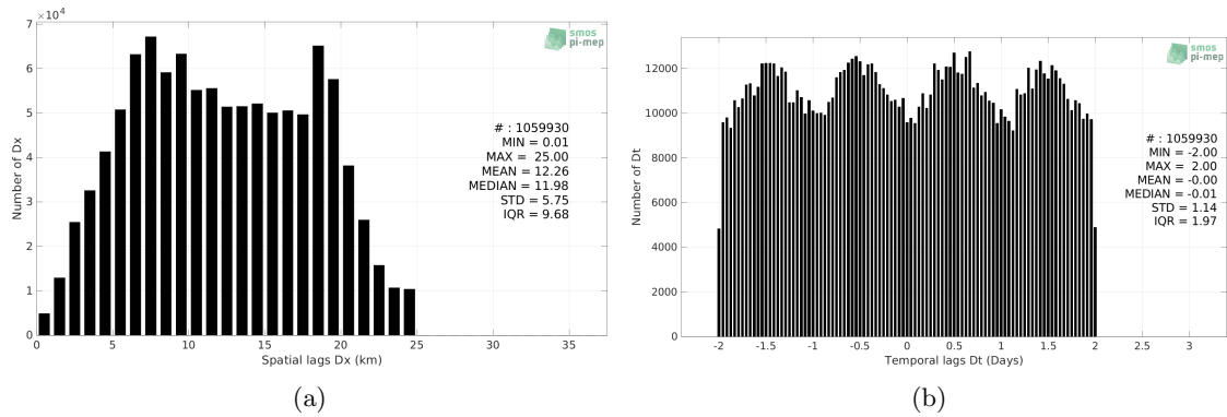
Figure 5: Histograms of the spatial (a) and temporal (b) lags between the location/time of the ICES measurement and the date of the corresponding SMOS SSS L3 v8 - 18 Days (CATDS-CECOS-LOCEAN) SSS pixel.
