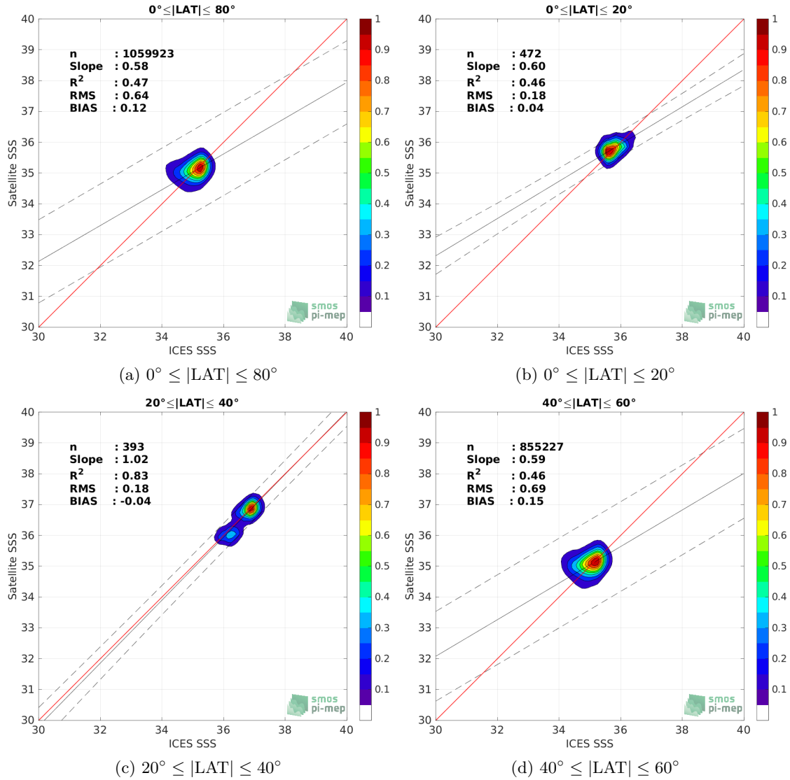
Figure 9: Contour maps of the concentration of SMOS SSS L3 v8 - 18 Days (CATDS-CECOS-LOCEAN) SSS (y-axis) versus ICES SSS (x-axis) at match-up pairs for different latitude bands. For each plot, the red line shows x=y . The black thin and dashed lines indicate a linear fit through the data cloud and the \pm 95\% confidence levels, respectively. The number match-up pairs n , the slope and R^2 coefficient of the linear fit, the root mean square (RMS) and the mean bias between satellite and in situ data are indicated for each latitude band in each plots.
