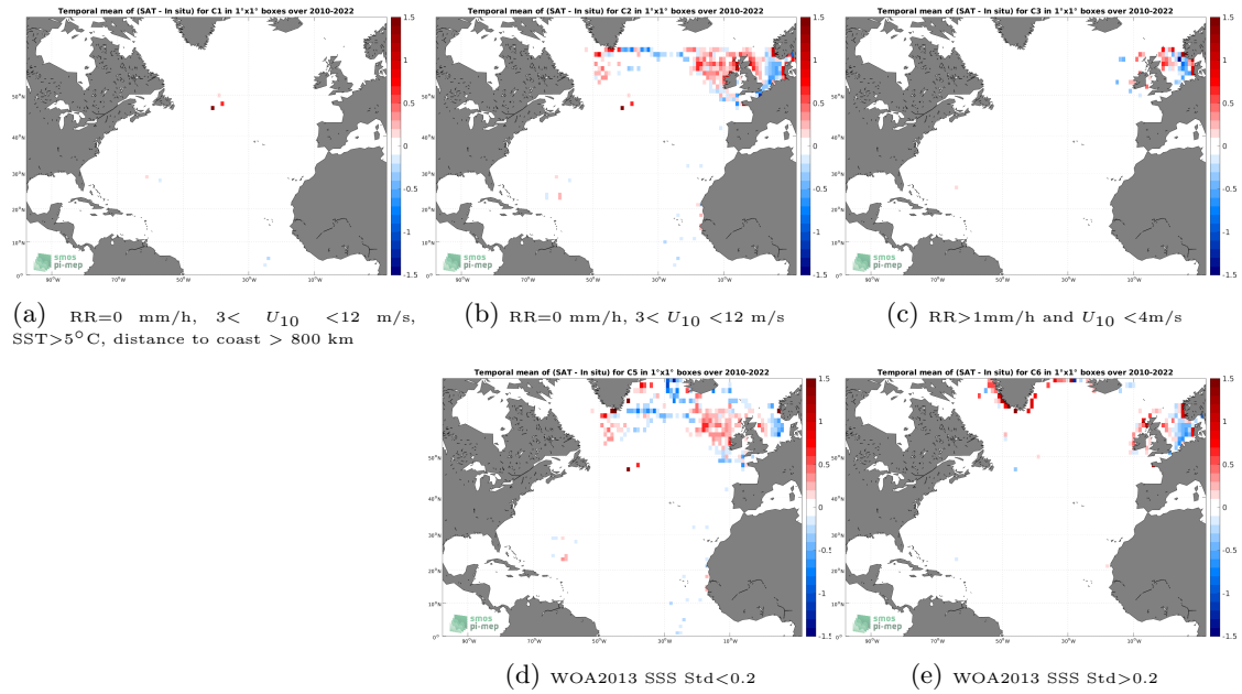
Figure 12: Temporal mean gridded over spatial boxes of size 1^\circ \times 1^\circ of \Delta\text{SSS} (SMOS SSS L3 v8 - 18 Days (CATDS-CECOS-LOCEAN) - ICES) for 5 different subdatasets corresponding to:RR=0 mm/h, 3 < U_{10} < 12 m/s, SST >5^\circ\text{C} , distance to coast > 800 km (a), RR=0 mm/h, 3 < U_{10} < 12 m/s (b), RR >1 mm/h and U_{10} < 4 m/s (c), WOA2013 SSS Std <0.2 (d), WOA2013 SSS Std >0.2 (e).
