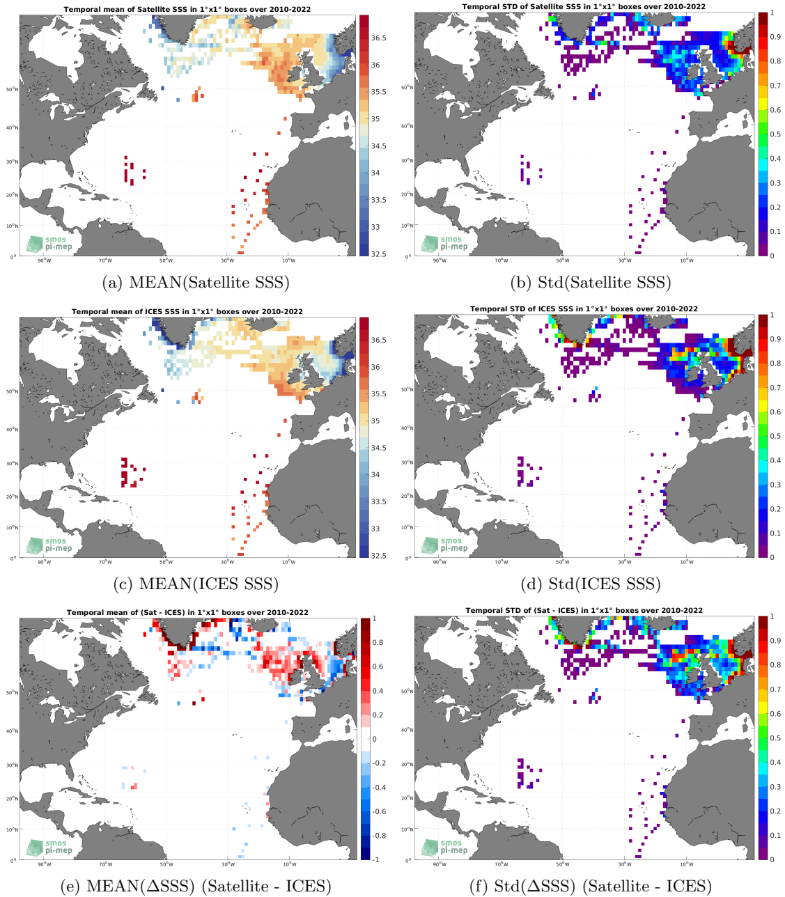
Figure 6: Temporal mean (left) and Std (right) of SSS from SMOS SSS L3 v8 - 18 Days (CATDS-CECOS-LOCEAN) (top), ICES (middle), and of \Delta SSS (Satellite - ICES). Only match-up pairs are used to generate these maps.
