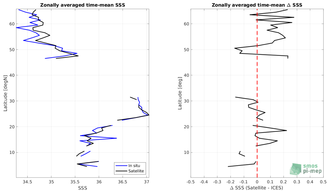
Figure 8: Left panel: Zonal mean SSS from SMOS SSS L3 v8 - 18 Days (CATDS-CECOS-LOCEAN) satellite product (black) and from ICES (blue). Right panel: Zonal mean of \Delta SSS (Satellite - ICES) for all the collected Pi-MEP match-up pairs estimated over the full satellite product period.
