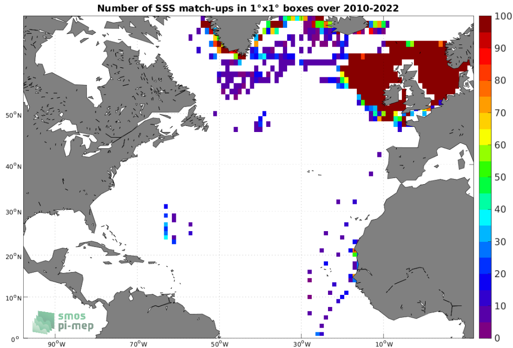
Figure 4: Number of SSS match-ups between ICES SSS and the SMOS SSS L3 v8 - 18 Days (CATDS-CECOS-LOCEAN) SSS product for the North Atlantic Ocean Pi-MEP region over 1^\circ \times 1^\circ boxes and for the full satellite product period.
