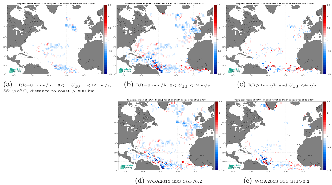
Figure 11: Temporal mean gridded over spatial boxes of size 1^\circ \times 1^\circ of \Delta\text{SSS} (SMOS SSS L3 v8 - 18 Days (CATDS-CEC-LOCEAN) - Surface drifters) for 5 different subdatasets corresponding to:RR=0 mm/h, 3 < U_{10} < 12 m/s, SST >5^\circ\text{C} , distance to coast > 800 km (a), RR=0 mm/h, 3 < U_{10} < 12 m/s (b), RR >1 mm/h and U_{10} < 4 m/s (c), WOA2013 SSS Std <0.2 (d), WOA2013 SSS Std >0.2 (e).
