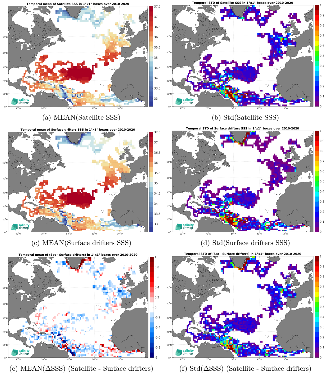
Figure 5: Temporal mean (left) and Std (right) of SSS from SMOS SSS L3 v8 - 18 Days (CATDS-CEC-LOCEAN) (top), Surface drifters (middle), and of \Delta SSS (Satellite - Surface drifters). Only match-up pairs are used to generate these maps.
