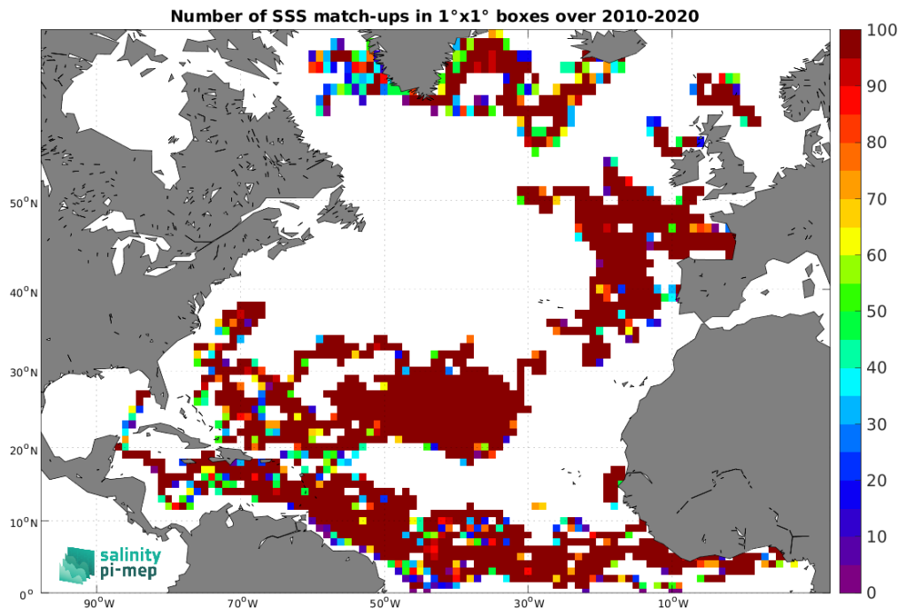
Figure 3: Number of SSS match-ups between Surface drifters SSS and the SMOS SSS L3 v8 - 18 Days (CATDS-CEC-LOCEAN) SSS product for the North Atlantic Ocean Pi-MEP region over 1^\circ \times 1^\circ boxes and for the full satellite product period.
