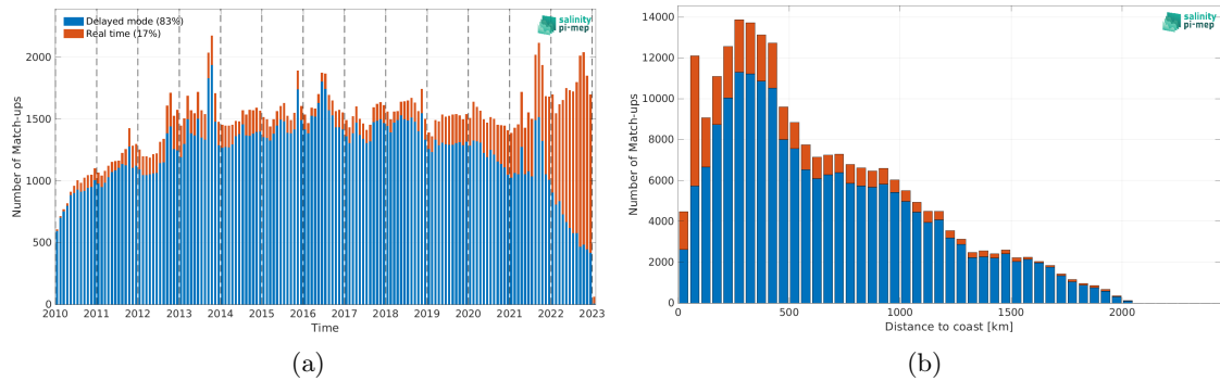
Figure 1: Number of match-ups between Argo and SMOS SSS L3 v8 - 18 Days (CATDS-CEC-LOCEAN) SSS as a function of time (a) and as function of the distance to coast (b) over the North Atlantic Ocean Pi-MEP region and for the full satellite product period.
