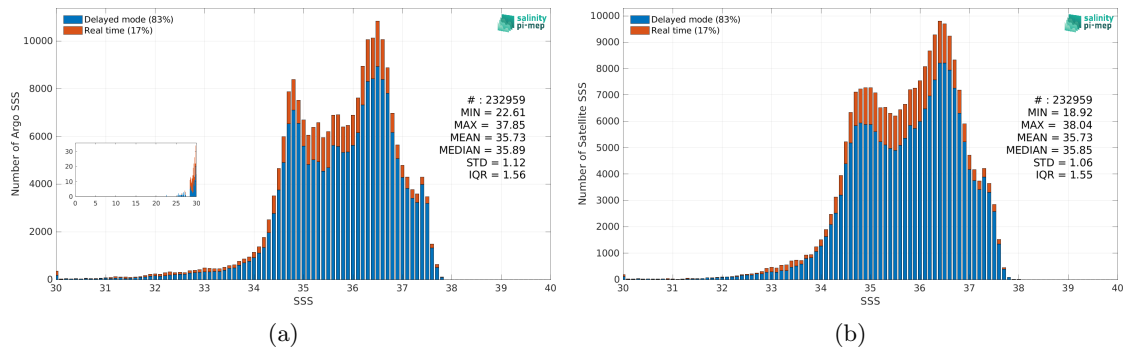
Figure 2: Histograms of SSS from Argo (a) and SMOS SSS L3 v8 - 18 Days (CATDS-CEC-LOCEAN) (b) considering all match-up pairs per bins of 0.1 over the North Atlantic Ocean Pi-MEP region and for the full satellite product period.
