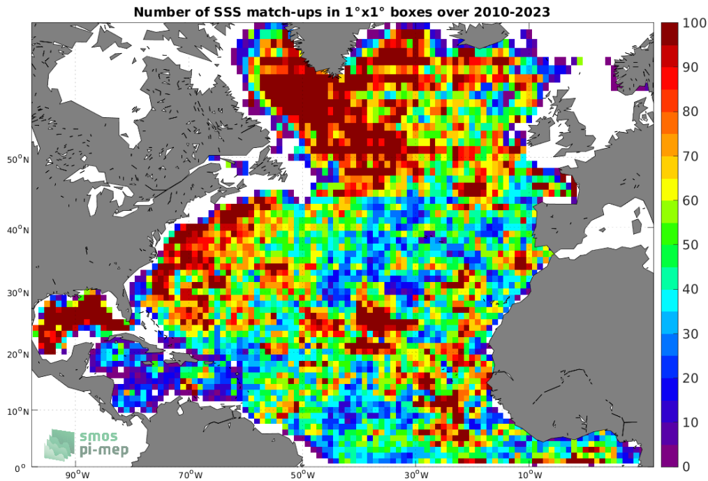
Figure 4: Number of SSS match-ups between Argo SSS and the SMOS SSS L3 v8 - 18 Days (CATDS-CECOS-LOCEAN) SSS product for the North Atlantic Ocean Pi-MEP region over 1^\circ \times 1^\circ boxes and for the full satellite product period.
