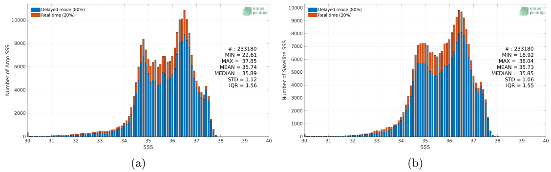
Figure 2: Histograms of SSS from Argo (a) and SMOS SSS L3 v8 - 18 Days (CATDS-CECOS-LOCEAN) (b) considering all match-up pairs per bins of 0.1 over the North Atlantic Ocean Pi-MEP region and for the full satellite product period.
