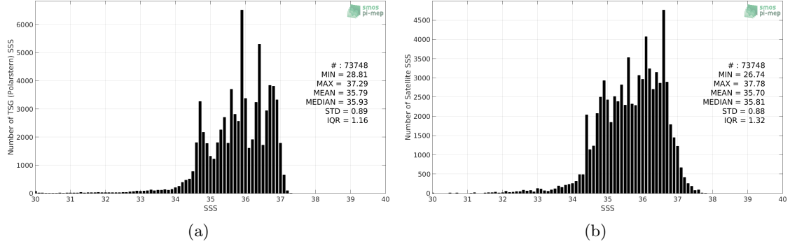
Figure 2: Histograms of SSS from TSG (Polarstern) (a) and SMOS SSS L3 v7 - 9 Days (CATDS-CECOS-LOCEAN) (b) considering all match-up pairs per bins of 0.1 over the North Atlantic Ocean Pi-MEP region and for the full satellite product period.
