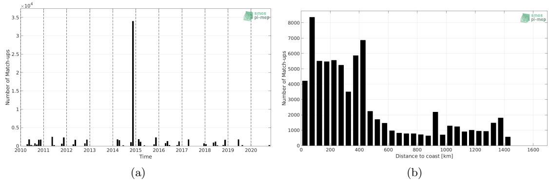
Figure 1: Number of match-ups between TSG (Polarstern) and SMOS SSS L3 v7 - 9 Days (CATDS-CECOS-LOCEAN) SSS as a function of time (a) and as function of the distance to coast (b) over the North Atlantic Ocean Pi-MEP region and for the full satellite product period.
