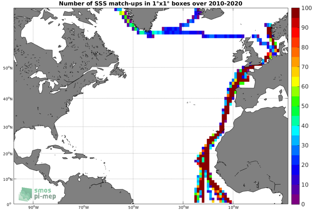
Figure 4: Number of SSS match-ups between TSG (Polarstern) SSS and the SMOS SSS L3 v7 - 9 Days (CATDS-CECOS-LOCEAN) SSS product for the North Atlantic Ocean Pi-MEP region over 1^\circ \times 1^\circ boxes and for the full satellite product period.
