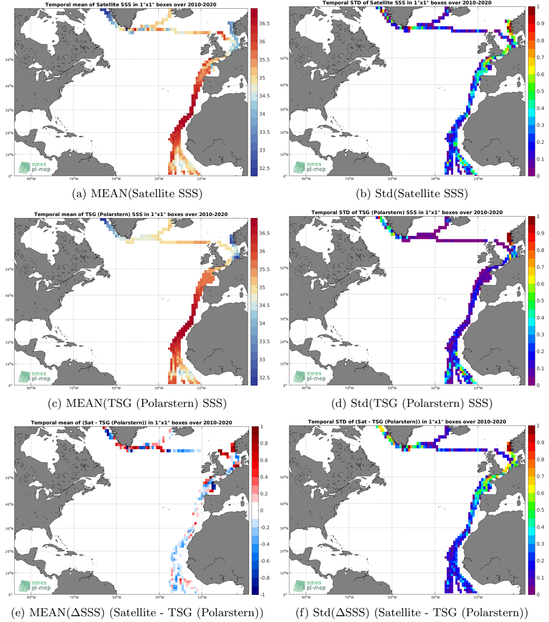
Figure 6: Temporal mean (left) and Std (right) of SSS from SMOS SSS L3 v7 - 9 Days (CATDS-CECOS-LOCEAN) (top), TSG (Polarstern) (middle), and of \Delta SSS (Satellite - TSG (Polarstern)). Only match-up pairs are used to generate these maps.
