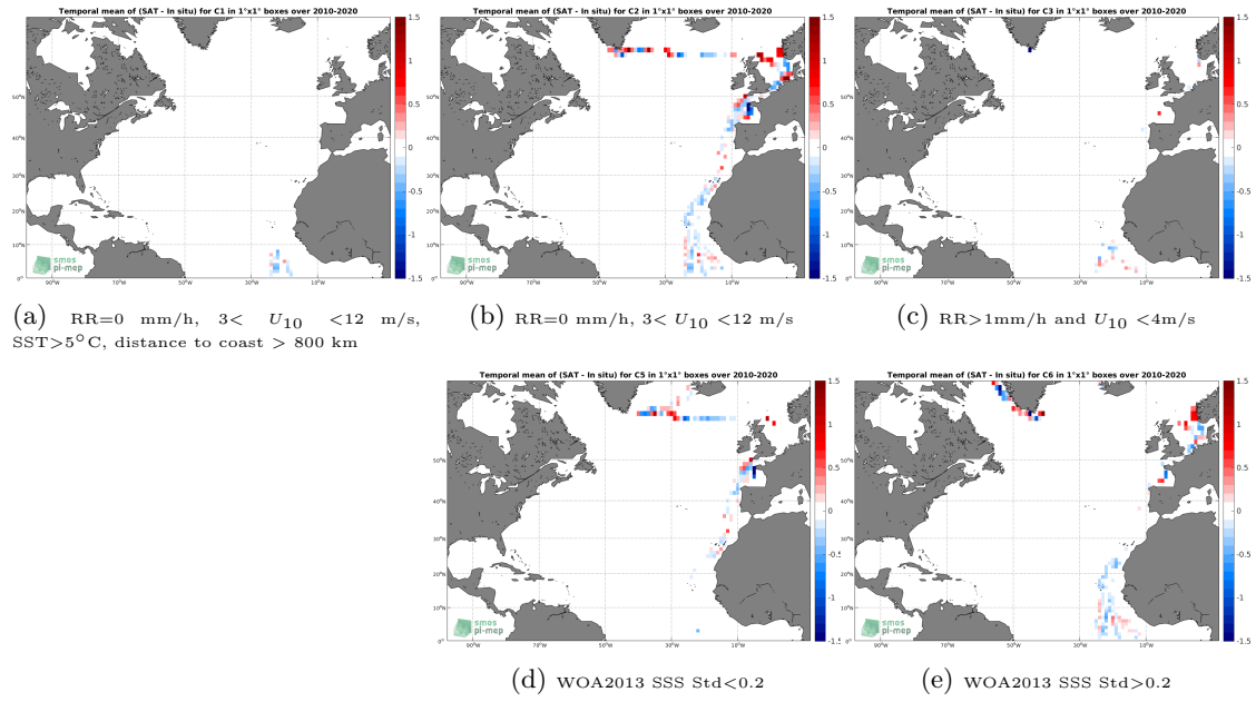
Figure 12: Temporal mean gridded over spatial boxes of size 1^\circ \times 1^\circ of \Delta SSS (SMOS SSS L3 v7 - 9 Days (CATDS-CECOS-LOCEAN) - TSG (Polarstern)) for 5 different subdatasets corresponding to: RR=0 mm/h, 3 < U_{10} < 12 m/s, SST >5^\circ\text{C} , distance to coast > 800 km (a), RR=0 mm/h, 3 < U_{10} < 12 m/s (b), RR >1 mm/h and U_{10} < 4 m/s (c), WOA2013 SSS Std <0.2 (d), WOA2013 SSS Std >0.2 (e).
