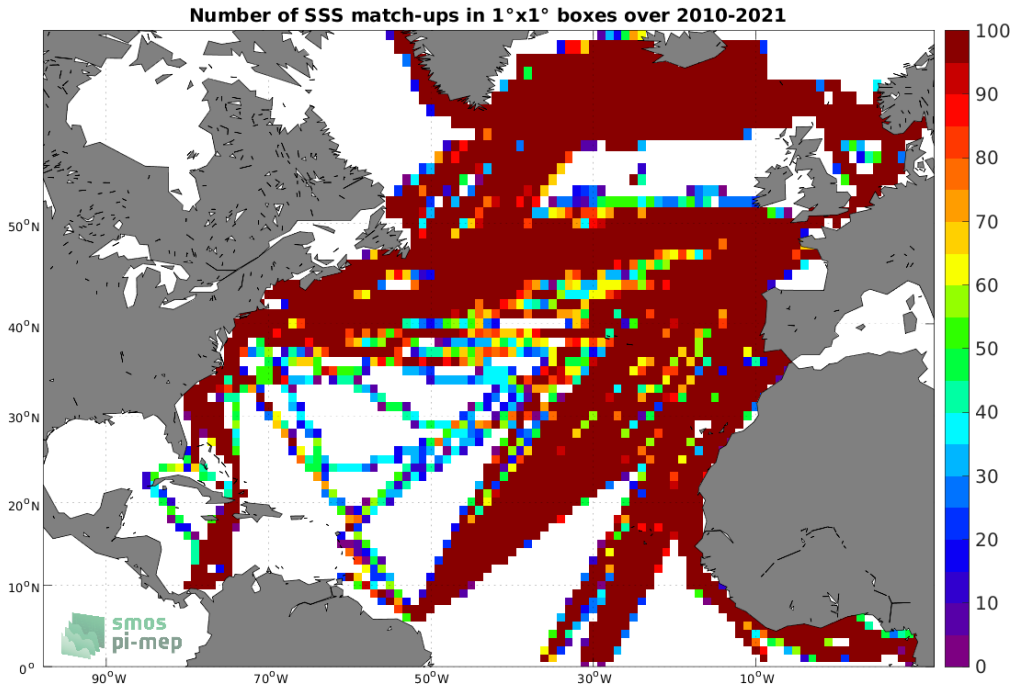
Figure 4: Number of SSS match-ups between TSG (LEGOS-DM) SSS and the SMOS SSS L3 v7 - 9 Days (CATDS-CECOS-LOCEAN) SSS product for the North Atlantic Ocean Pi-MEP region over 1°x1° boxes and for the full satellite product period.
