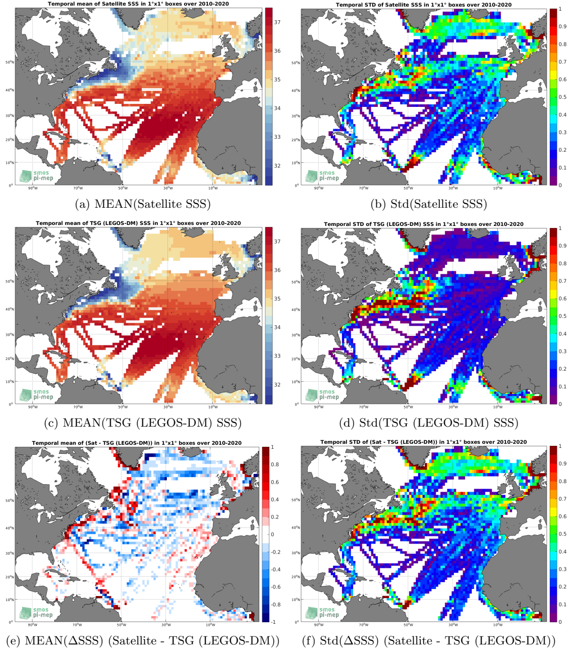
Figure 6: Temporal mean (left) and Std (right) of SSS from SMOS SSS L3 v7 - 9 Days (CATDS-CECOS-LOCEAN) (top), TSG (LEGOS-DM) (middle), and of \Delta SSS (Satellite - TSG (LEGOS-DM)). Only match-up pairs are used to generate these maps.
