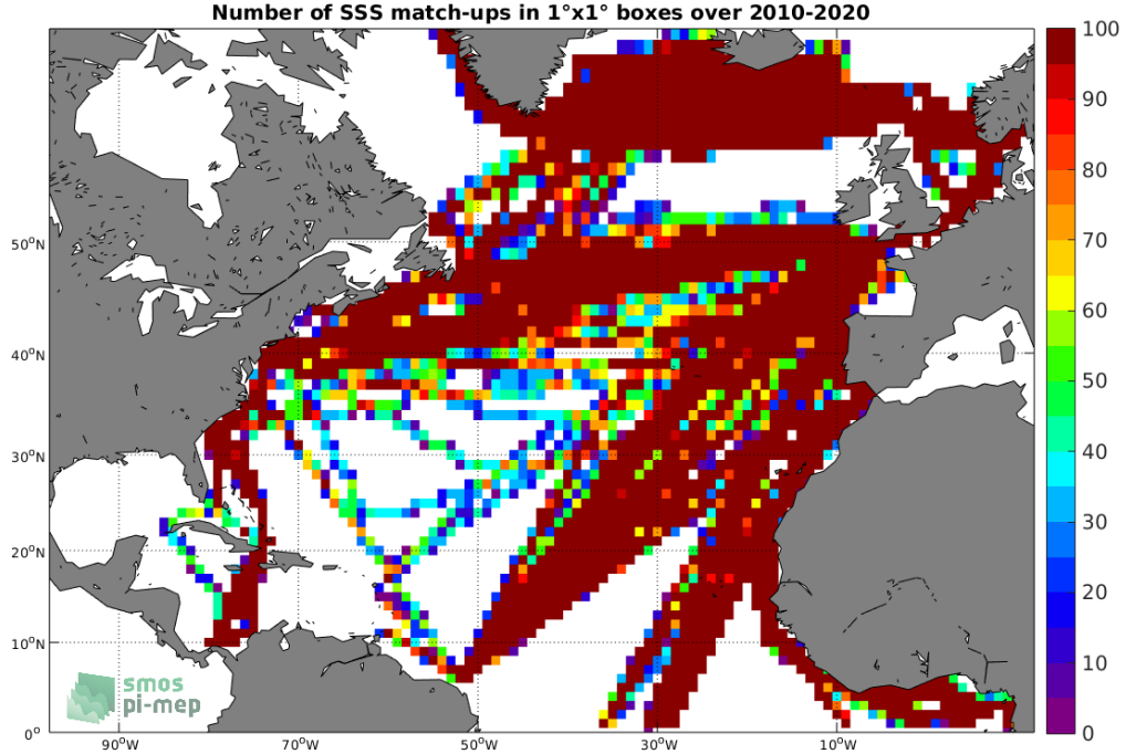
Figure 4: Number of SSS match-ups between TSG (LEGOS-DM) SSS and the SMOS SSS L3 v7 - 9 Days (CATDS-CECOS-LOCEAN) SSS product for the North Atlantic Ocean Pi-MEP region over 1^\circ \times 1^\circ boxes and for the full satellite product period.
