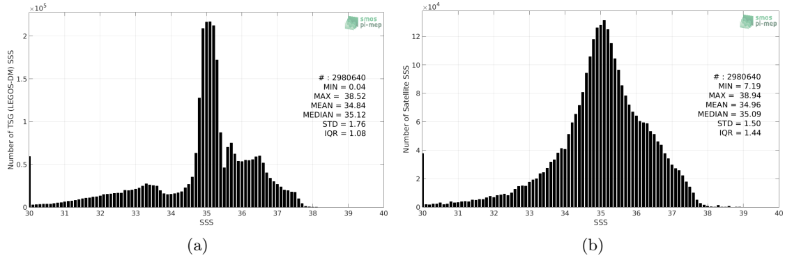
Figure 2: Histograms of SSS from TSG (LEGOS-DM) (a) and SMOS SSS L3 v7 - 9 Days (CATDS-CECOS-LOCEAN) (b) considering all match-up pairs per bins of 0.1 over the North Atlantic Ocean Pi-MEP region and for the full satellite product period.
