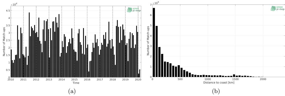
Figure 1: Number of match-ups between TSG (LEGOS-DM) and SMOS SSS L3 v7 - 9 Days (CATDS-CECOS-LOCEAN) SSS as a function of time (a) and as function of the distance to coast (b) over the North Atlantic Ocean Pi-MEP region and for the full satellite product period.
