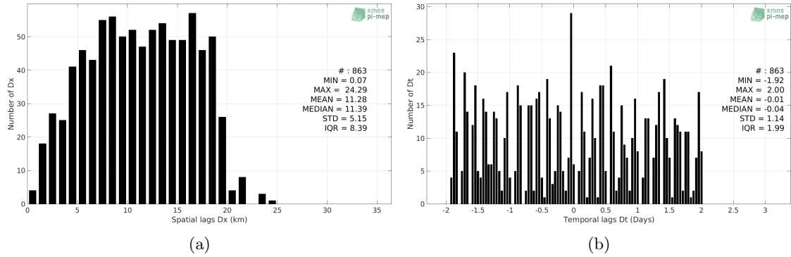
Figure 5: Histograms of the spatial (a) and temporal (b) lags between the location/time of the Marine mammals measurement and the date of the corresponding SMOS SSS L3 v7 - 9 Days (CATDS-CECOS-LOCEAN) SSS pixel.
