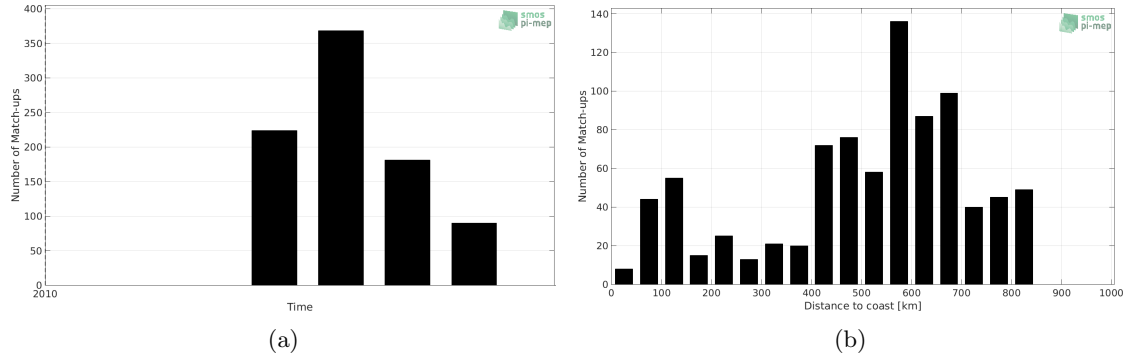
Figure 1: Number of match-ups between Marine mammals and SMOS SSS L3 v7 - 9 Days (CATDS-CECOS-LOCEAN) SSS as a function of time (a) and as function of the distance to coast (b) over the North Atlantic Ocean Pi-MEP region and for the full satellite product period.
