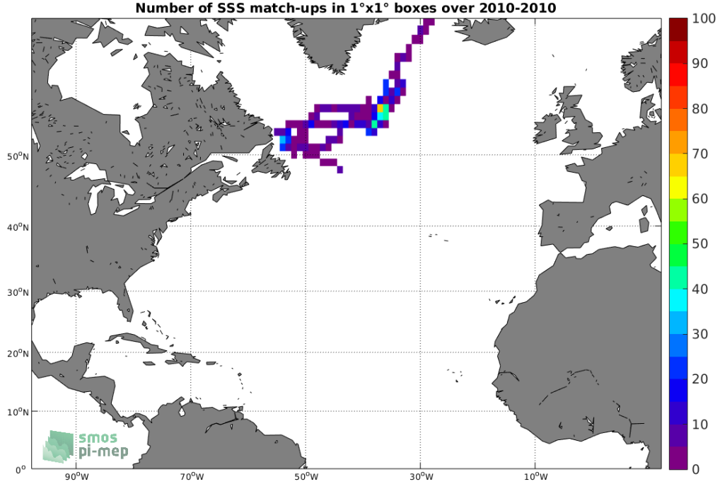
Figure 4: Number of SSS match-ups between Marine mammals SSS and the SMOS SSS L3 v7 - 9 Days (CATDS-CECOS-LOCEAN) SSS product for the North Atlantic Ocean Pi-MEP region over 1^\circ \times 1^\circ boxes and for the full satellite product period.
