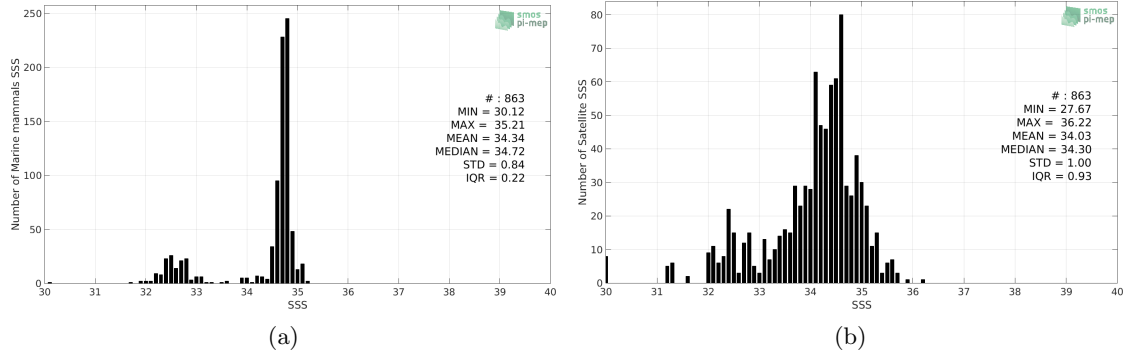
Figure 2: Histograms of SSS from Marine mammals (a) and SMOS SSS L3 v7 - 9 Days (CATDS-CECOS-LOCEAN) (b) considering all match-up pairs per bins of 0.1 over the North Atlantic Ocean Pi-MEP region and for the full satellite product period.
