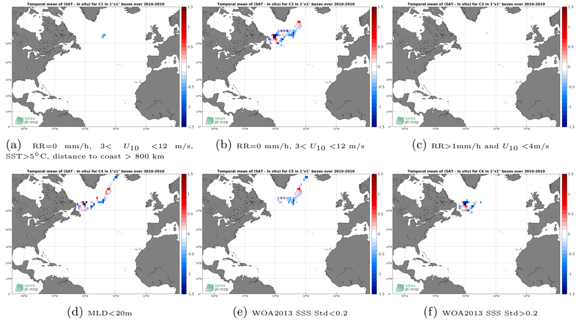
Figure 12: Temporal mean gridded over spatial boxes of size 1^{\circ} \times 1^{\circ} of \Delta\text{SSS} (SMOS SSS L3 v7 - 9 Days (CATDS-CECOS-LOCEAN) - Marine mammals) for 6 different subdatasets corresponding to: RR=0 mm/h, 3 < U_{10} < 12 m/s, SST > 5^{\circ}\text{C} , distance to coast > 800 km (a), RR=0 mm/h, 3 < U_{10} < 12 m/s (b), RR > 1\text{mm/h} and U_{10} < 4\text{m/s} (c), MLD < 20\text{m} (d), WOA2013 SSS Std < 0.2 (e), WOA2013 SSS Std > 0.2 (f).
