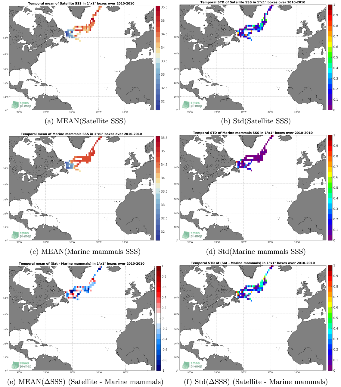
Figure 6: Temporal mean (left) and Std (right) of SSS from SMOS SSS L3 v7 - 9 Days (CATDS-CECOS-LOCEAN) (top), Marine mammals (middle), and of \Delta SSS (Satellite - Marine mammals). Only match-up pairs are used to generate these maps.
