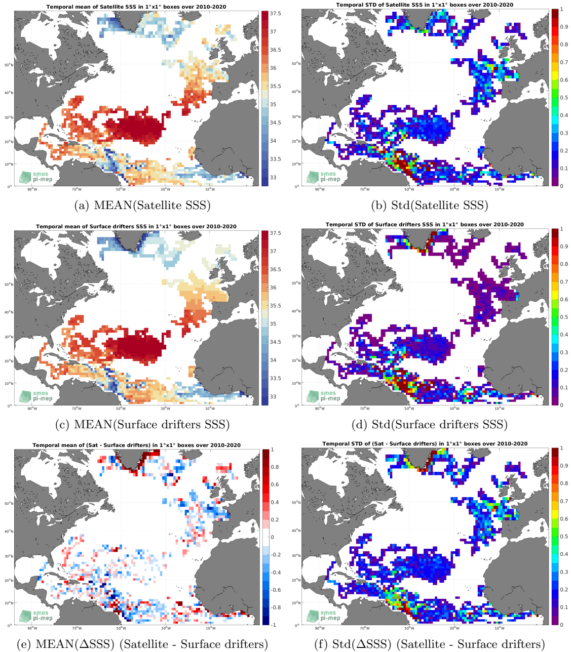
Figure 5: Temporal mean (left) and Std (right) of SSS from SMOS SSS L3 v7 - 9 Days (CATDS-CECOS-LOCEAN) (top), Surface drifters (middle), and of \Delta SSS (Satellite - Surface drifters). Only match-up pairs are used to generate these maps.
