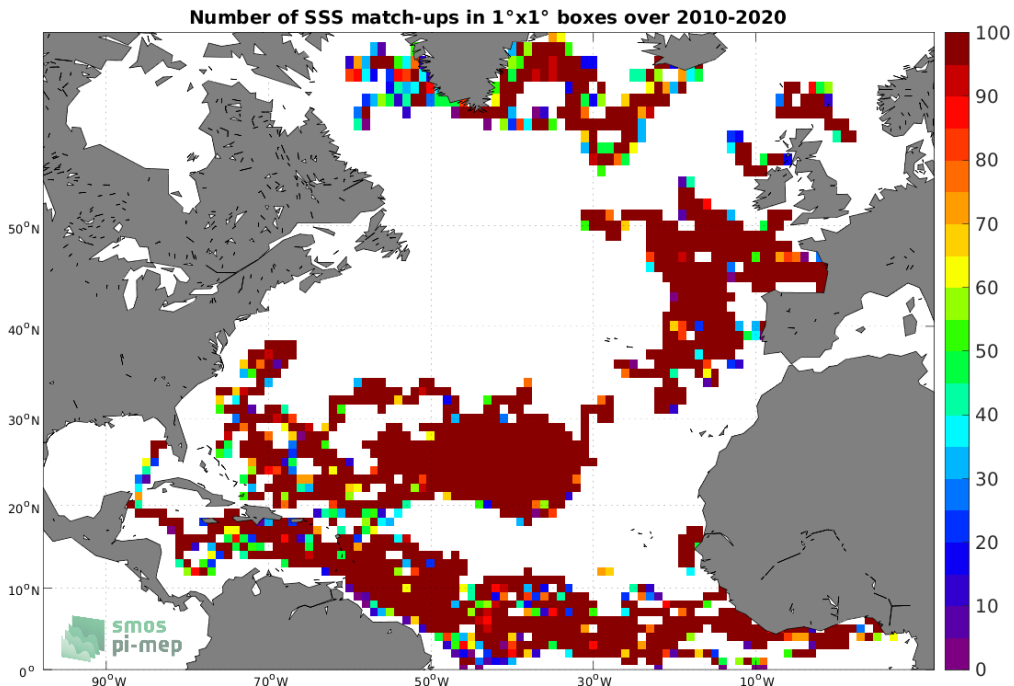
Figure 3: Number of SSS match-ups between Surface drifters SSS and the SMOS SSS L3 v7 - 9 Days (CATDS-CECOS-LOCEAN) SSS product for the North Atlantic Ocean Pi-MEP region over 1^\circ \times 1^\circ boxes and for the full satellite product period.
