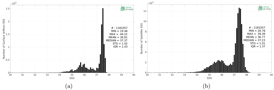
Figure 2: Histograms of SSS from Surface drifters (a) and SMOS SSS L3 v7 - 9 Days (CATDS-CECOS-LOCEAN) (b) considering all match-up pairs per bins of 0.1 over the North Atlantic Ocean Pi-MEP region and for the full satellite product period.
