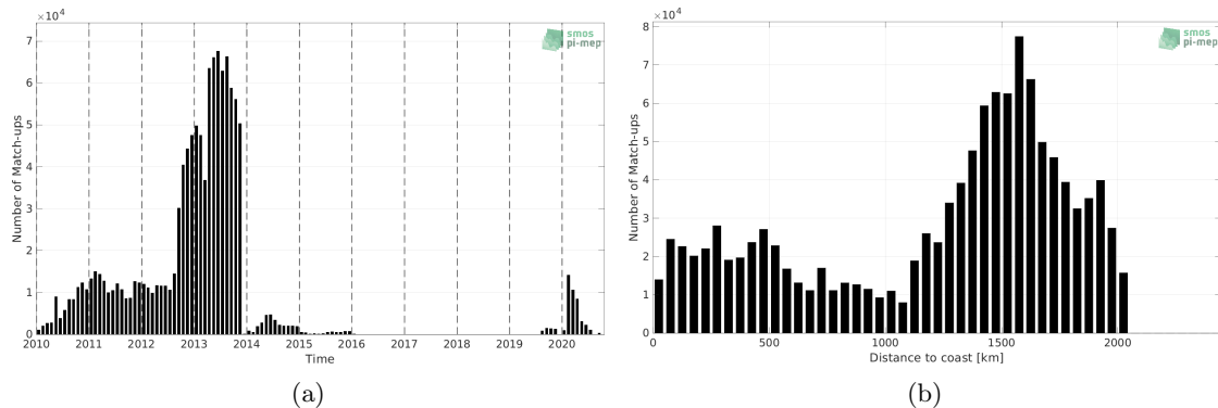
Figure 1: Number of match-ups between Surface drifters and SMOS SSS L3 v7 - 9 Days (CATDS-CECOS-LOCEAN) SSS as a function of time (a) and as function of the distance to coast (b) over the North Atlantic Ocean Pi-MEP region and for the full satellite product period.
