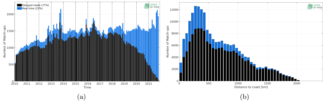
Figure 1: Number of match-ups between Argo and SMOS SSS L3 v7 - 9 Days (CATDS-CECOS-LOCEAN) SSS as a function of time (a) and as function of the distance to coast (b) over the North Atlantic Ocean Pi-MEP region and for the full satellite product period.
