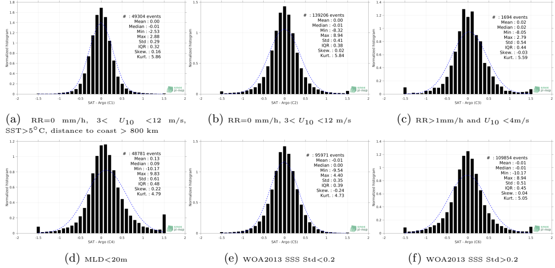
Figure 13: Normalized histogram of \Delta SSS (SMOS SSS L3 v7 - 9 Days (CATDS-CECOS-LOCEAN) - Argo) for 6 different subdatasets corresponding to: RR=0 mm/h, 3 < U_{10} < 12 m/s, SST>5°C, distance to coast > 800 km (a), RR=0 mm/h, 3 < U_{10} < 12 m/s (b), RR>1mm/h and U_{10} < 4 m/s (c), MLD<20m (d), WOA2013 SSS Std<0.2 (e), WOA2013 SSS Std>0.2 (f).
