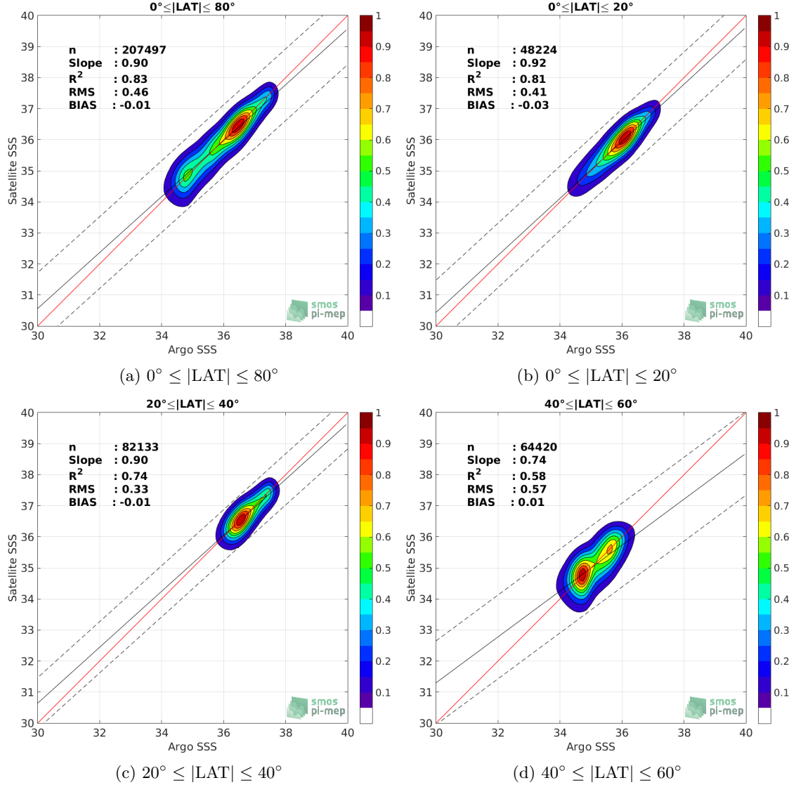
Figure 9: Contour maps of the concentration of SMOS SSS L3 v7 - 9 Days (CATDS-CECOS-LOCEAN) SSS (y-axis) versus Argo SSS (x-axis) at match-up pairs for different latitude bands. For each plot, the red line shows x=y . The black thin and dashed lines indicate a linear fit through the data cloud and the \pm 95\% confidence levels, respectively. The number match-up pairs n , the slope and R^2 coefficient of the linear fit, the root mean square (RMS) and the mean bias between satellite and in situ data are indicated for each latitude band in each plots.
