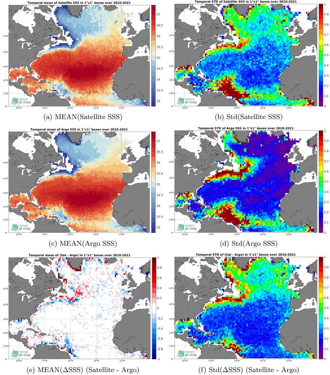
Figure 6: Temporal mean (left) and Std (right) of SSS from SMOS SSS L3 v7 - 9 Days (CATDS-CECOS-LOCEAN) (top), Argo (middle), and of \Delta SSS (Satellite - Argo). Only match-up pairs are used to generate these maps.
