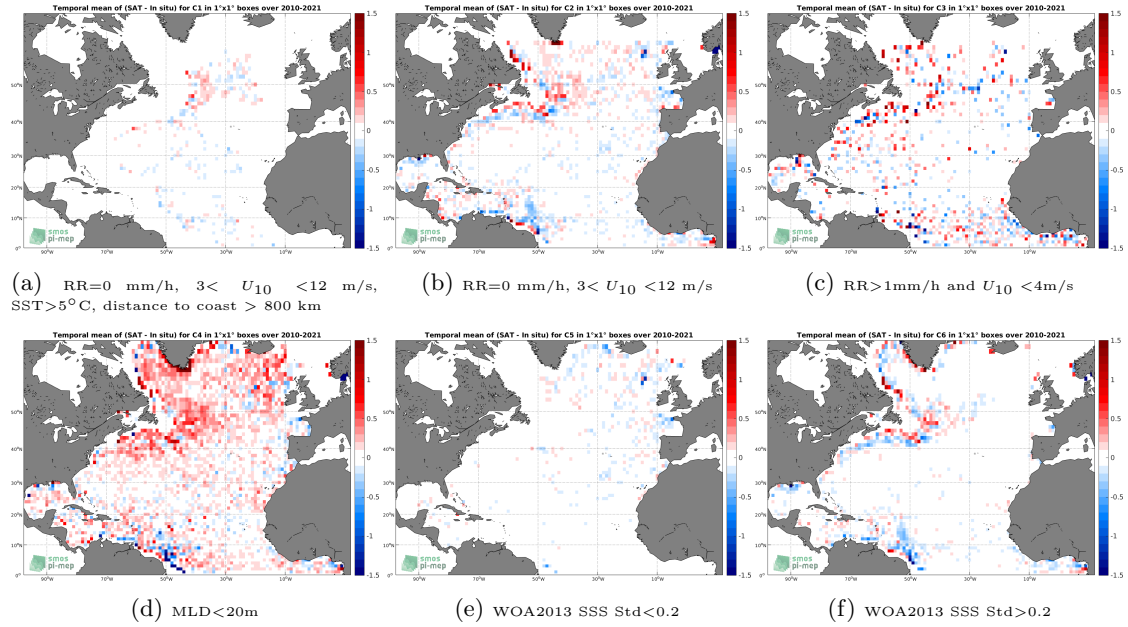
Figure 12: Temporal mean gridded over spatial boxes of size 1^\circ \times 1^\circ of \Delta SSS (SMOS SSS L3 v7 - 9 Days (CATDS-CECOS-LOCEAN) - Argo) for 6 different subdatasets corresponding to:RR=0 mm/h, 3 < U_{10} < 12 m/s, SST >5^\circ C, distance to coast > 800 km (a), RR=0 mm/h, 3 < U_{10} < 12 m/s (b), RR >1 mm/h and U_{10} < 4 m/s (c),MLD <20 m (d),WOA2013 SSS Std <0.2 (e),WOA2013 SSS Std >0.2 (f).
