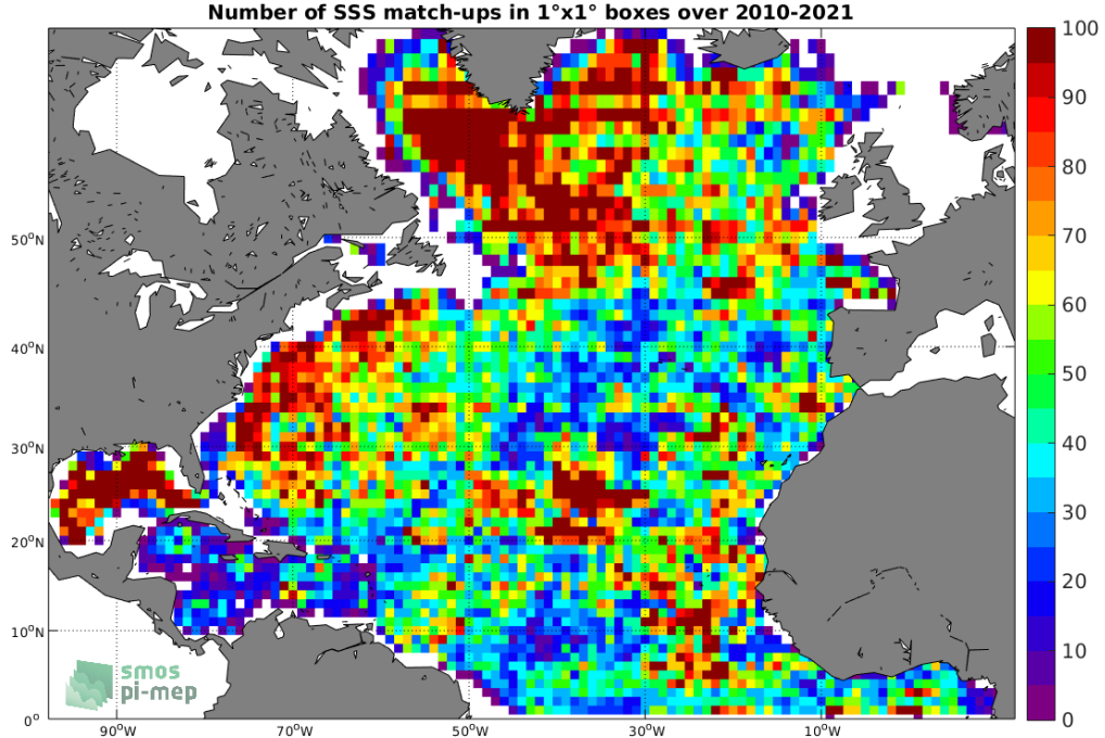
Figure 4: Number of SSS match-ups between Argo SSS and the SMOS SSS L3 v7 - 9 Days (CATDS-CECOS-LOCEAN) SSS product for the North Atlantic Ocean Pi-MEP region over 1^\circ \times 1^\circ boxes and for the full satellite product period.
