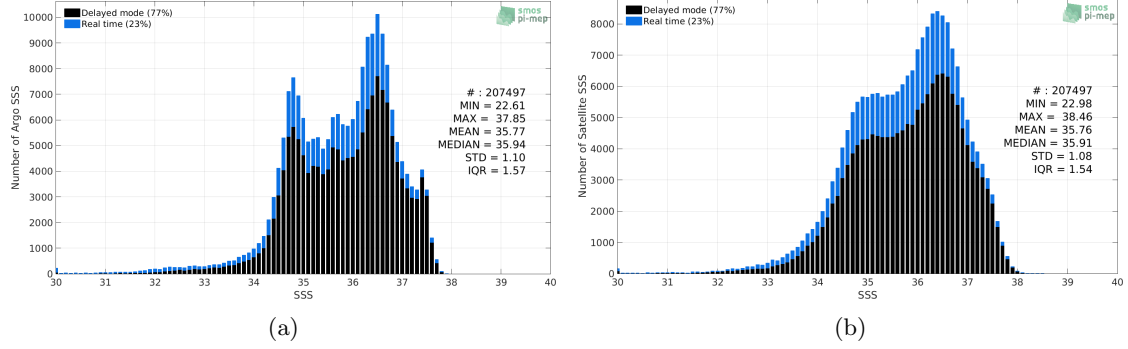
Figure 2: Histograms of SSS from Argo (a) and SMOS SSS L3 v7 - 9 Days (CATDS-CECOS-LOCEAN) (b) considering all match-up pairs per bins of 0.1 over the North Atlantic Ocean Pi-MEP region and for the full satellite product period.
