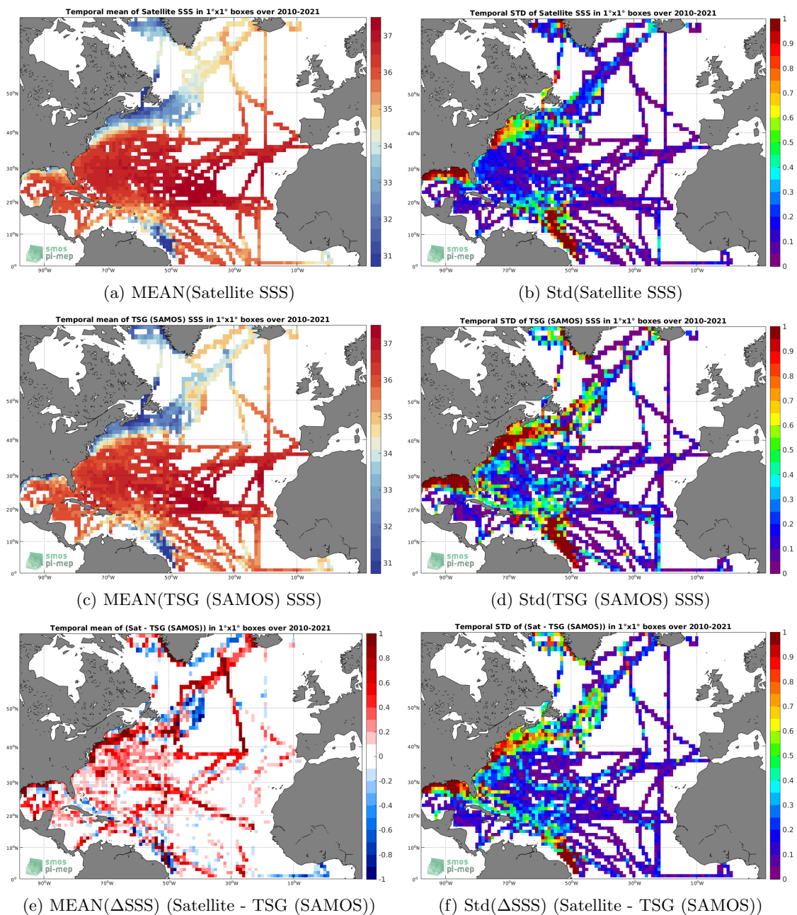
Figure 6: Temporal mean (left) and Std (right) of SSS from SMOS SSS L3 v7 - 18 Days (CATDS-CECOS-LOCEAN) (top), TSG (SAMOS) (middle), and of \Delta SSS (Satellite - TSG (SAMOS)). Only match-up pairs are used to generate these maps.
