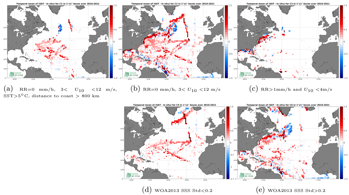
Figure 12: Temporal mean gridded over spatial boxes of size 1^\circ \times 1^\circ of \Delta\text{SSS} (SMOS SSS L3 v7 - 18 Days (CATDS-CECOS-LOCEAN) - TSG (SAMOS)) for 5 different subdatasets corresponding to:RR=0 mm/h, 3 < U_{10} < 12 m/s, SST > 5^\circ\text{C} , distance to coast > 800 km (a), RR=0 mm/h, 3 < U_{10} < 12 m/s (b), RR > 1 mm/h and U_{10} < 4 m/s (c), WOA2013 SSS Std < 0.2 (d), WOA2013 SSS Std > 0.2 (e).
