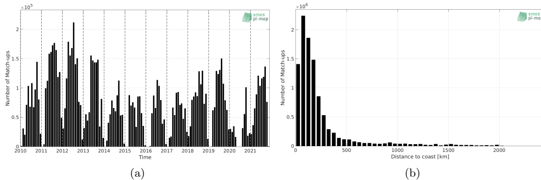
Figure 1: Number of match-ups between TSG (SAMOS) and SMOS SSS L3 v7 - 18 Days (CATDS-CECOS-LOCEAN) SSS as a function of time (a) and as function of the distance to coast (b) over the North Atlantic Ocean Pi-MEP region and for the full satellite product period.
