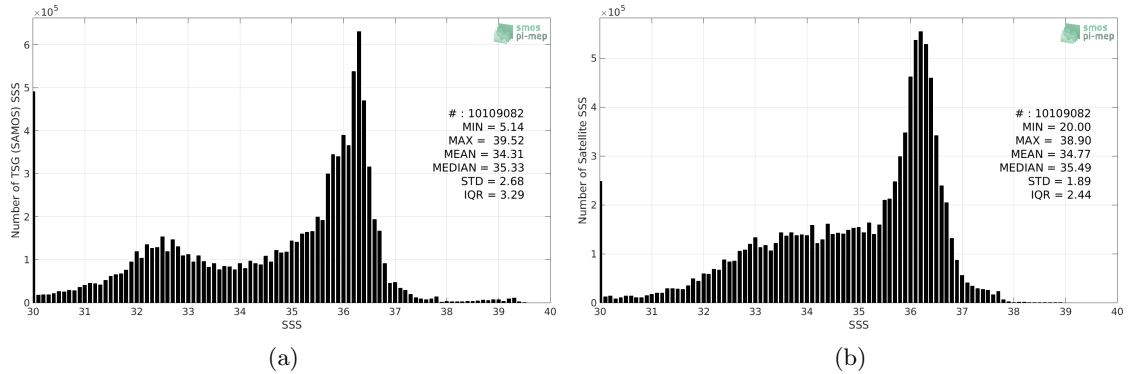
Figure 2: Histograms of SSS from TSG (SAMOS) (a) and SMOS SSS L3 v7 - 18 Days (CATDS-CECOS-LOCEAN) (b) considering all match-up pairs per bins of 0.1 over the North Atlantic Ocean Pi-MEP region and for the full satellite product period.
