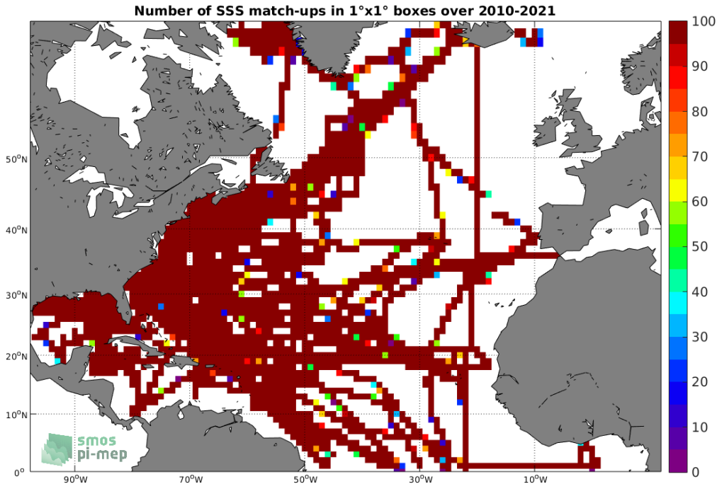
Figure 4: Number of SSS match-ups between TSG (SAMOS) SSS and the SMOS SSS L3 v7 - 18 Days (CATDS-CECOS-LOCEAN) SSS product for the North Atlantic Ocean Pi-MEP region over 1^{\circ} \times 1^{\circ} boxes and for the full satellite product period.
