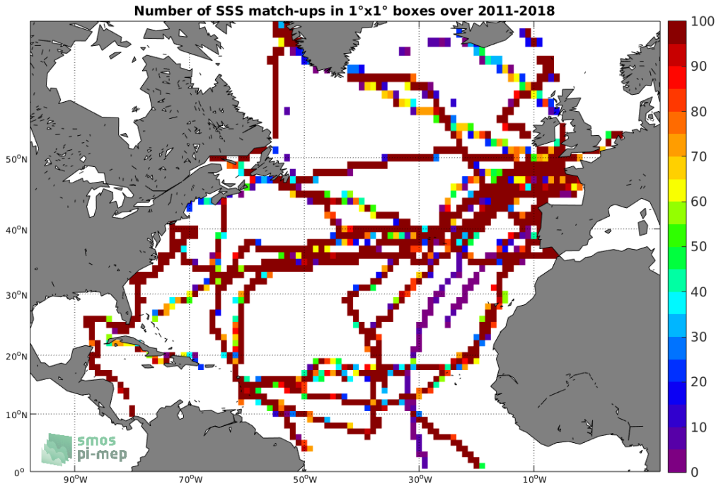
Figure 4: Number of SSS match-ups between TSG (GOSUD-Sailing-ship) SSS and the SMOS SSS L3 v7 - 18 Days (CATDS-CECOS-LOCEAN) SSS product for the North Atlantic Ocean Pi-MEP region over 1^\circ \times 1^\circ boxes and for the full satellite product period.
