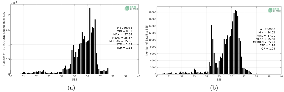
Figure 2: Histograms of SSS from TSG (GOSUD-Sailing-ship) (a) and SMOS SSS L3 v7 - 18 Days (CATDS-CECOS-LOCEAN) (b) considering all match-up pairs per bins of 0.1 over the North Atlantic Ocean Pi-MEP region and for the full satellite product period.
