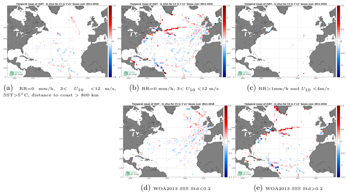
Figure 12: Temporal mean gridded over spatial boxes of size 1^\circ \times 1^\circ of \Delta\text{SSS} (SMOS SSS L3 v7 - 18 Days (CATDS-CECOS-LOCEAN) - TSG (GOSUD-Sailing-ship)) for 5 different subdatasets corresponding to:RR=0 mm/h, 3 < U_{10} < 12 m/s, SST>5°C, distance to coast > 800 km (a), RR=0 mm/h, 3 < U_{10} < 12 m/s (b), RR>1mm/h and U_{10} < 4 m/s (c), WOA2013 SSS Std<0.2 (d), WOA2013 SSS Std>0.2 (e).
