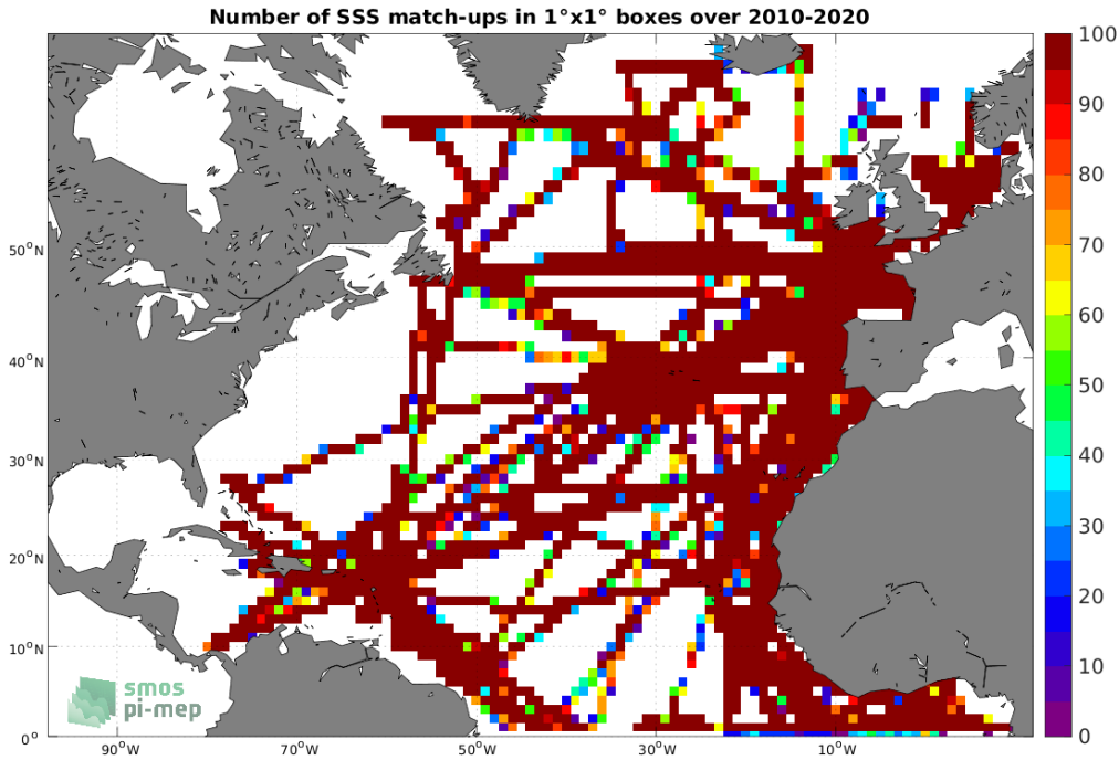
Figure 4: Number of SSS match-ups between TSG (GOSUD-Research-vessel) SSS and the SMOS SSS L3 v7 - 18 Days (CATDS-CECOS-LOCEAN) SSS product for the North Atlantic Ocean Pi-MEP region over 1^\circ \times 1^\circ boxes and for the full satellite product period.
