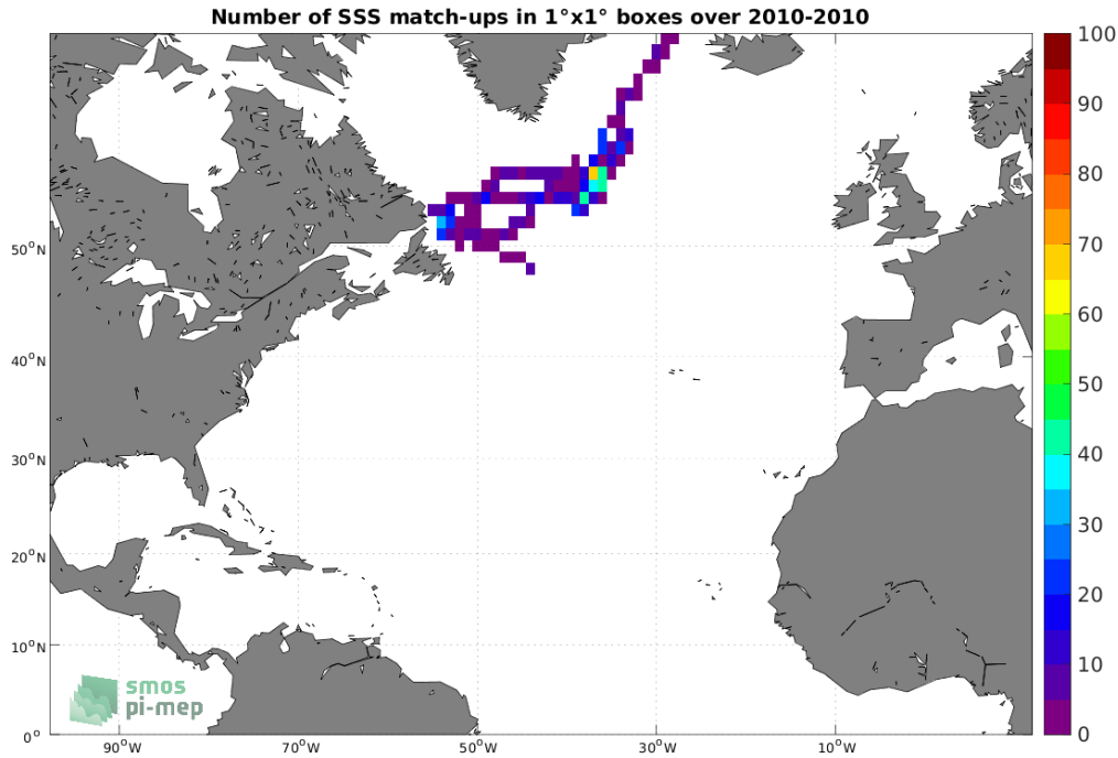
Figure 4: Number of SSS match-ups between Marine mammals SSS and the SMOS SSS L3 v7 - 18 Days (CATDS-CECOS-LOCEAN) SSS product for the North Atlantic Ocean Pi-MEP region over 1^\circ \times 1^\circ boxes and for the full satellite product period.
